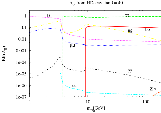
Fig. 3. Branching ratios for the CP-odd scalar A_0 of the MSSM.
