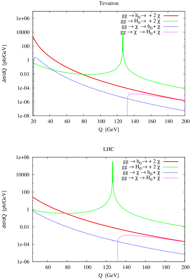
Fig. 13. gg \rightarrow 2 -scalar reactions mediated by trilinear vertices.
