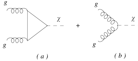
Fig. 8. The two contributions to the gg \rightarrow \chi production channel.
