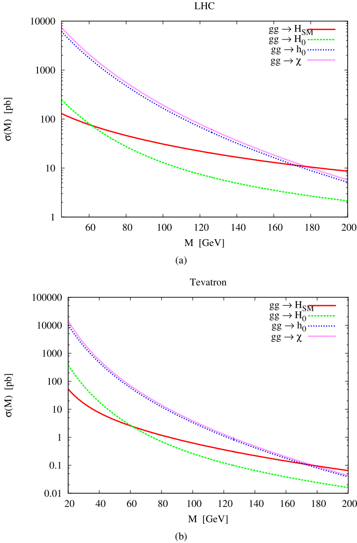
Fig. 9. Cross section for the production of the two Higgs h_0 and H_0 and the axi-Higgs via gluon–gluon fusion at LO at the LHC (a) and at the Tevatron (b).
