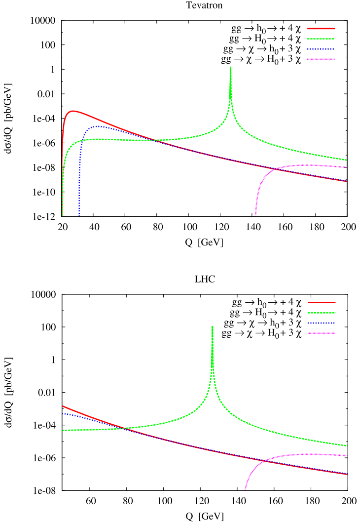
Fig. 14. Production of 3 and 4 scalars from gluon–gluon fusion mediated by trilinear and quadrilinear vertices.
