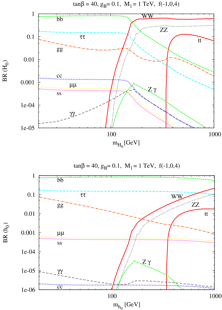
Fig. 5. Study of the branching ratios of the CP-even sector.
