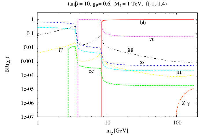
Fig. 2. Study of the branching ratios of the axi-Higgs. We analyze the dependence on the free parameters g_B , \tan\beta .
