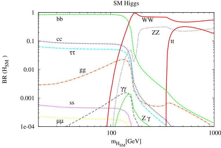
Fig. 6. Study of the branching ratios of the SM-Higgs.
