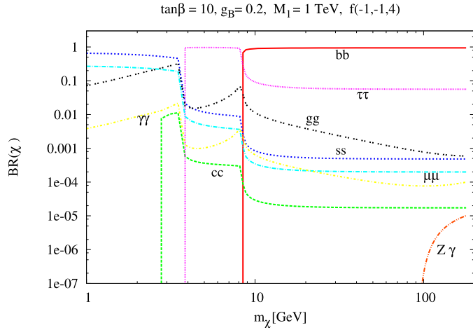
Fig. 2. Study of the branching ratios of the axi-Higgs. We analyze the dependence on the free parameters g_B , \tan\beta .
