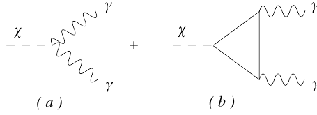
Fig. 1. Massless plus massive contributions to the \chi \rightarrow \gamma\gamma process.
