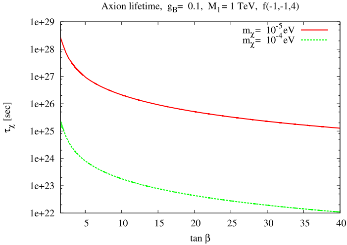
Fig. 15. Lifetime for an ultralight axion as a function of \tan \beta .
