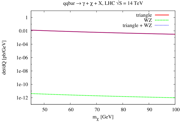
Fig. 11. Invariant mass distribution for the associated production of an axion plus one photon at the LHC.
