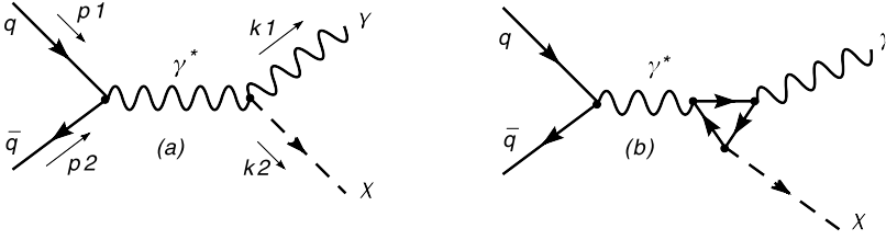
Fig. 10. Production channel for a single axion plus a photon.
