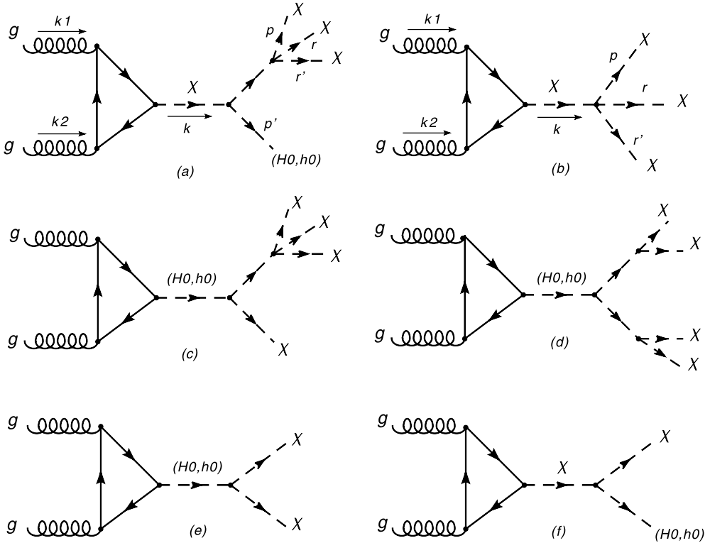
Fig. 12. Channels for multi axion production from gluon–gluon fusion.
