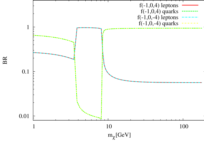
Fig. 4. Study of the leptonic and the quarks branching ratios of the axi-Higgs. We analyze the dependence on the function f(q_{QL}^B, q_{uR}^B, \Delta q^B) .
