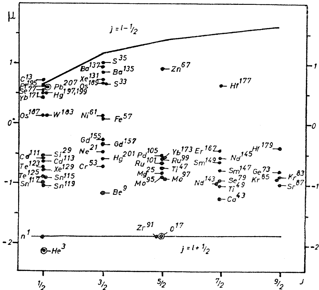
Fig. 11. Experimental magnetic moments (data from El-59b, Bo-62b, Gr-68b) and Schmidt limits for odd-neutron nuclei, as functions of the total angular momentum j . The dotted lines in the upper figure are the Schmidt lines based on the magnetic moments for
