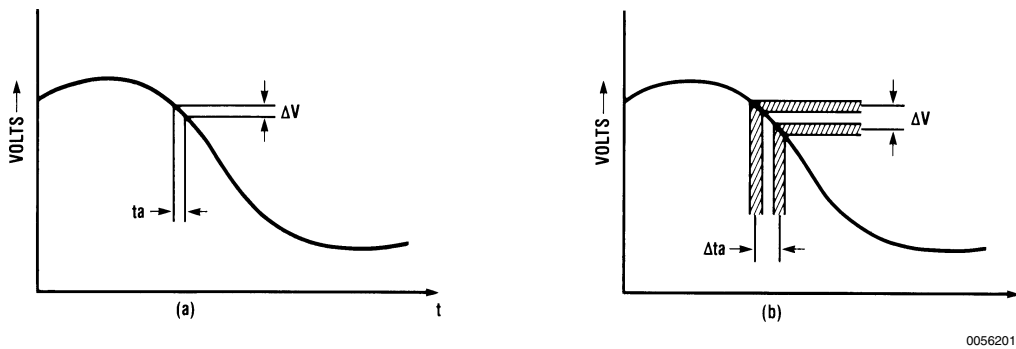
FIGURE 11. Quantization error.
