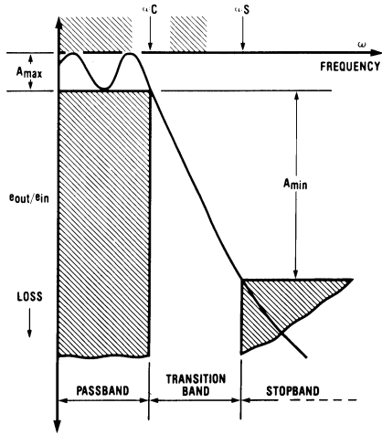
FIGURE 17. Common Low Pass Filter Response
