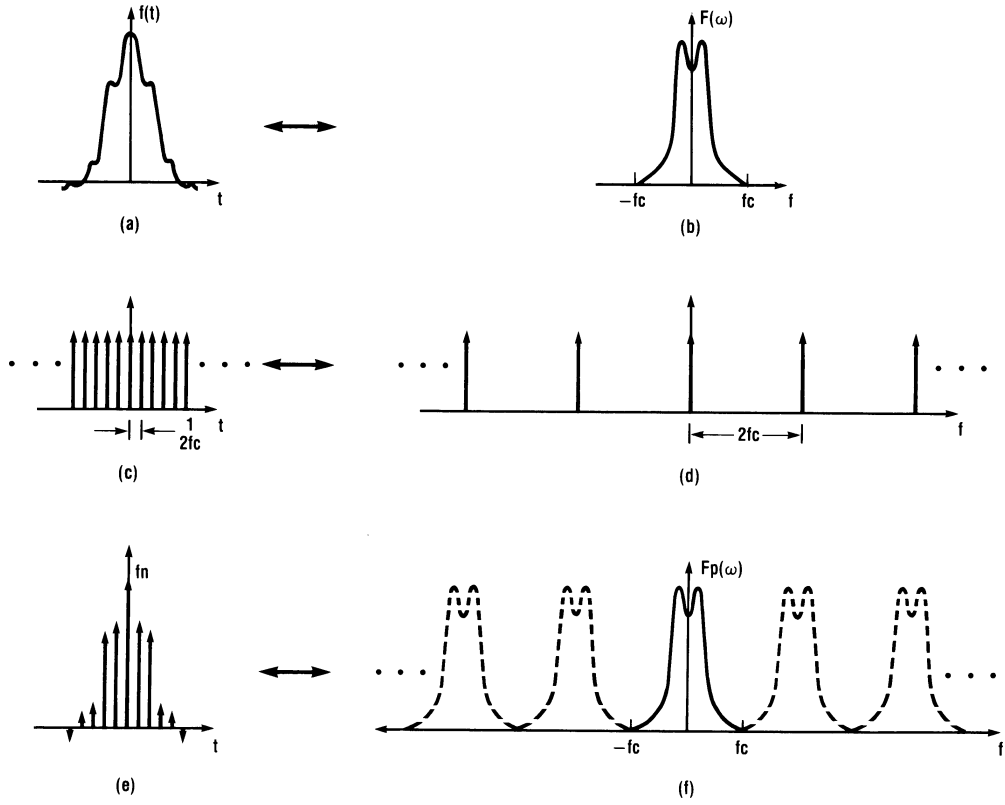
FIGURE 3. Fourier transform of a sampled signal.
