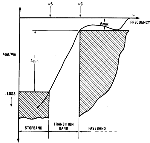
FIGURE 18. Common High Pass Filter Response
