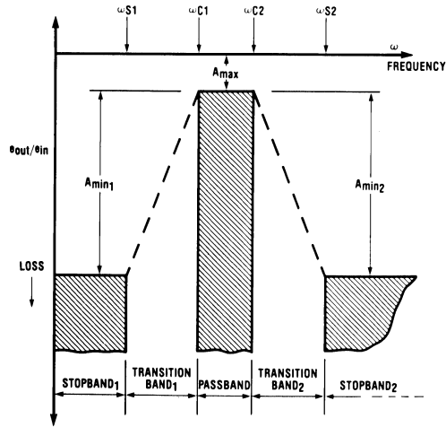
FIGURE 19. Common Band-pass Filter Response
