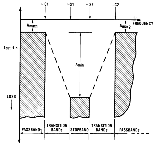
FIGURE 20. Common Band-Reject Filter Response
