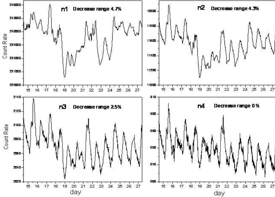
Figure 7. Scaler mode count rates, before weather effect corrections, from January 15 to 27, 2005, showing the detection of a Forbush decrease by ARGO-YBJ. The n1,...,n4 labels refer to the counting rates with at least 1,2,3 or 4 hits respectively (see text).
