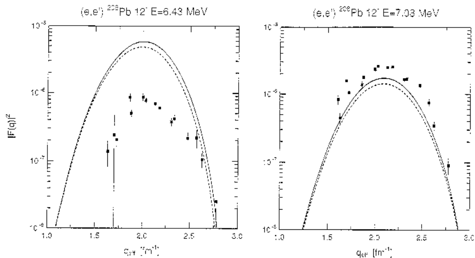
Fig. 5. Form factor squared for the 12^- states calculated with the two-state model. The full lines are calculated including MEC. The data are from ref. 12)
