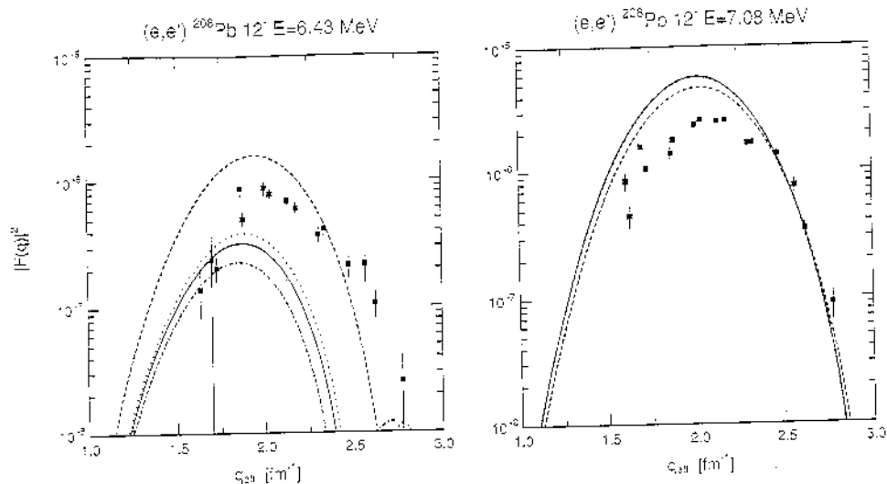
Fig. 7. Form factor squared of the two 12^- states. The full, dashed-dotted and dashed lines have been obtained with force 1, 2 and 3, respectively. The dotted lines have been calculated with the zero-range interaction of eq. (3) using g_0=0.26 and g'_0=0.83 .
