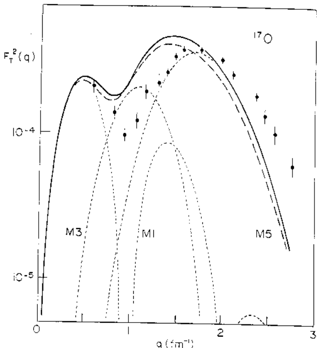
FIG. 28. The ^{17}\text{O} data of Hynes et al. (1979) compared to prediction of the extreme single-particle model calculated using a harmonic-oscillator wave function (solid curve). The long-dashed curve is calculated using a Woods-Saxon radial wave function.
