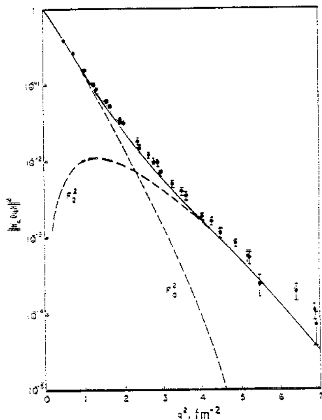
Fig. 10. Squared charge form factor of {}^7\text{Li} fitted by Hartree-Fock wave functions (full line). The monopole and quadrupole form factors are shown separately by the dashed lines. The experimental data are from Suelzle et al. (368) and the theoretical curves from Bouten et al. (63)
