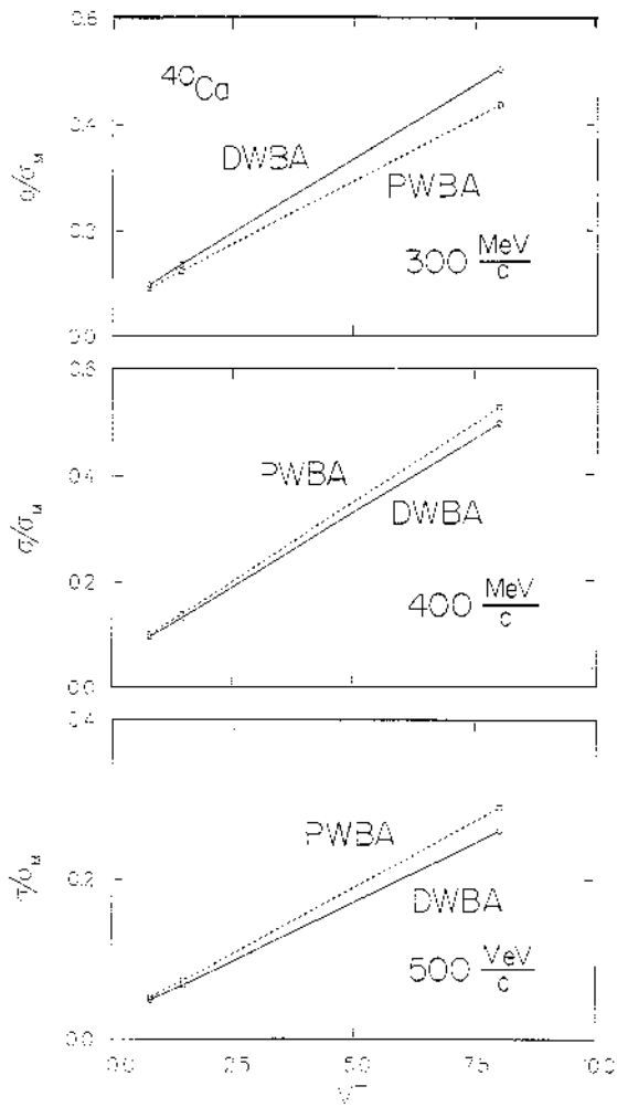
Fig. 2. Rosenbluth plots for the reaction ^{40}\text{Ca}(e, e')^{40}\text{Ca} . Also in this case the DWBA points are not perfectly aligned.
