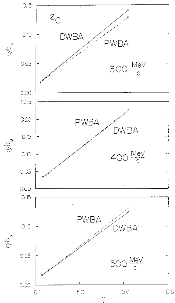
Fig. 1. Rosenbluth plots for the reaction ^{12}\text{C}(e, e')^{12}\text{C} . Note that the DWBA points are not perfectly aligned.
