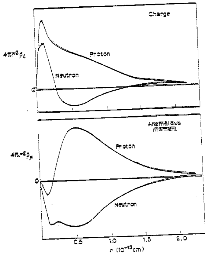
Fig. 15.22. Form factors for the nucleons
