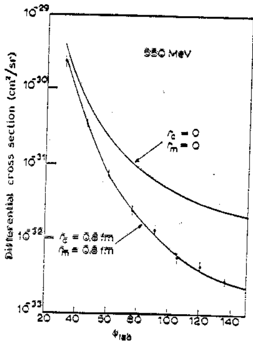
Electron scattering cross-section. The upper curve is for a point nucleus
