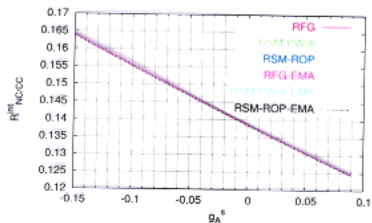
Upper panel: NC over CC ratio of differential cross sections versus the outgoing nucleon kinetic energy, for g_A^s = 0, -0.10 and using the RFG, RSM-PWIA and RSM-ROP models, as indicated in the legenda. Lower panel: NC over CC ratio of integrated cross sections versus g_A^s for the RFG, RSM-PWIA and RSM-ROP models, as indicated. Curves including Coulomb Distortion effects within the effective momentum approximation (EMA) are also shown.
