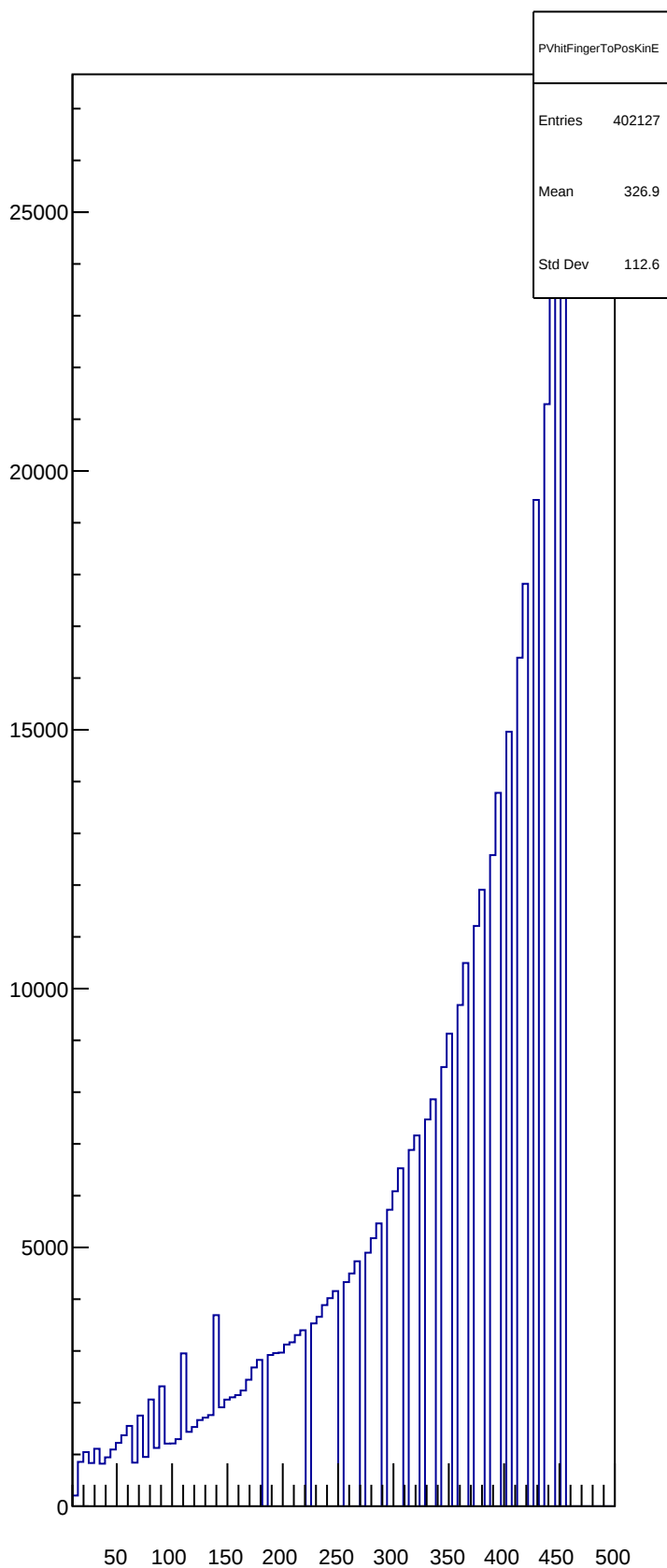
PVhitFingerToPosKinE
