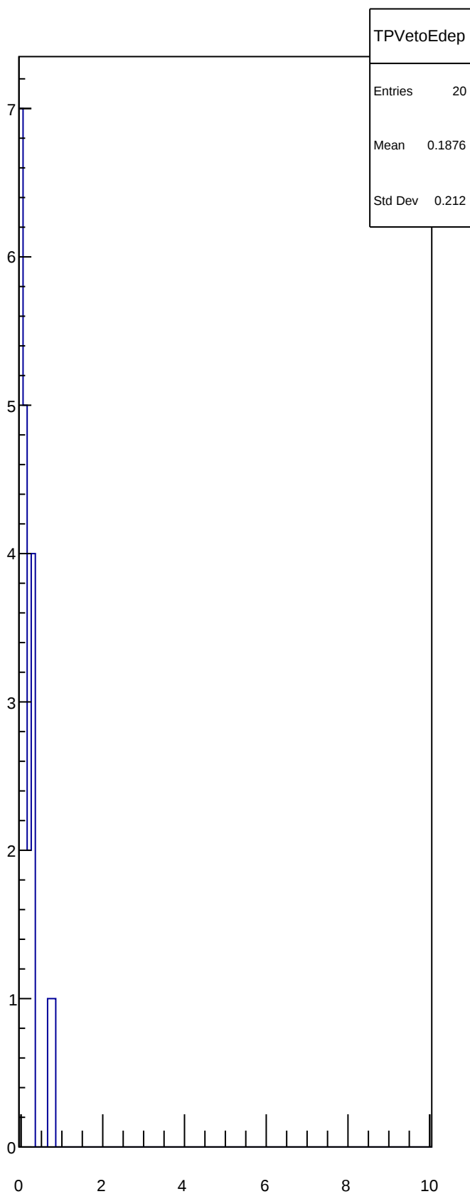
TPVetoEdep
