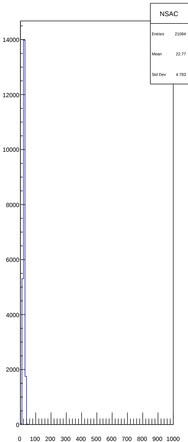
NSAC
