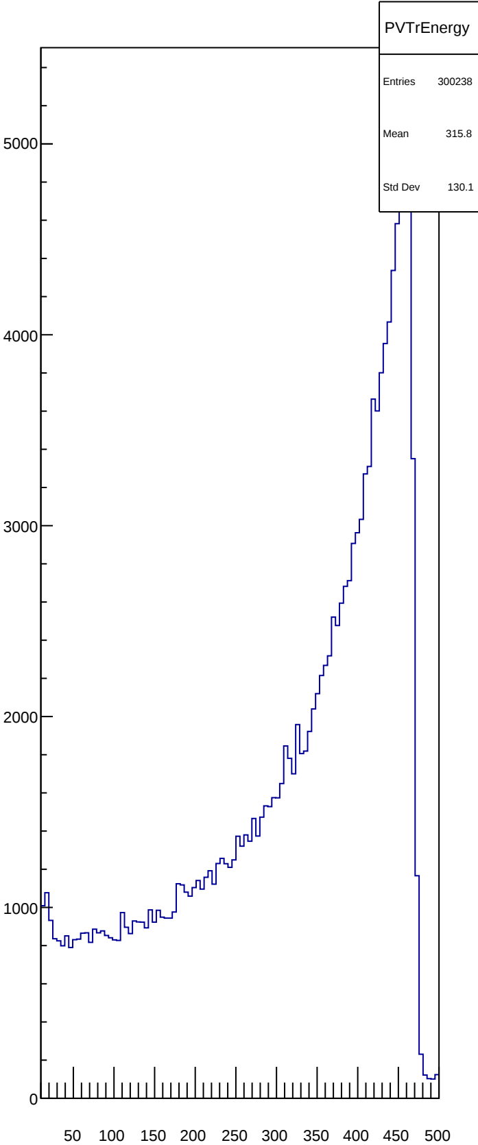
PVTrEnergy
