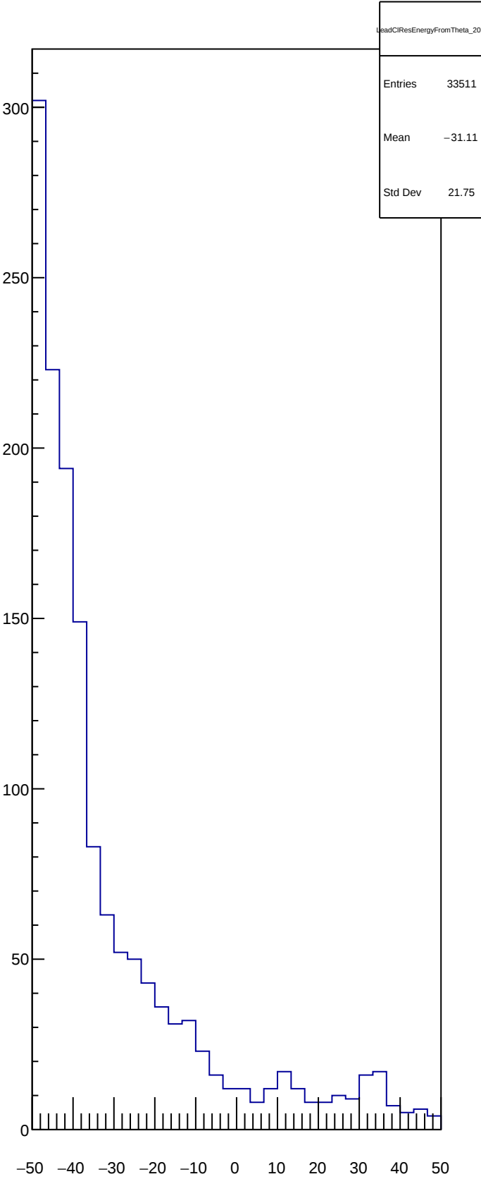
LeadCIResEnergyFromTheta_20
