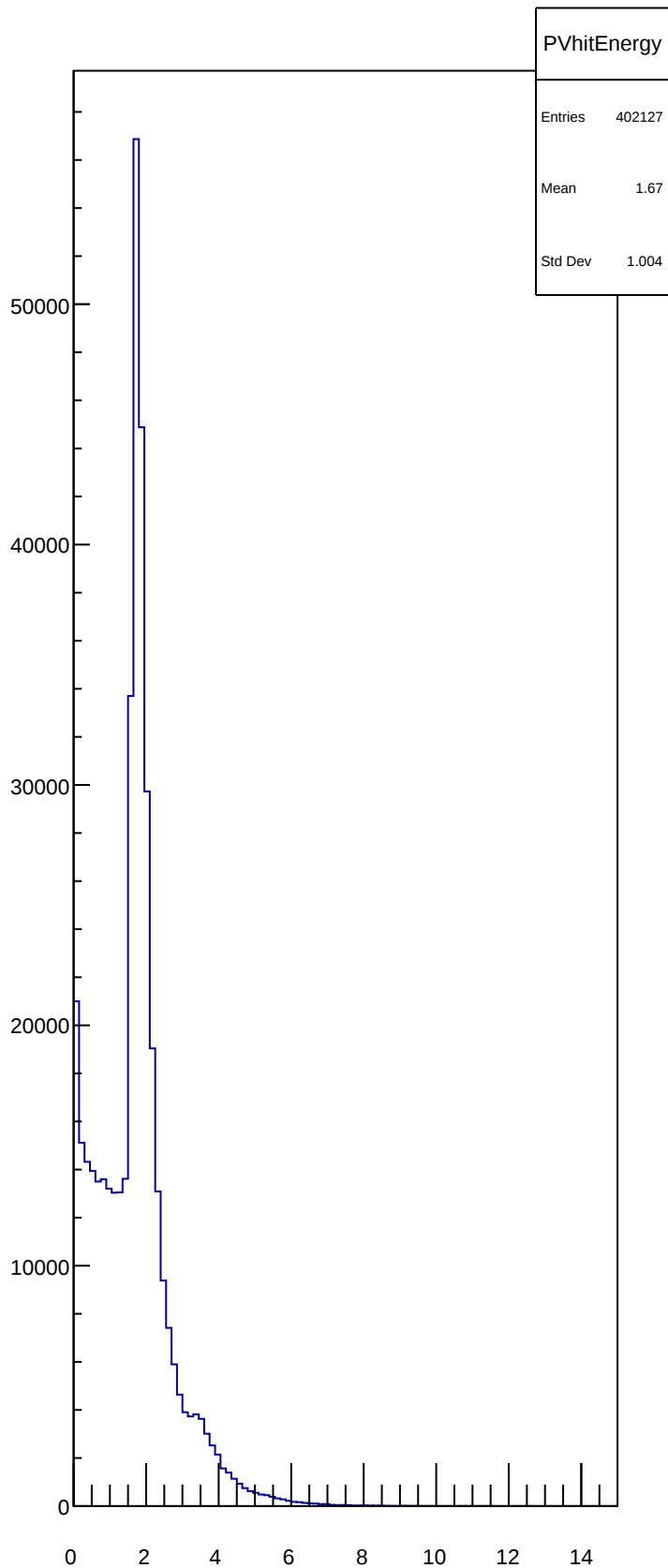
PVhitEnergy
