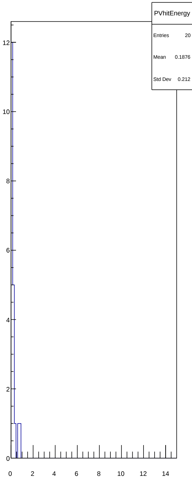
PVhitEnergy
