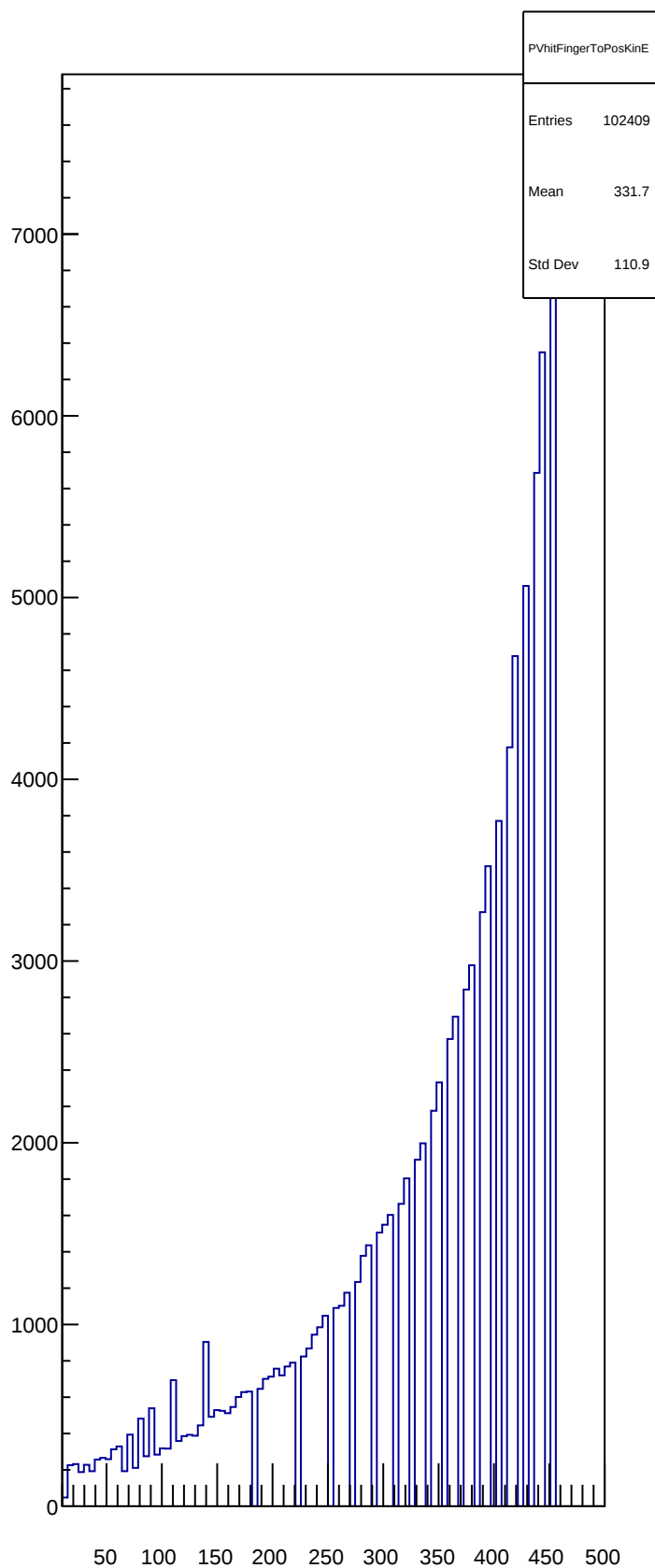
PVhitFingerToPosKinE
