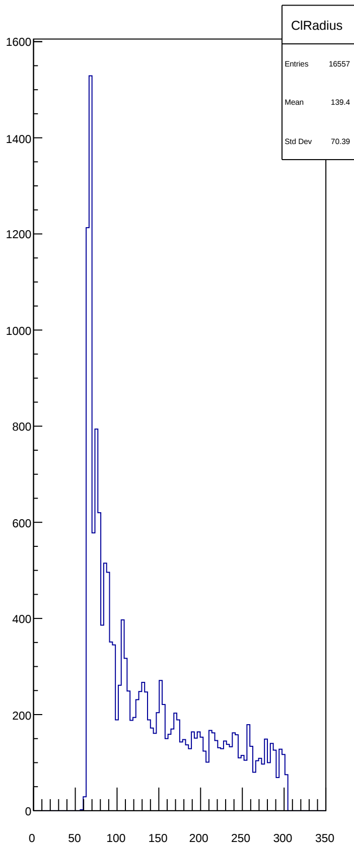
CIRadius
