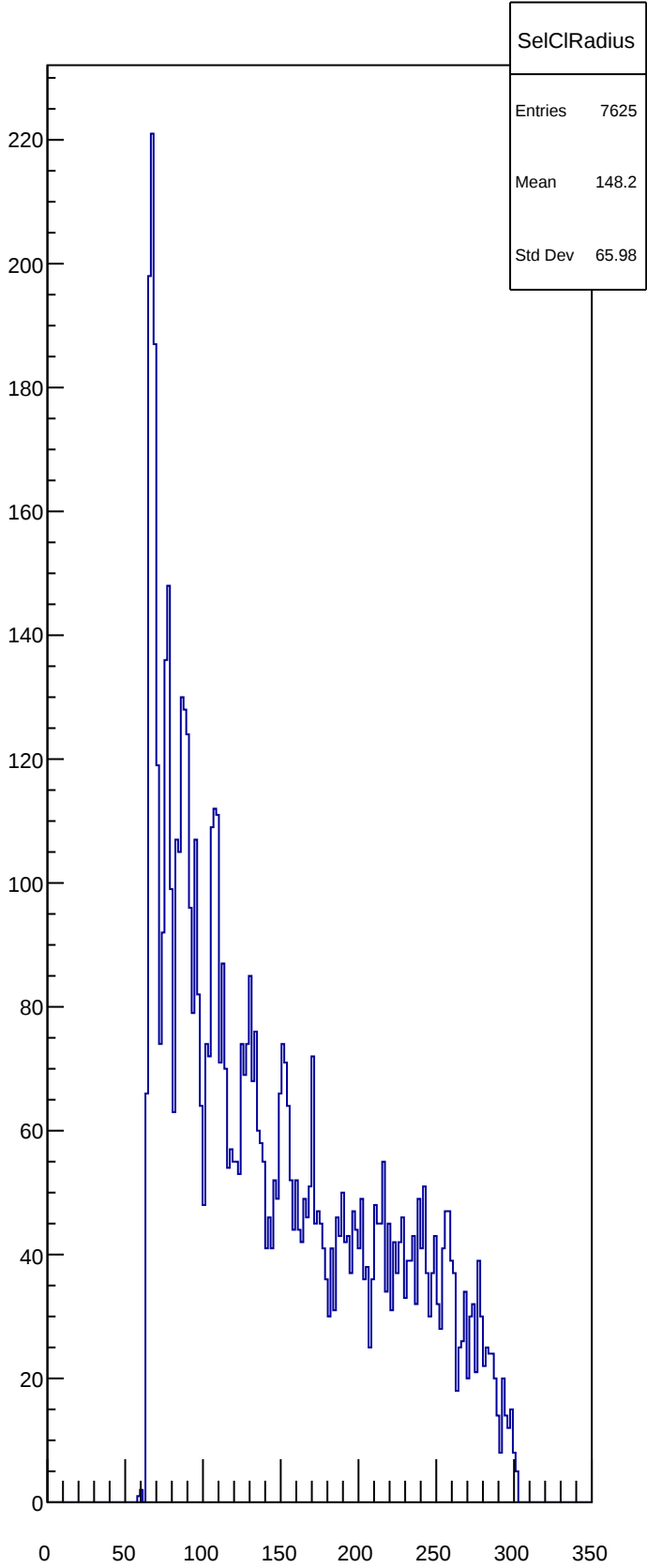
SelCIRadius
