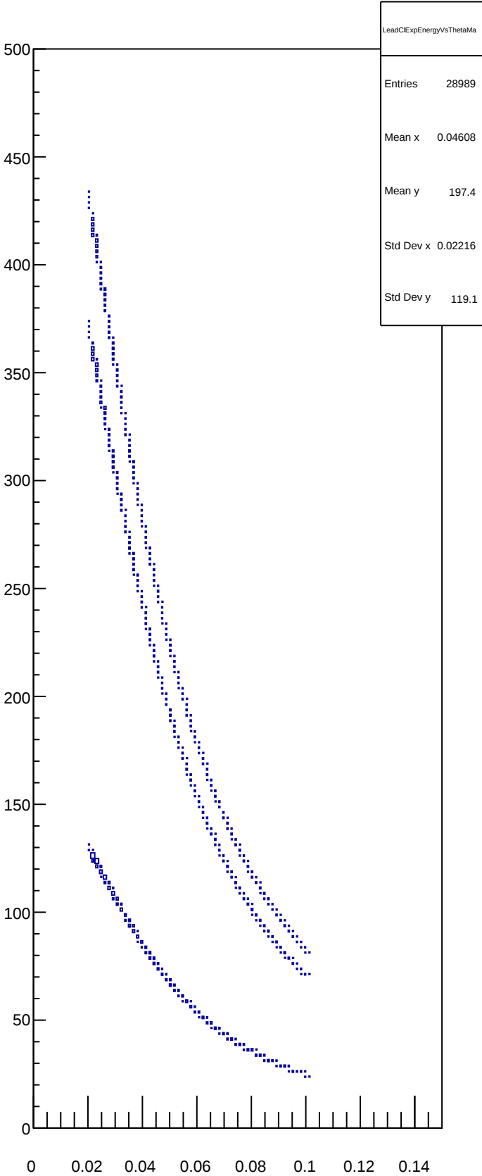
LeadCIExpEnergyVsThetaMa
