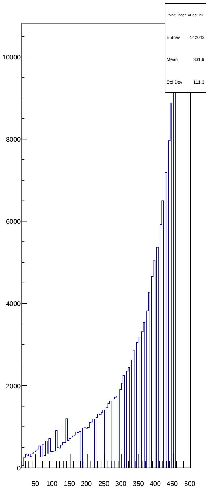
PVhitFingerToPosKinE
