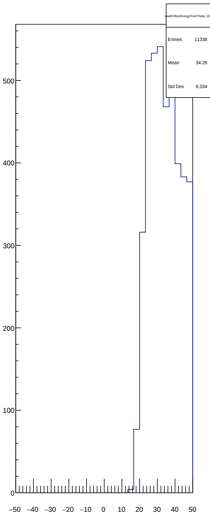
LeadCIResEnergyFromTheta_10
