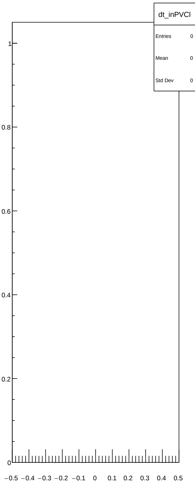
dt_inPVCI
