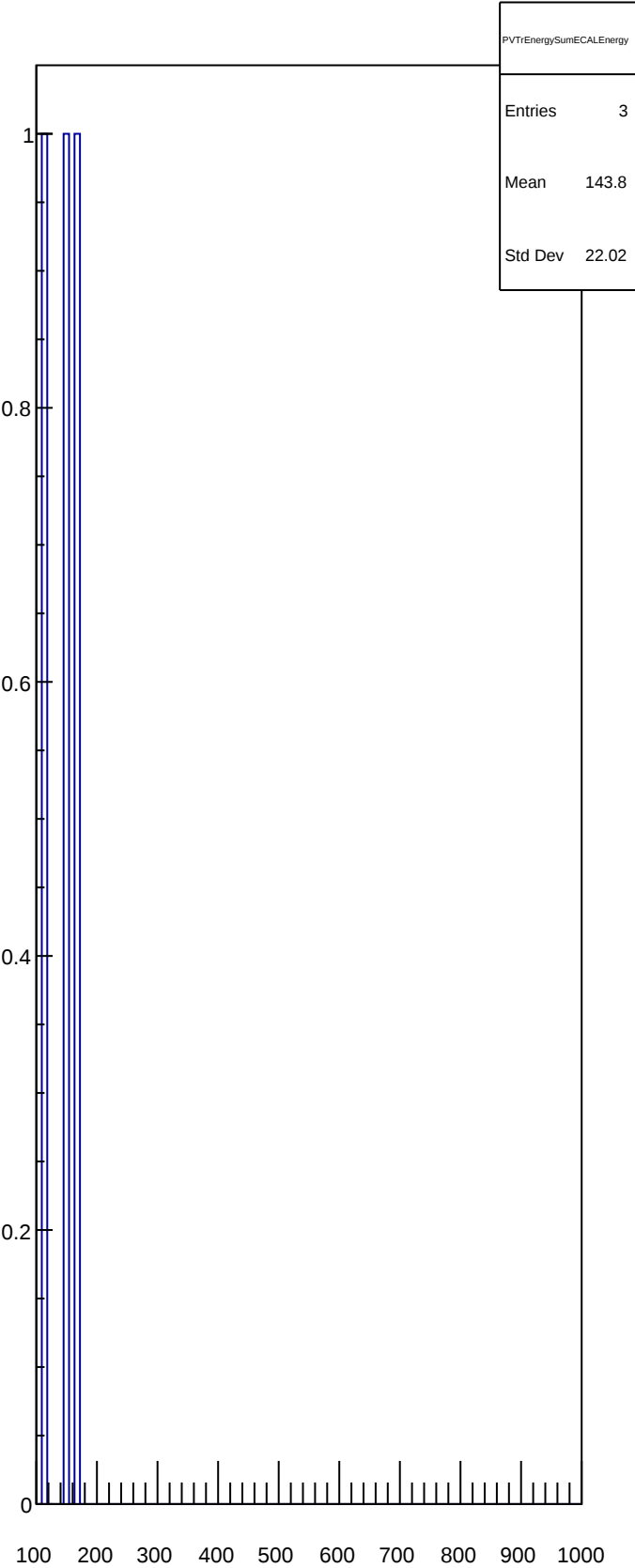
PVTrEnergySumECALEnergy
