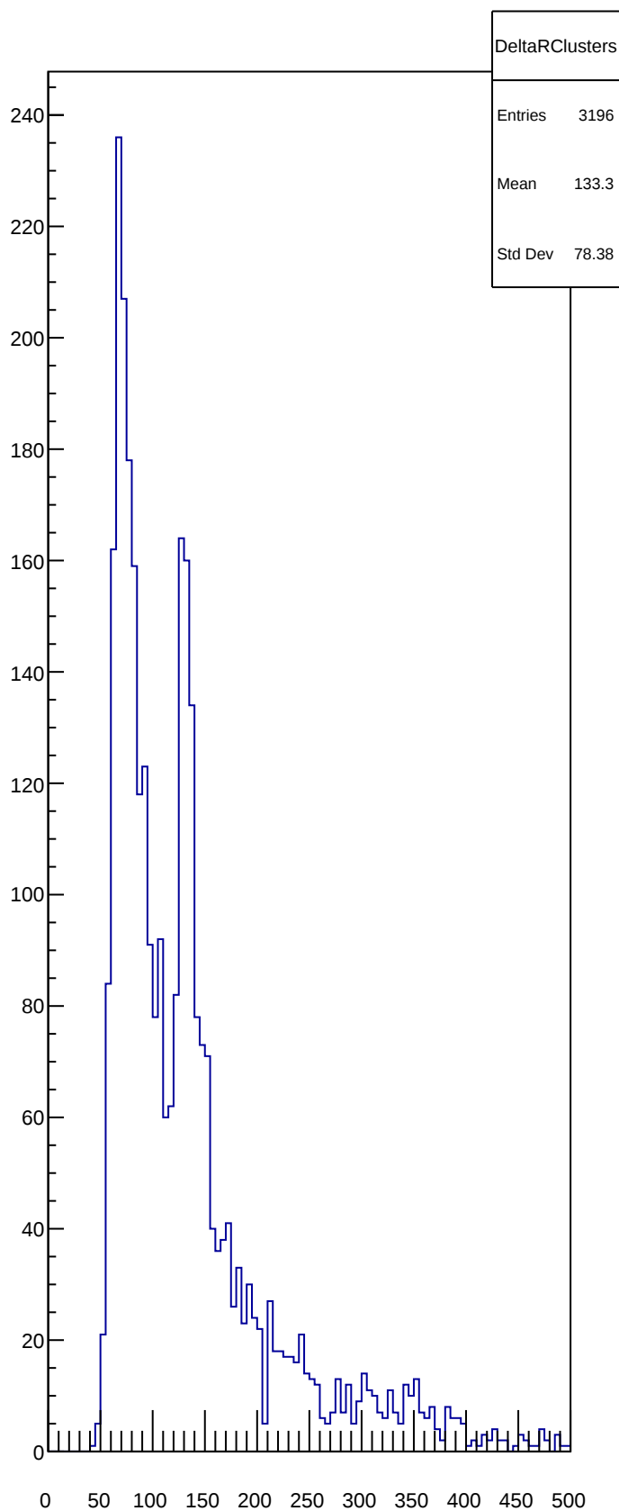
DeltaRClusters
