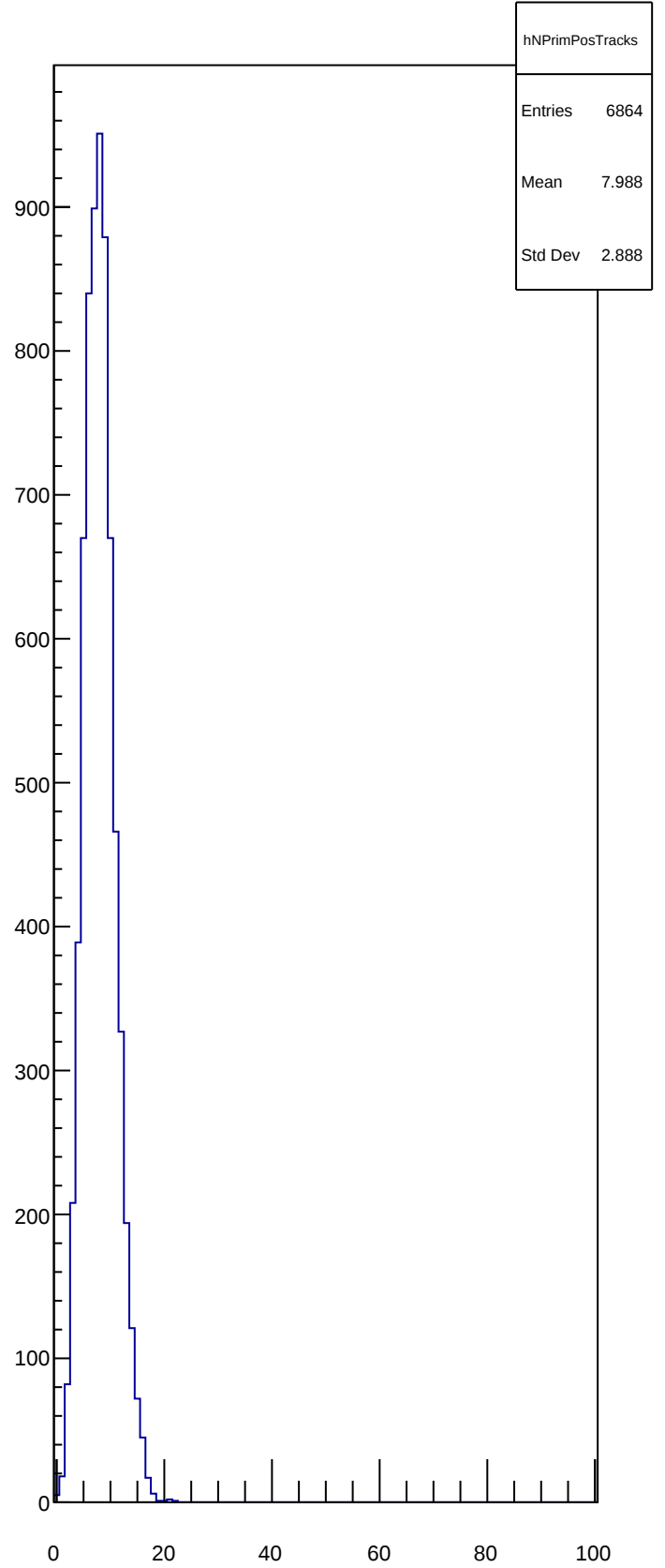
hNPrimPosTracks
