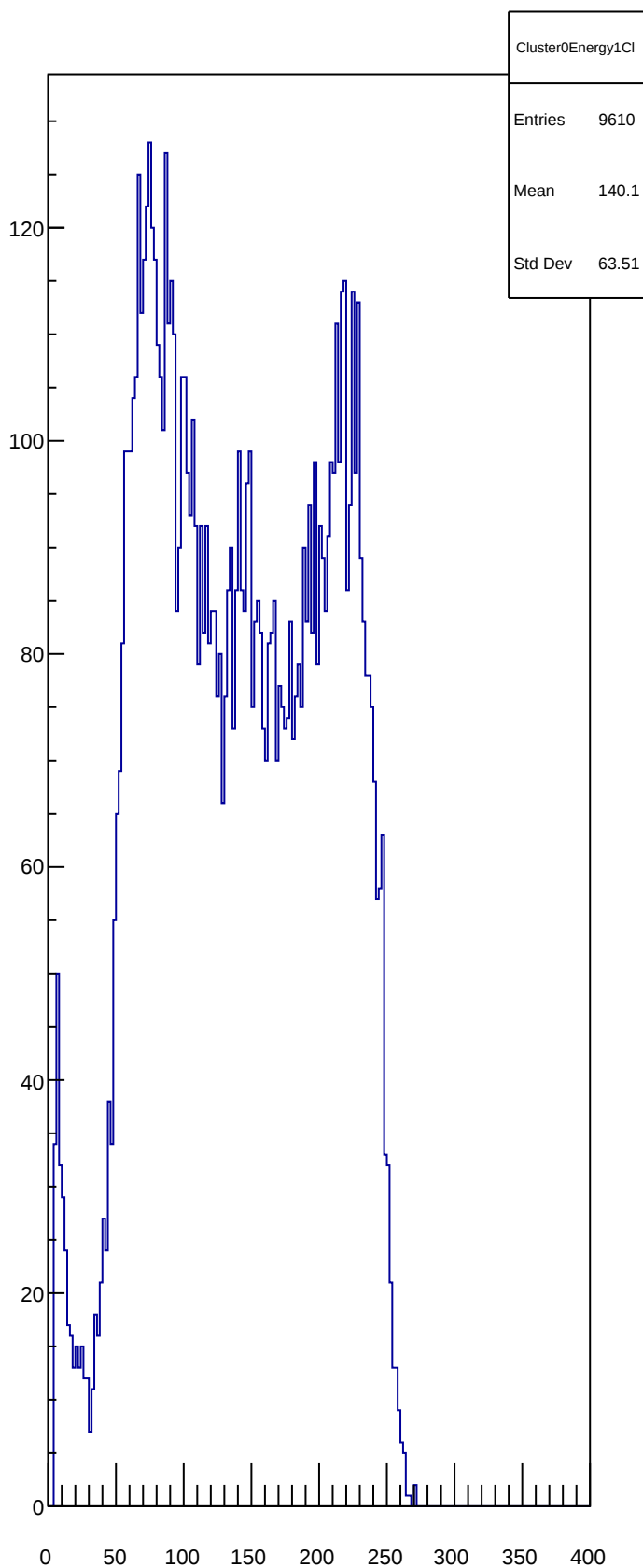
Cluster0Energy1Cl
