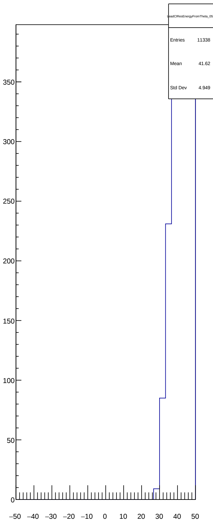
LeadCIResEnergyFromTheta_05
