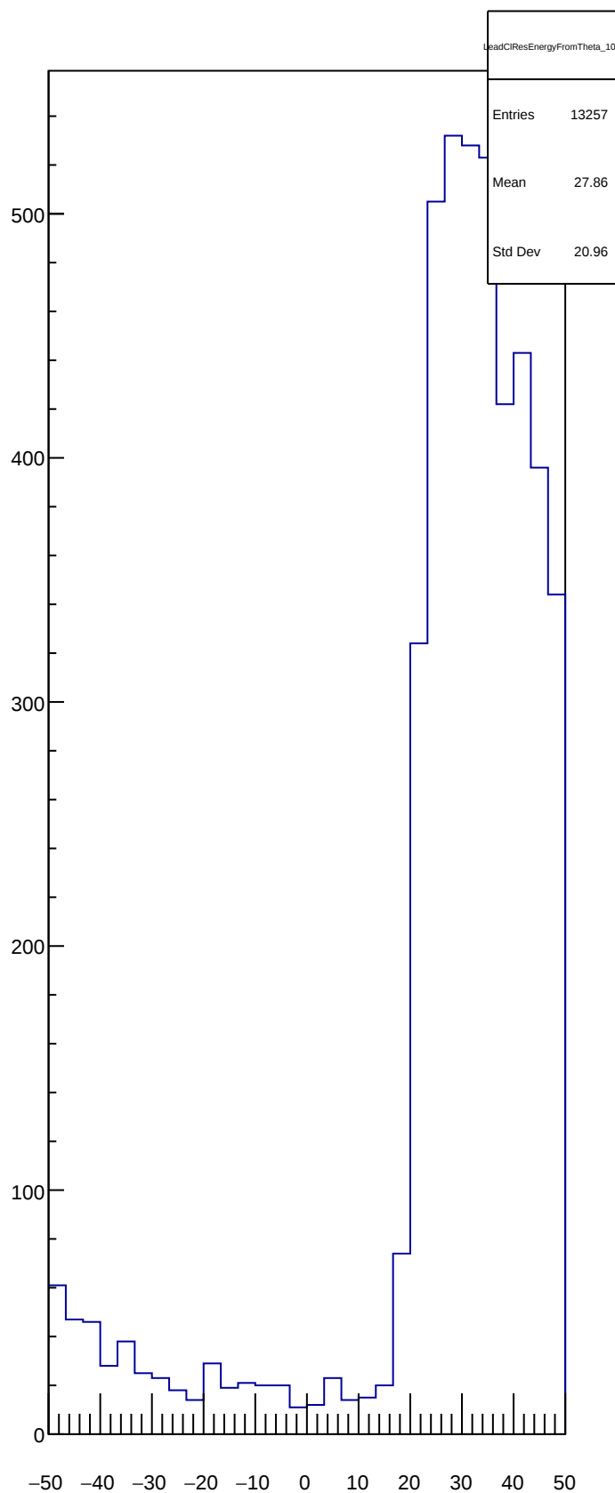
LeadCIResEnergyFromTheta_10
