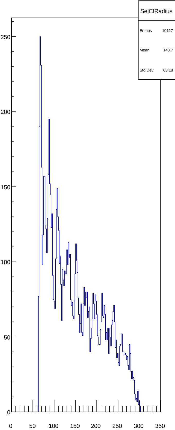
SelCIRadius
