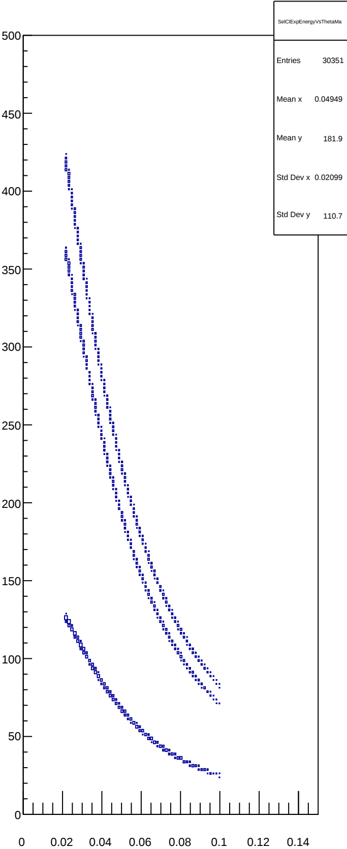
SelClExpEnergyVsThetaMa
