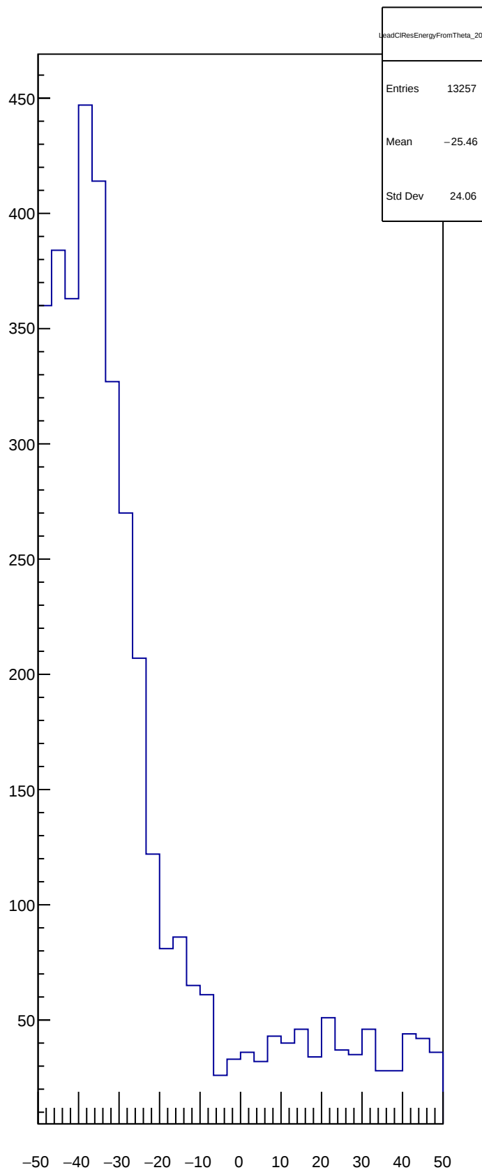
LeadCIResEnergyFromTheta_20
