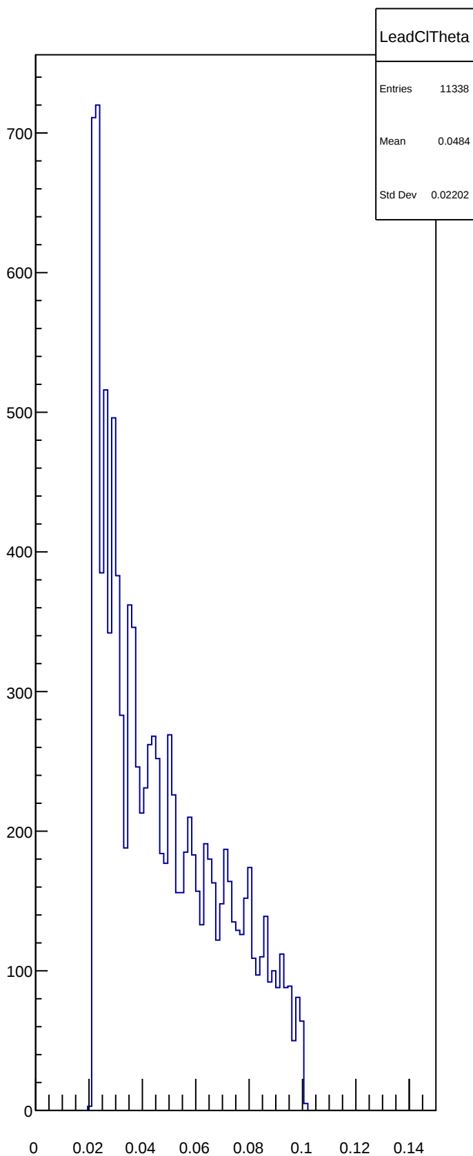
LeadCITheta
