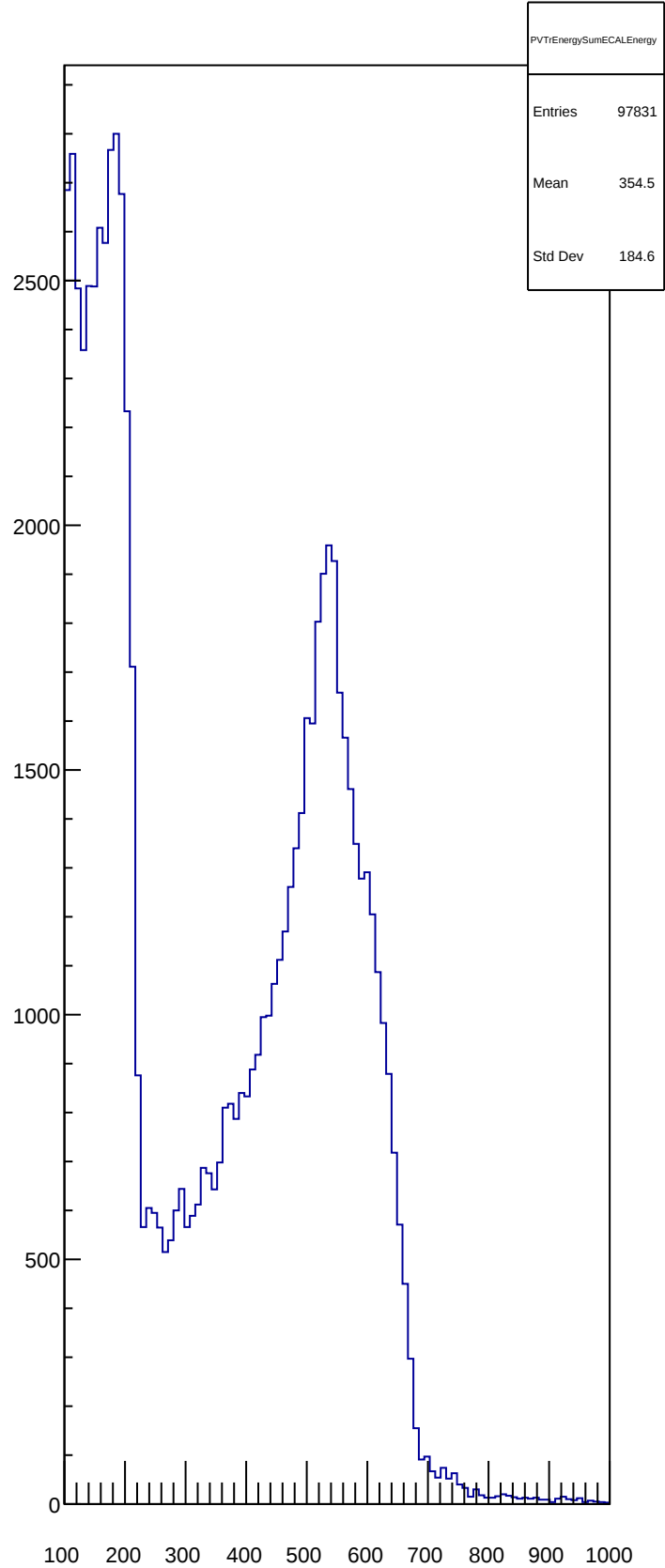
PVTrEnergySumECALEnergy
