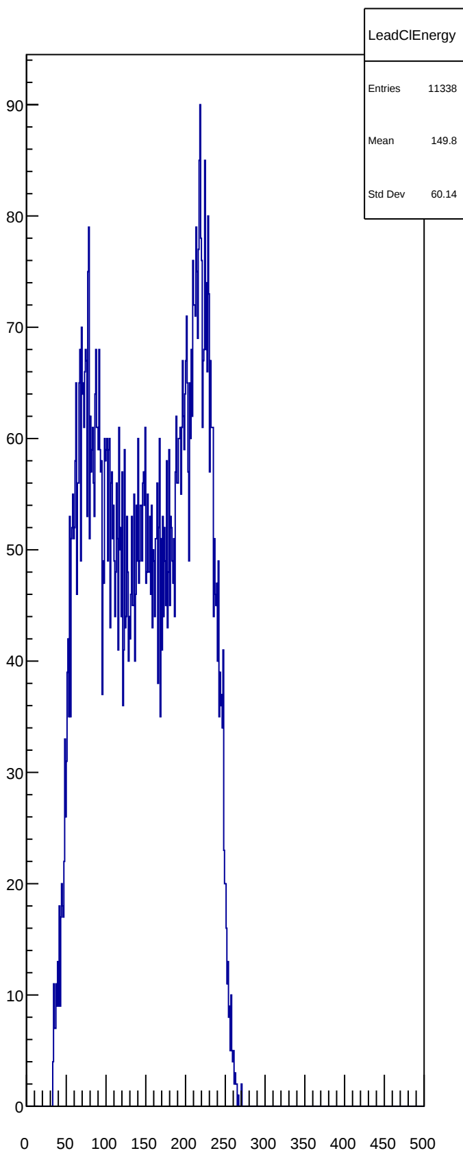
LeadClEnergy
