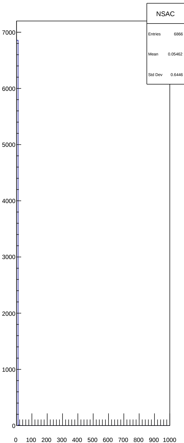
NSAC
