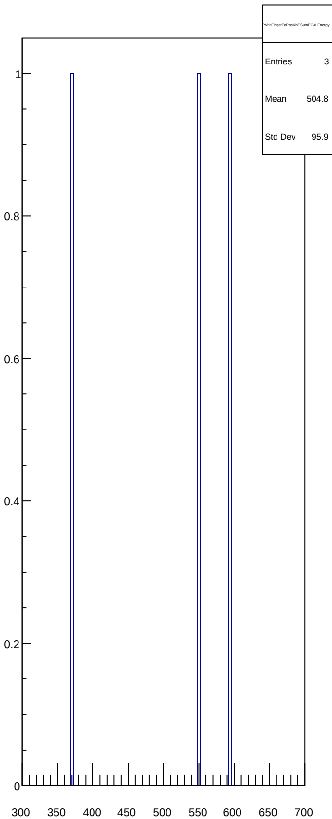
PVhitFingerToPosKinESumECALEnergy
