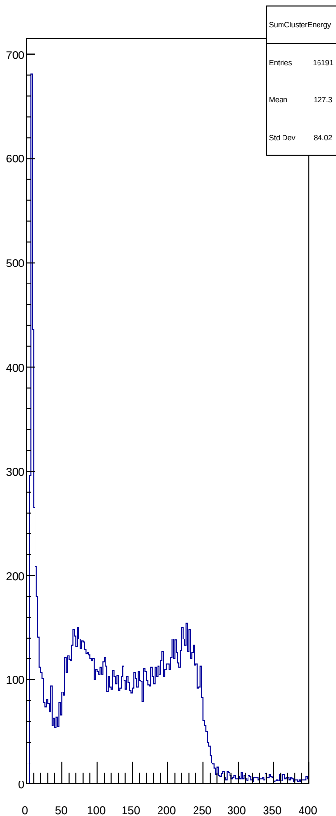
SumClusterEnergy
