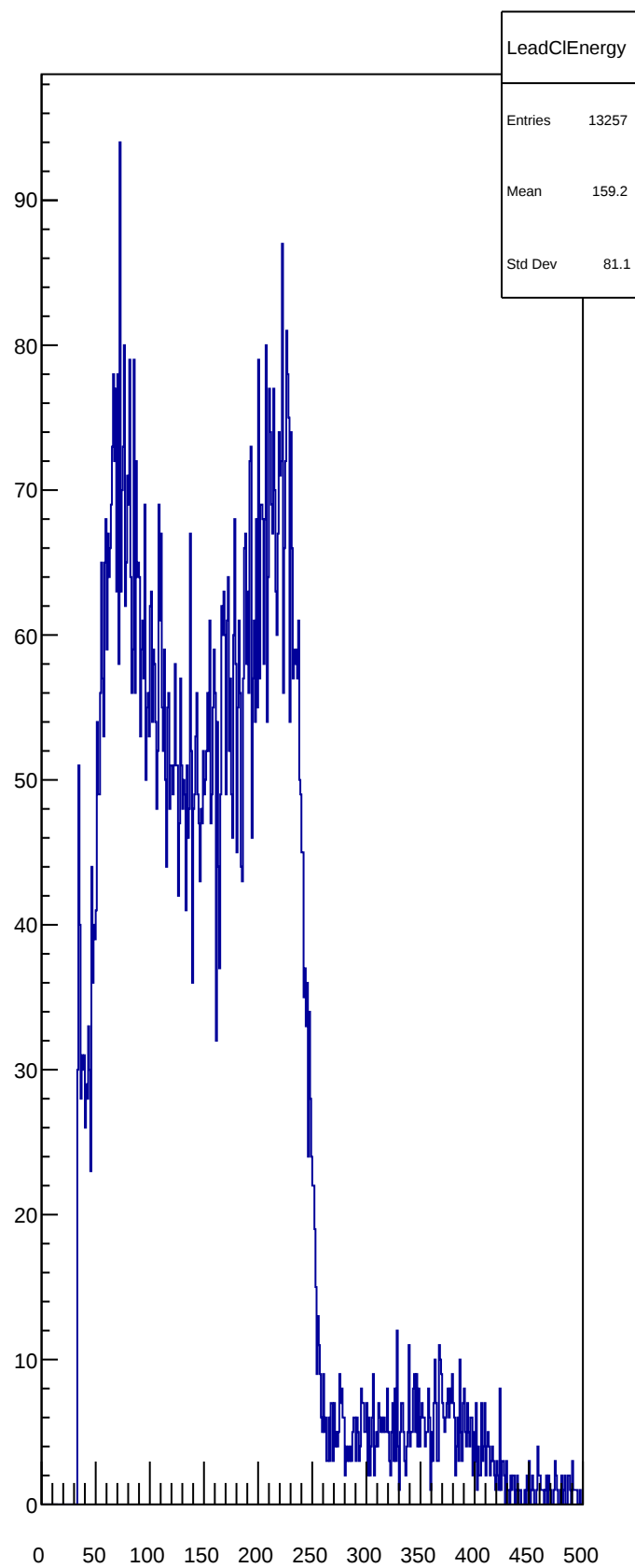
LeadClEnergy
