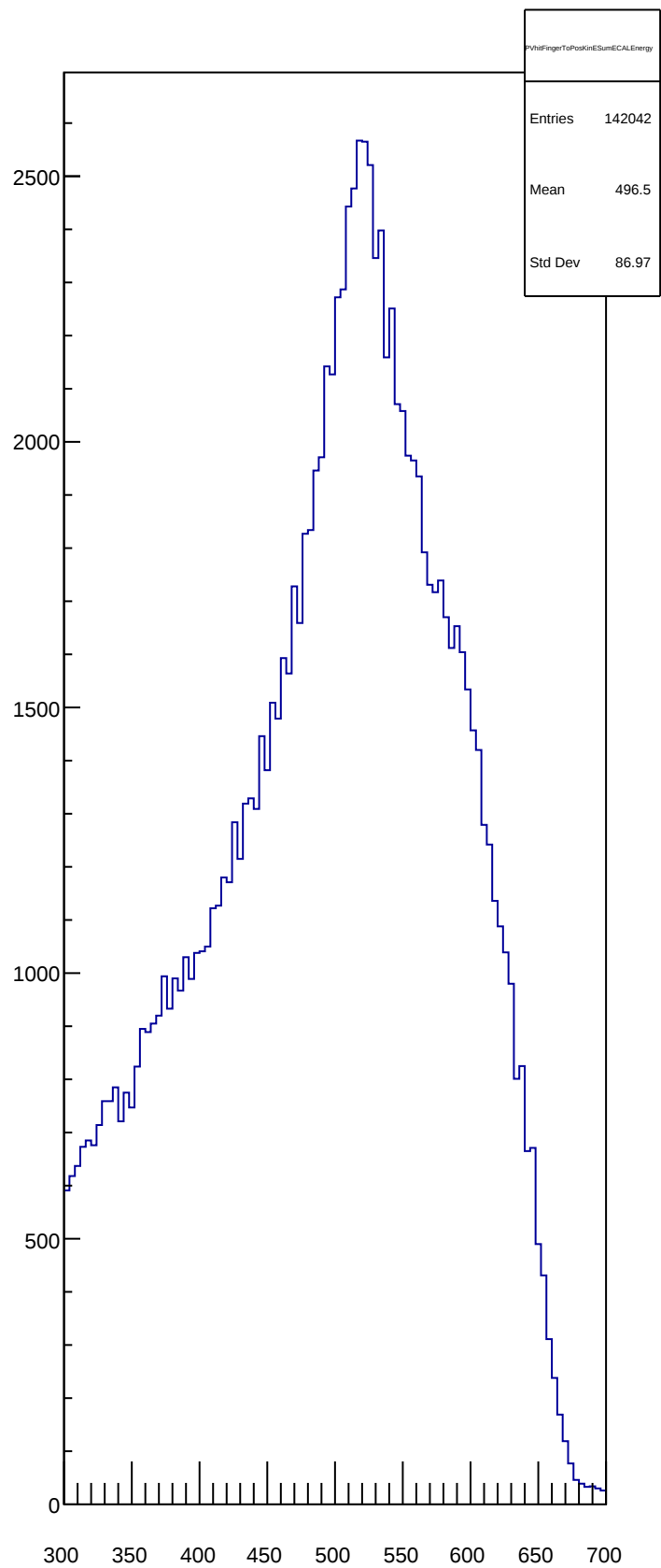
PVhitFingerToPosKinESumECALEnergy
