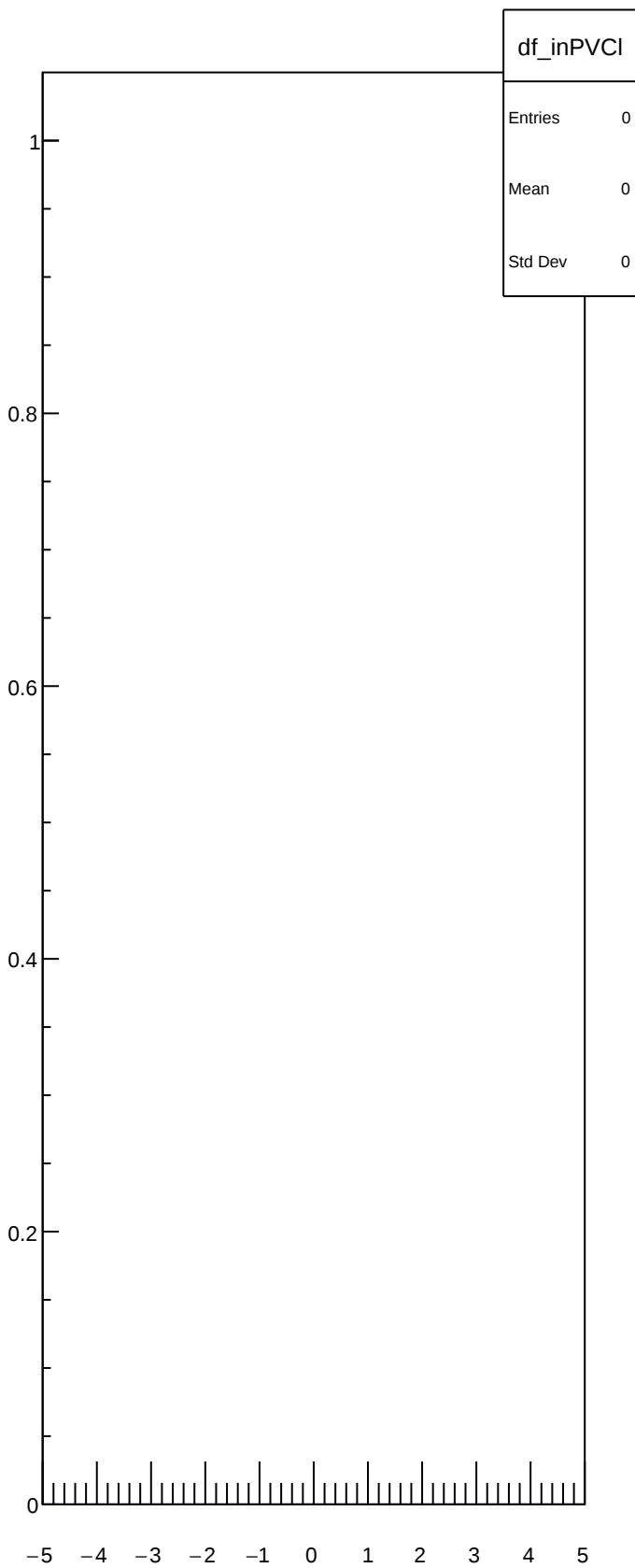
df_inPVCI
