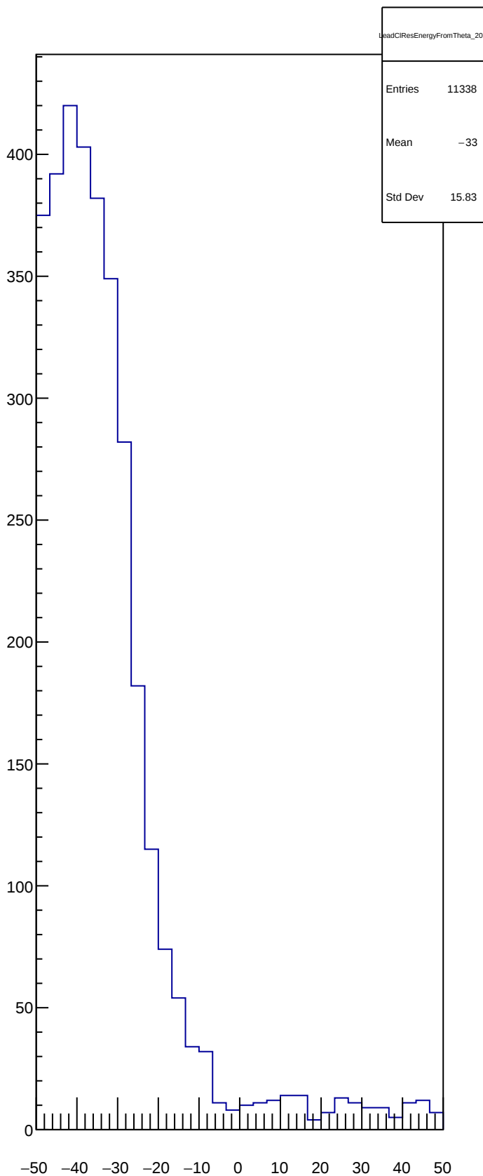
LeadCIResEnergyFromTheta_20
