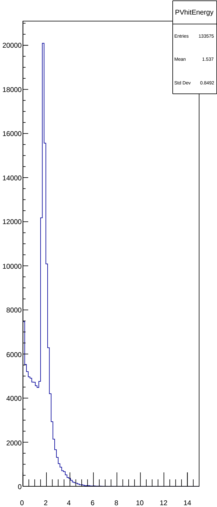
PVhitEnergy
