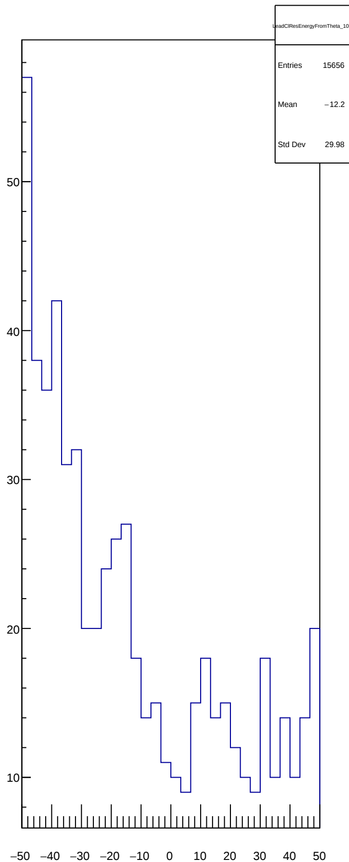
LeadCIResEnergyFromTheta_10
