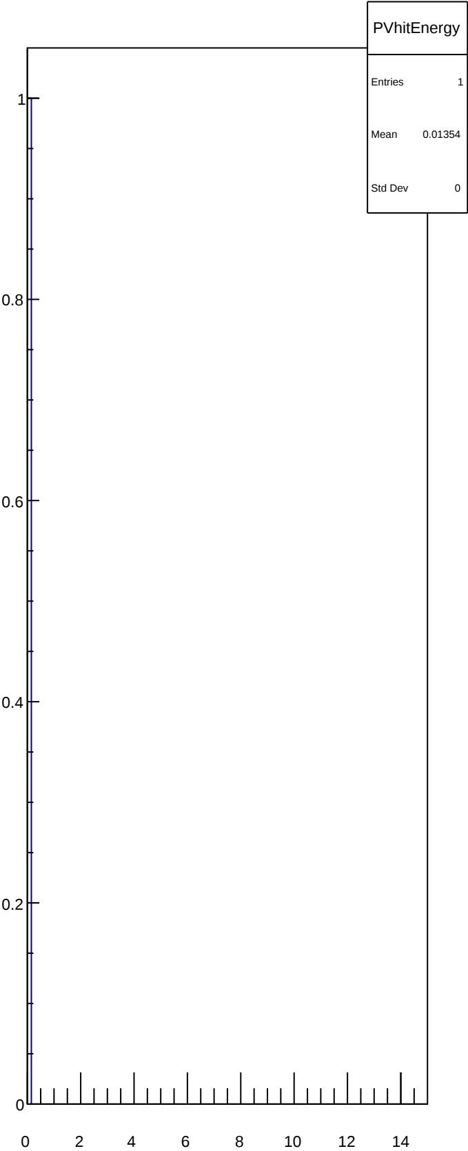
PVhitEnergy
