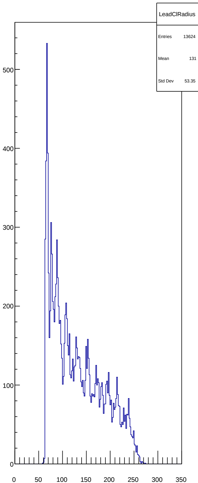
LeadCIRadius
