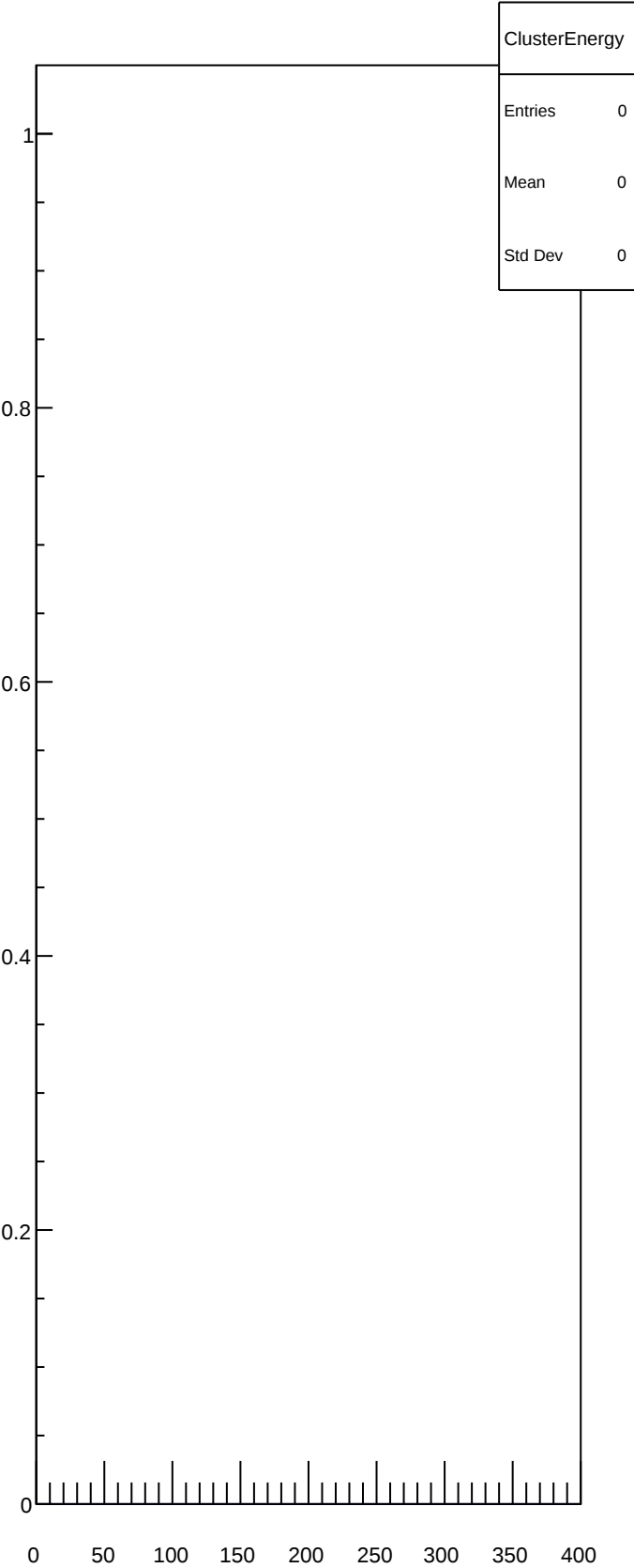
ClusterEnergy
