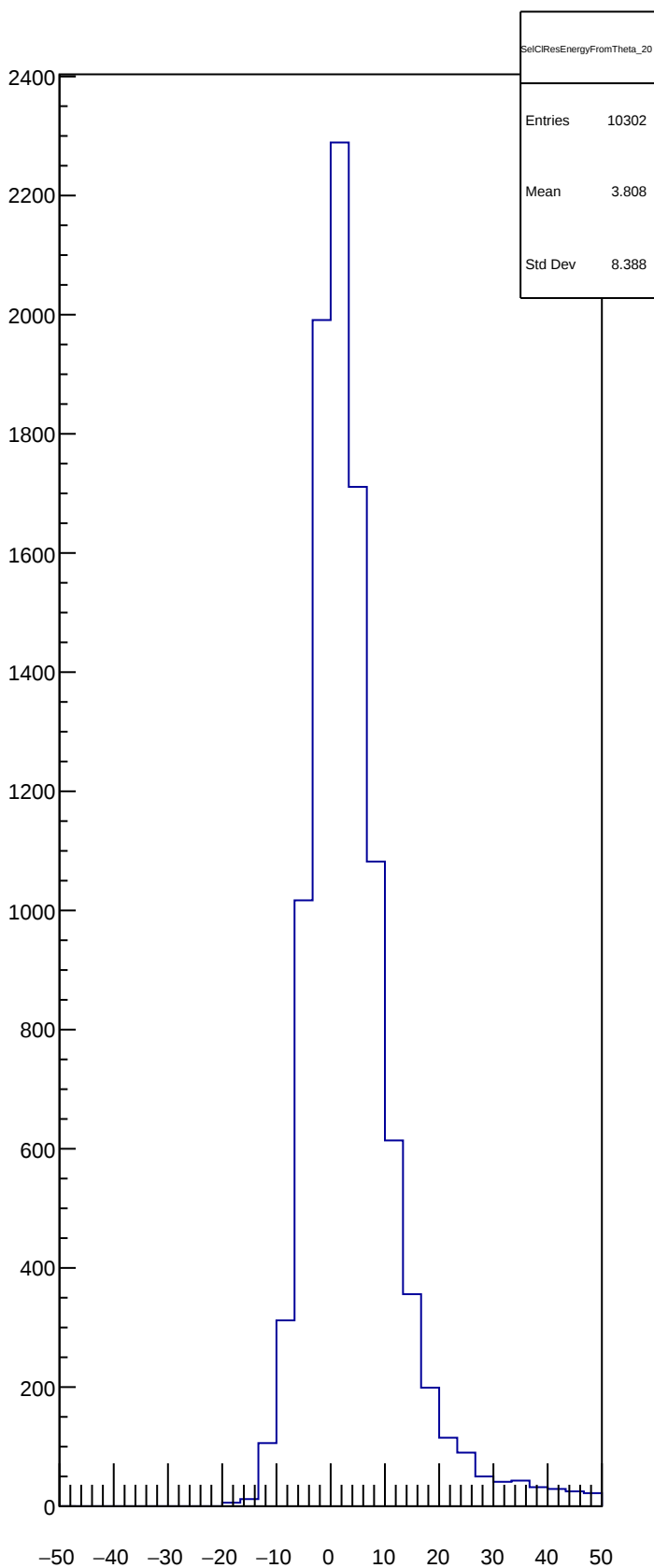
SelClResEnergyFromTheta_20
