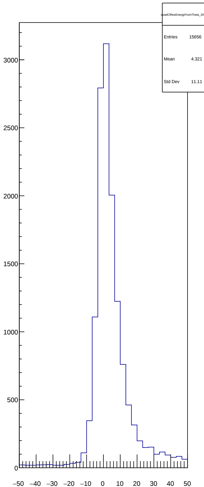
LeadCIResEnergyFromTheta_20
