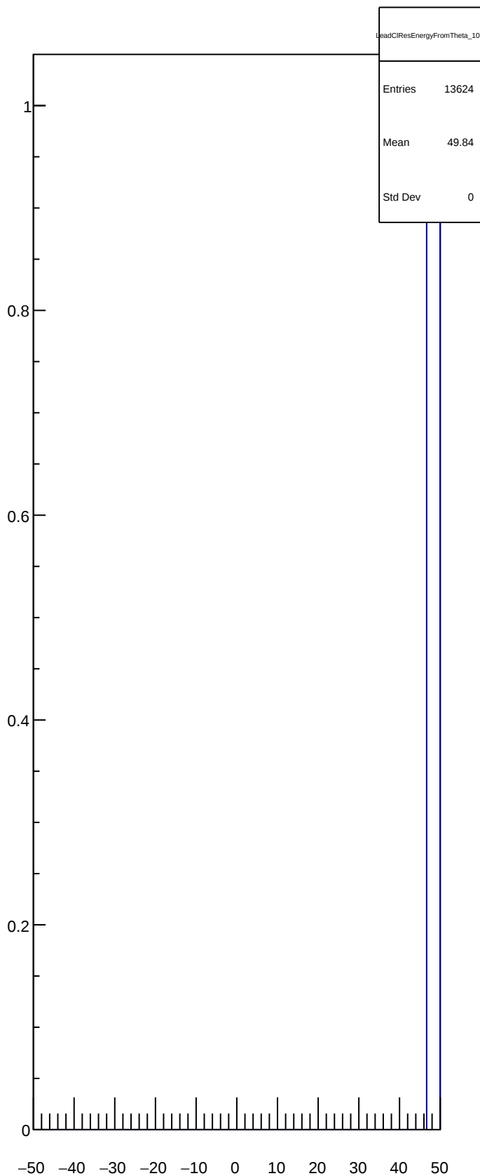
LeadCIResEnergyFromTheta_10
