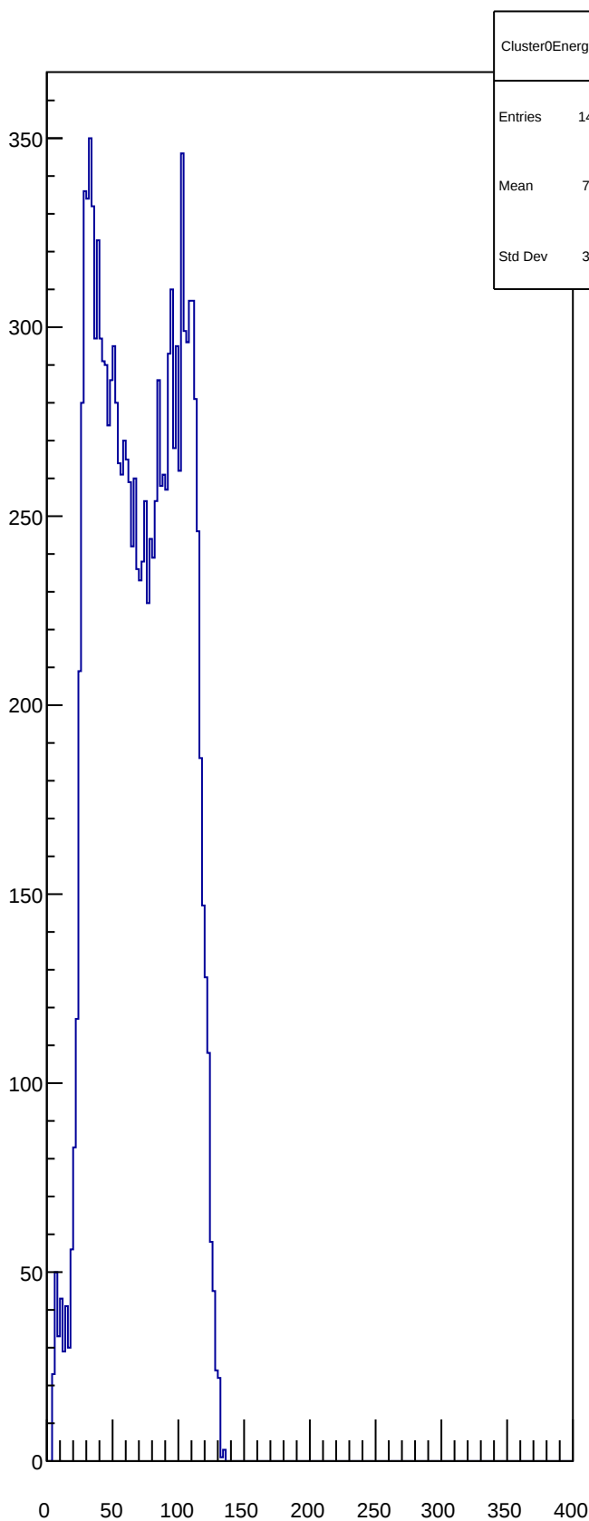
Cluster0Energy1Cl
