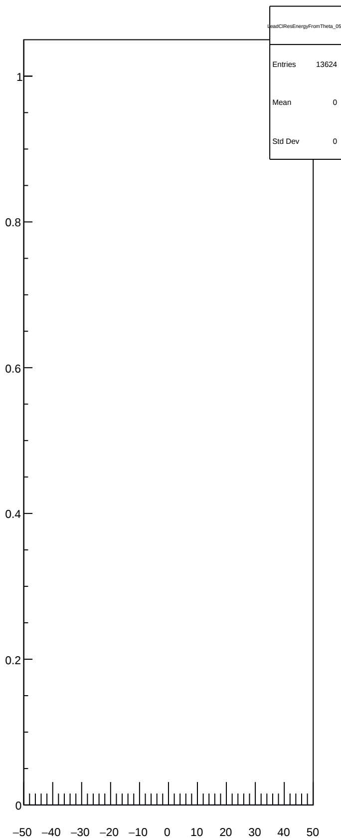
LeadCIResEnergyFromTheta_05
