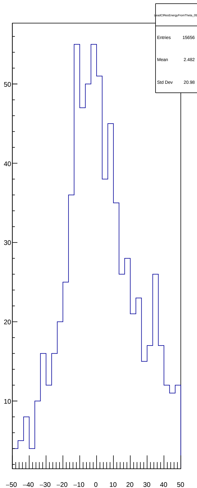
LeadCIResEnergyFromTheta_05
