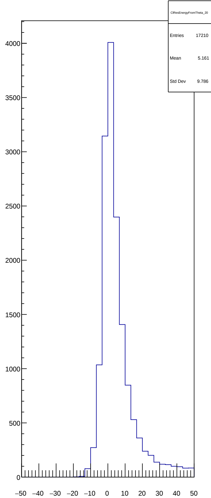
CIResEnergyFromTheta_20
