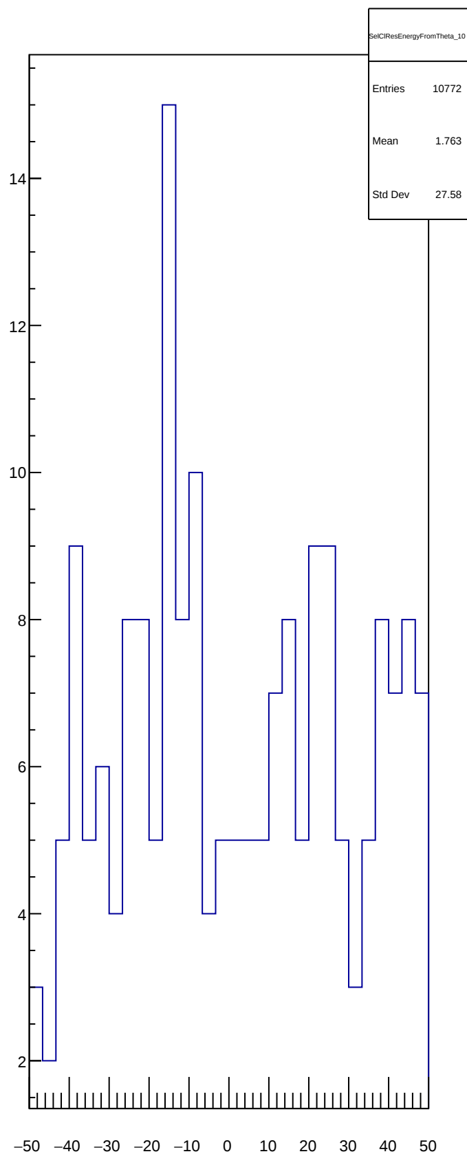
SelClResEnergyFromTheta_10
