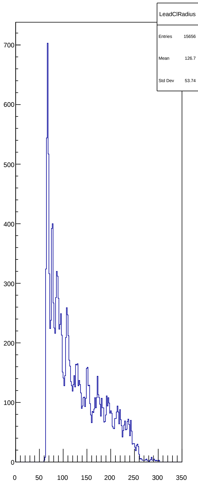
LeadCIRadius
