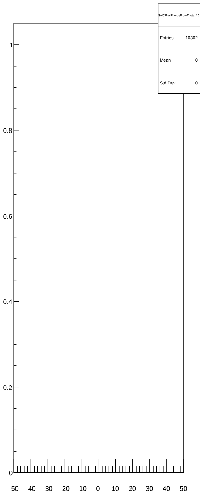
SelClResEnergyFromTheta_10
