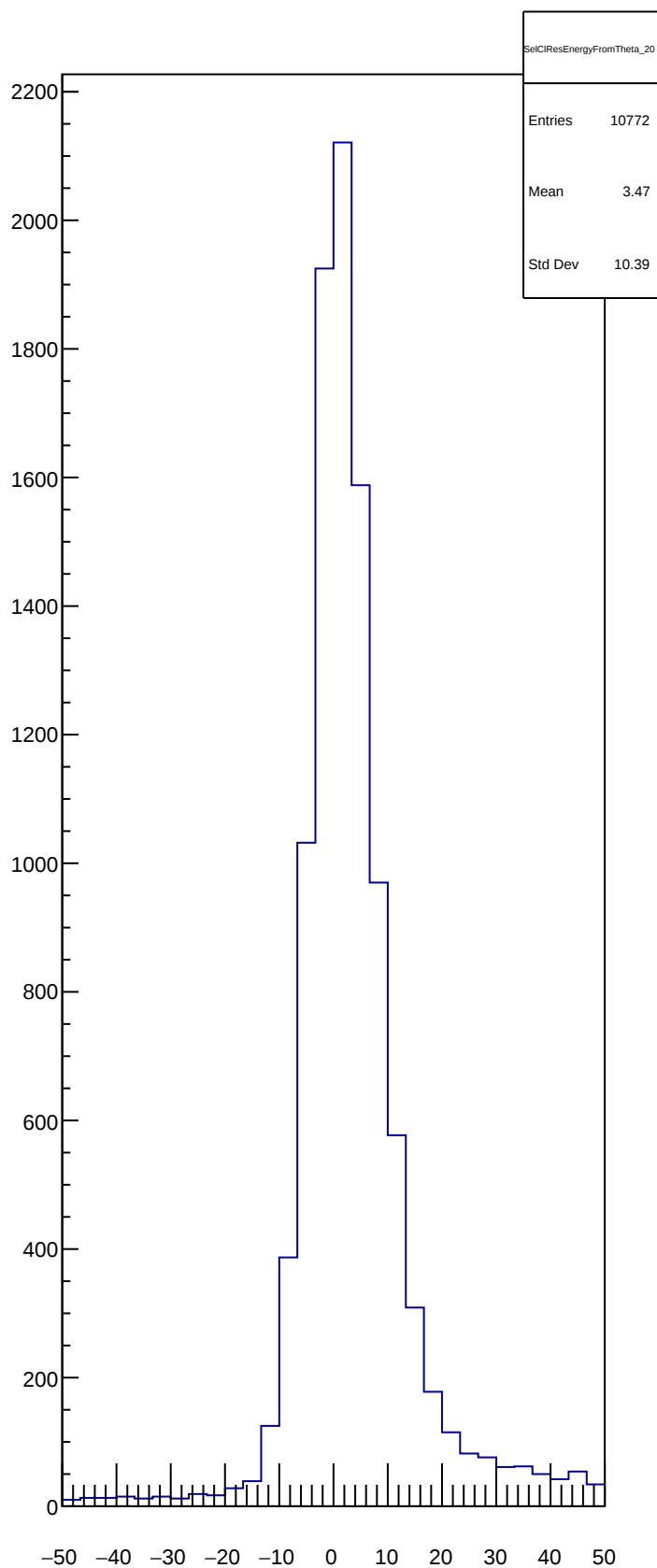
SelClResEnergyFromTheta_20
