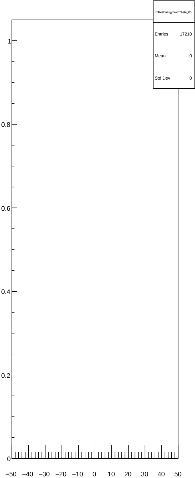
CIResEnergyFromTheta_05
