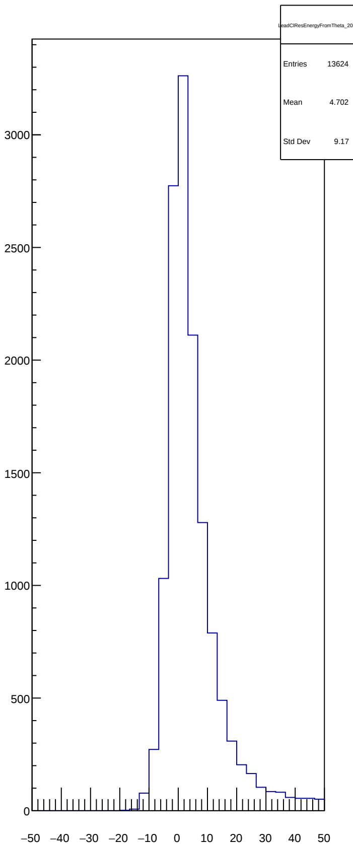
LeadCIResEnergyFromTheta_20
