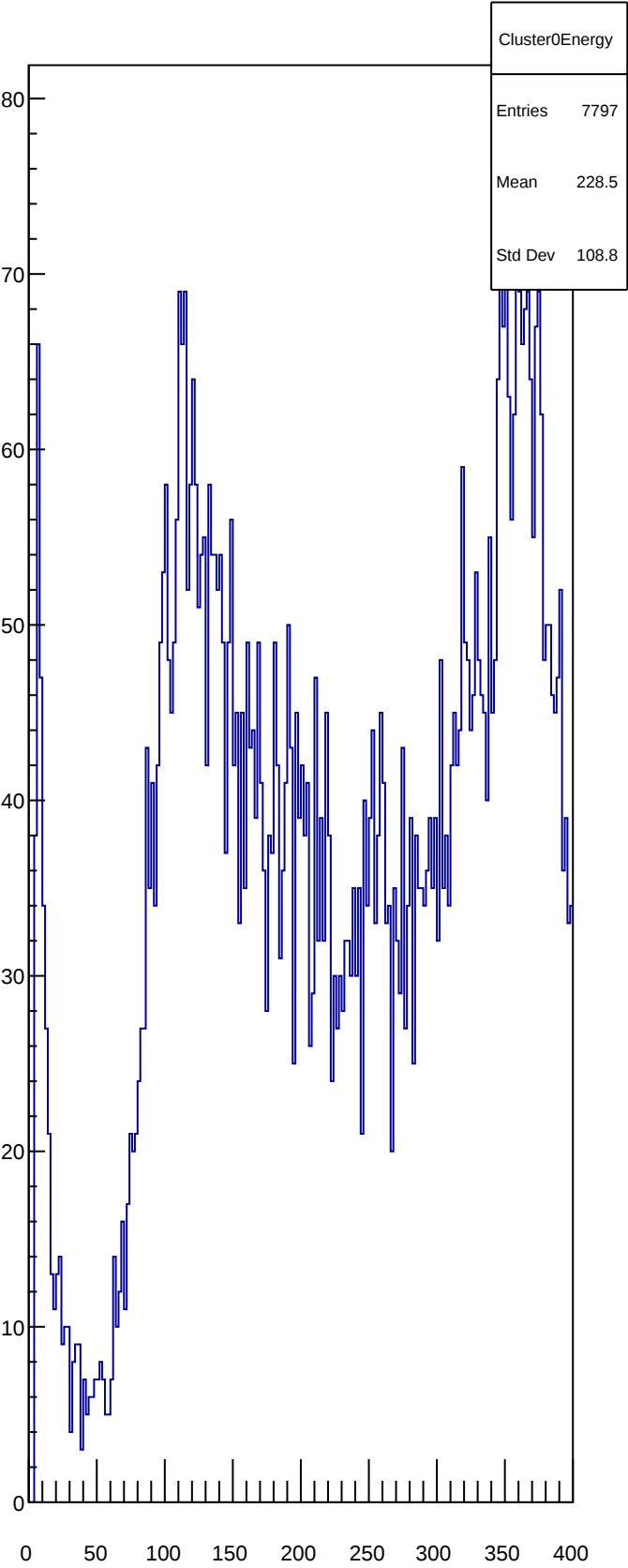
Cluster0Energy
