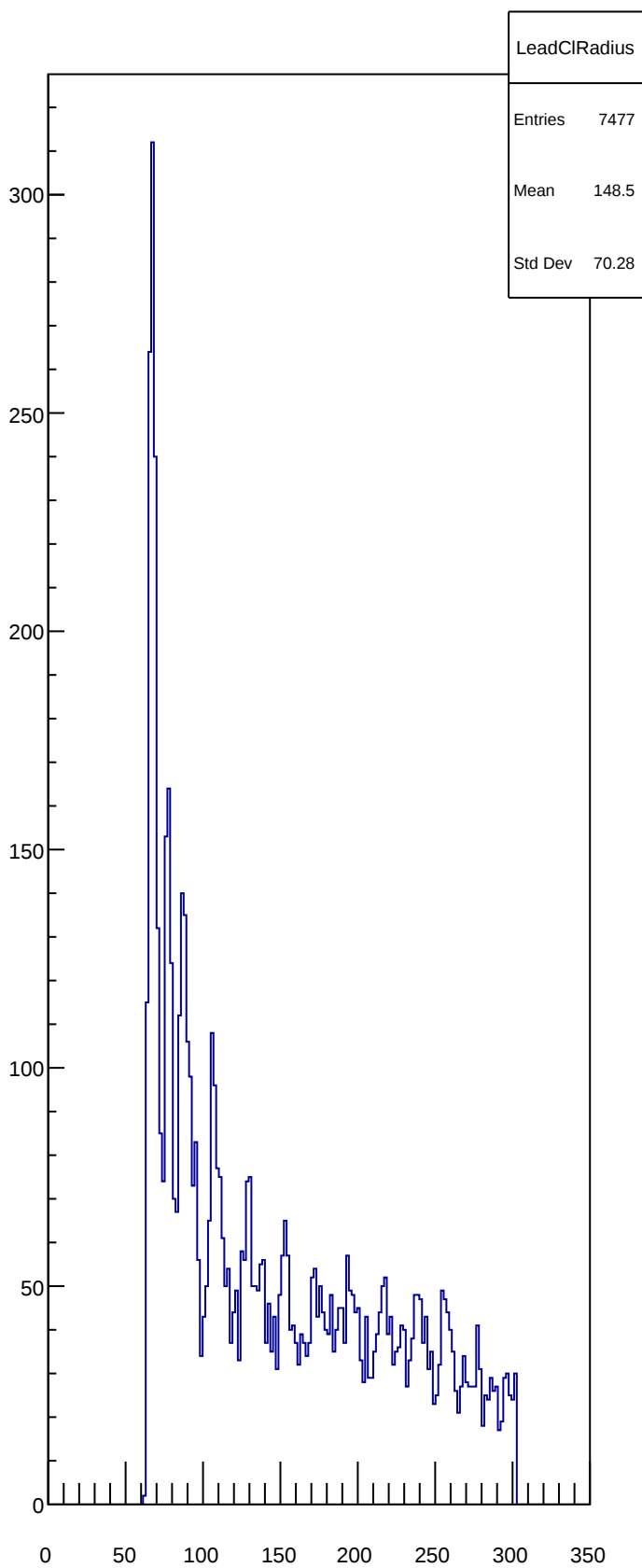
LeadCIRadius
