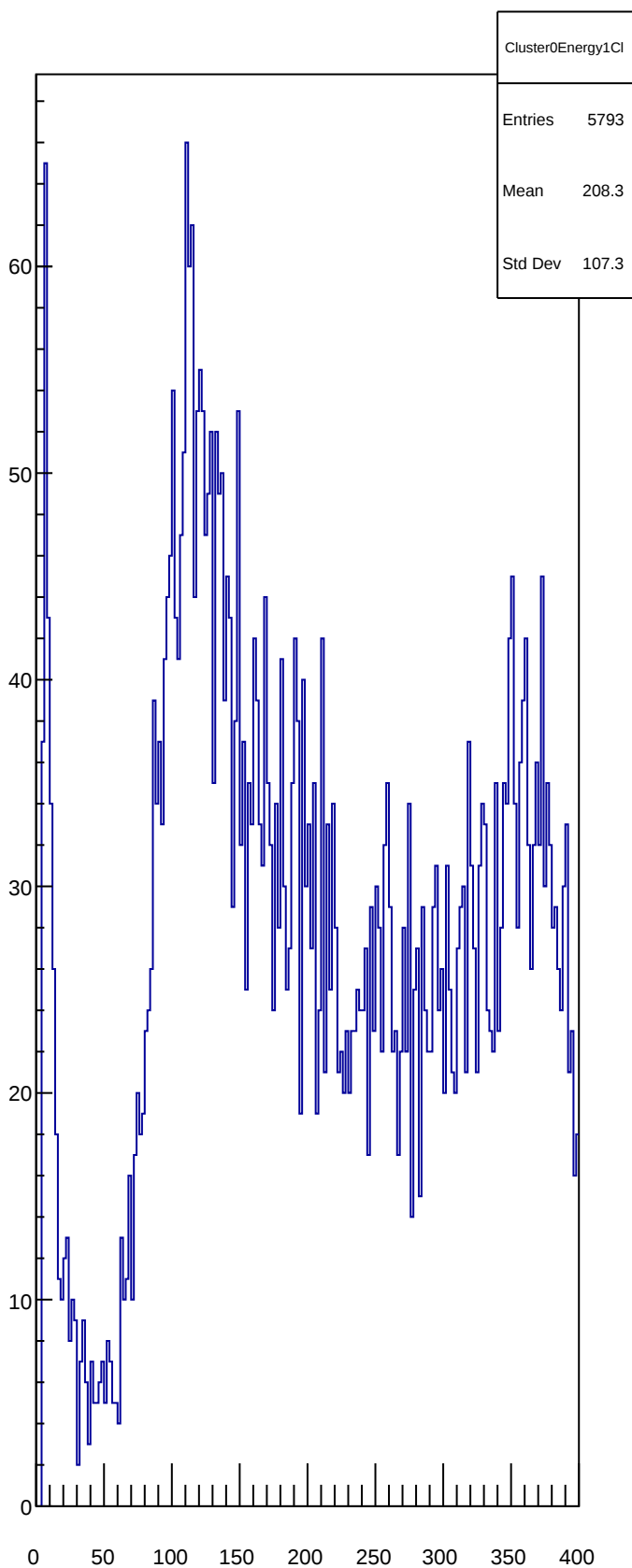
Cluster0Energy1Cl
