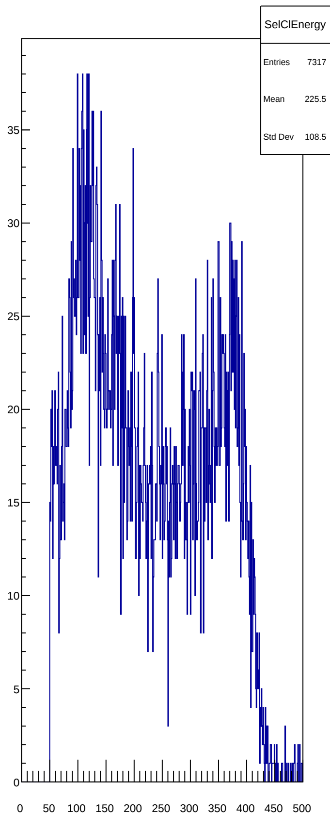
SelClEnergy
