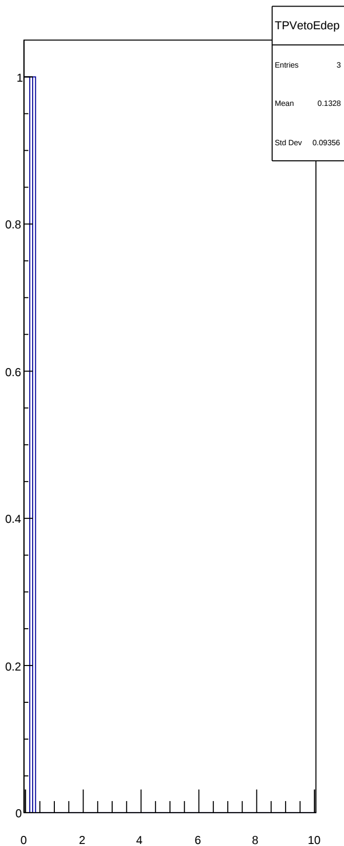
TPVetoEdep
