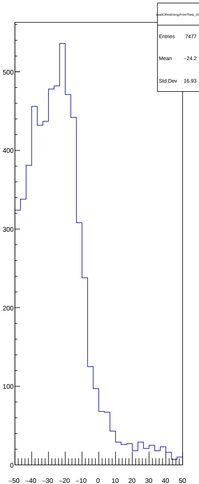
LeadCIResEnergyFromTheta_10
