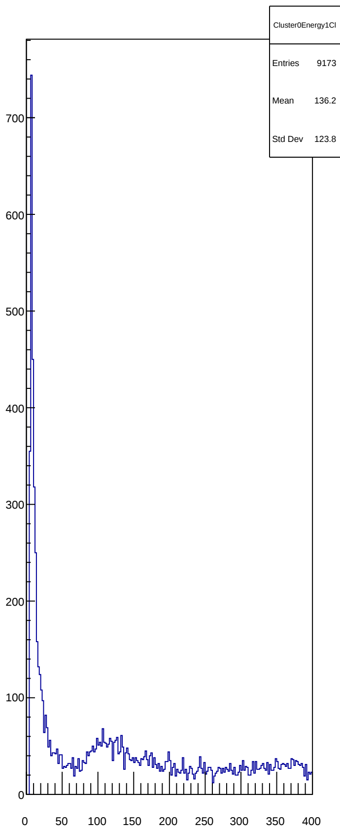
Cluster0Energy1Cl
