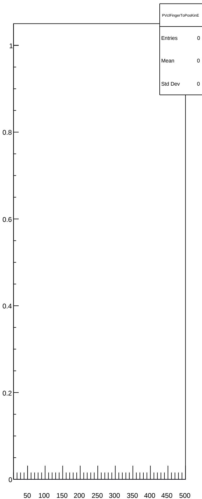
PVclFingerToPosKinE
