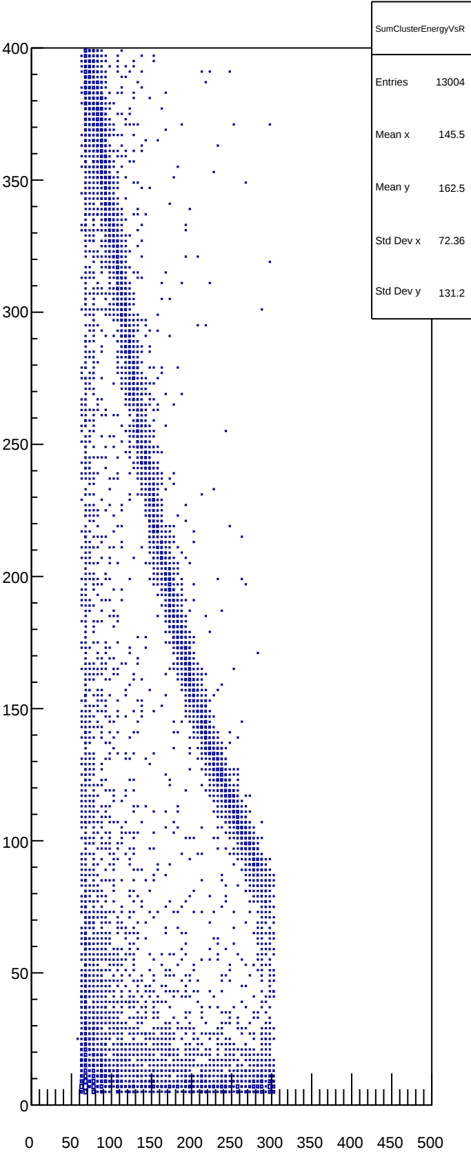
SumClusterEnergyVsR
