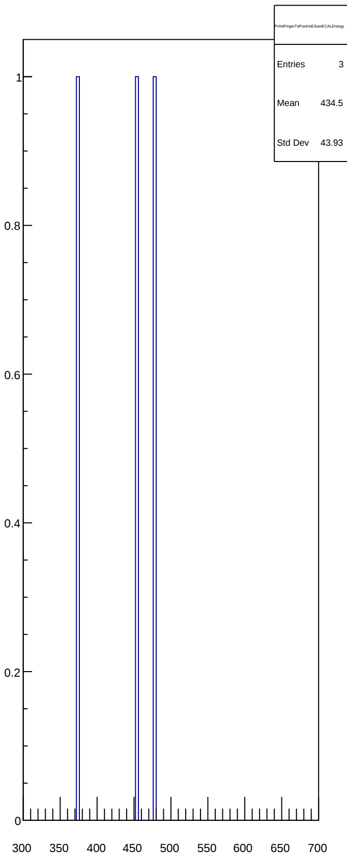
PVhitFingerToPosKinESumECALEnergy
