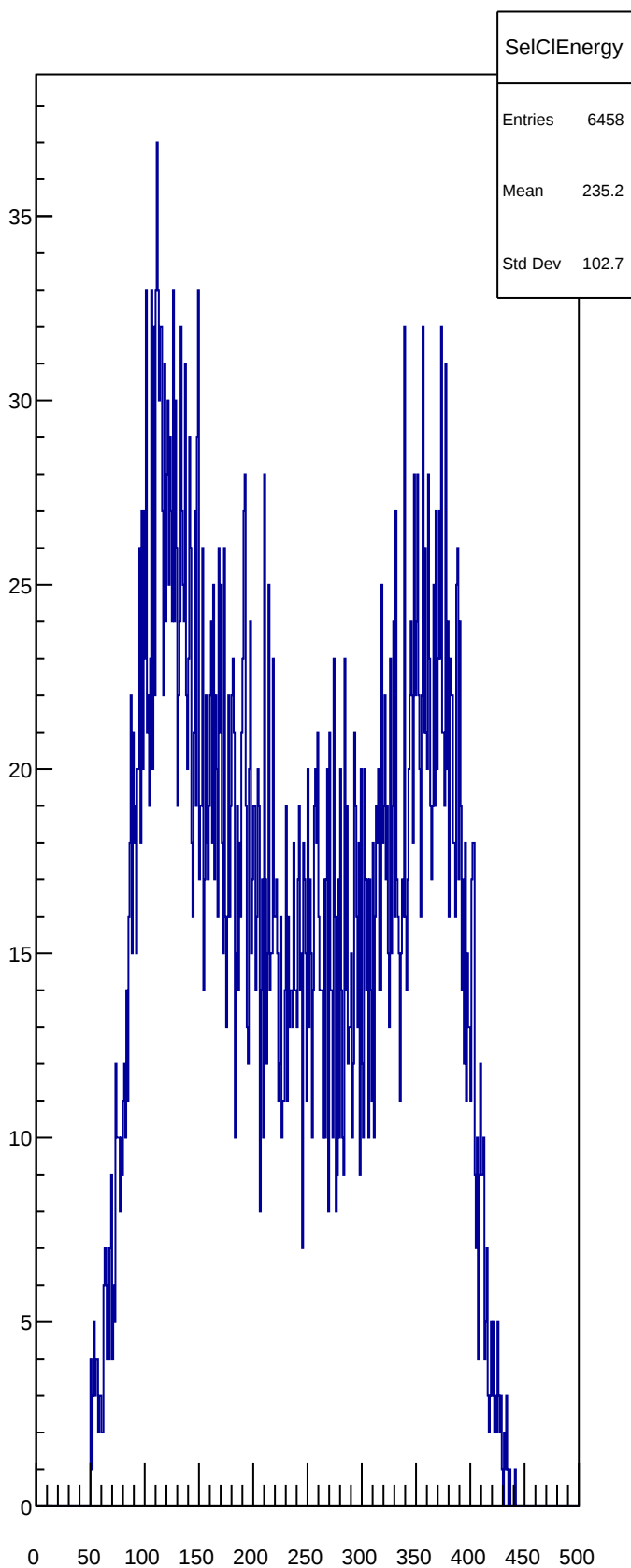
SelClEnergy
