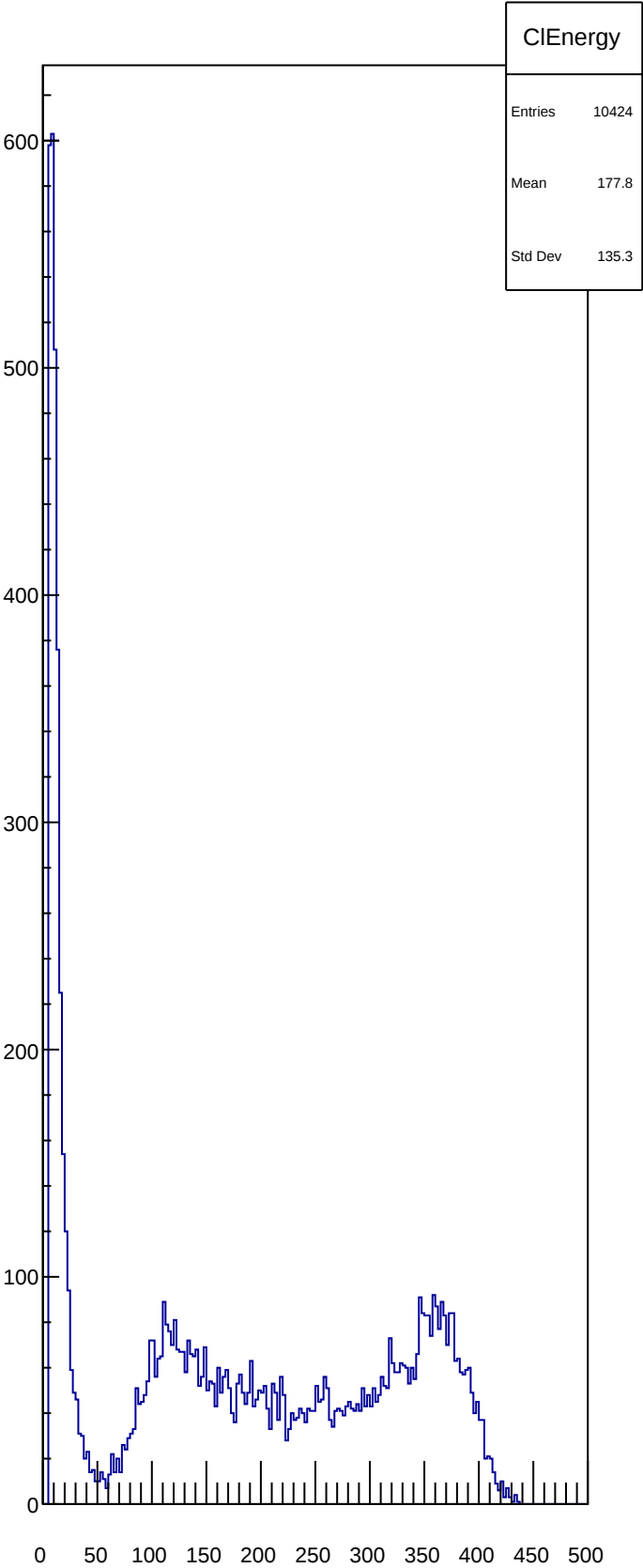
CIEnergy
