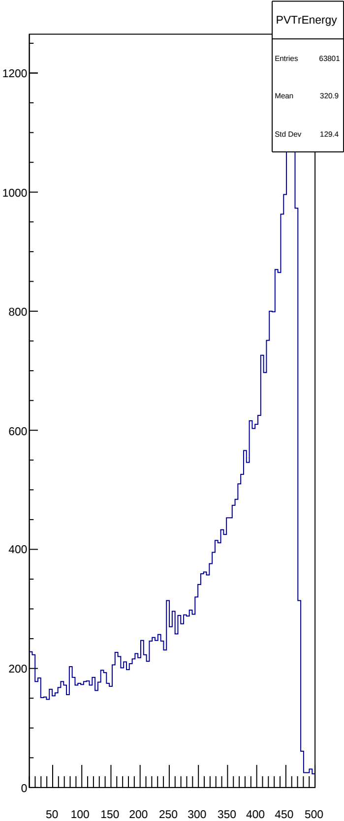
PVTrEnergy
