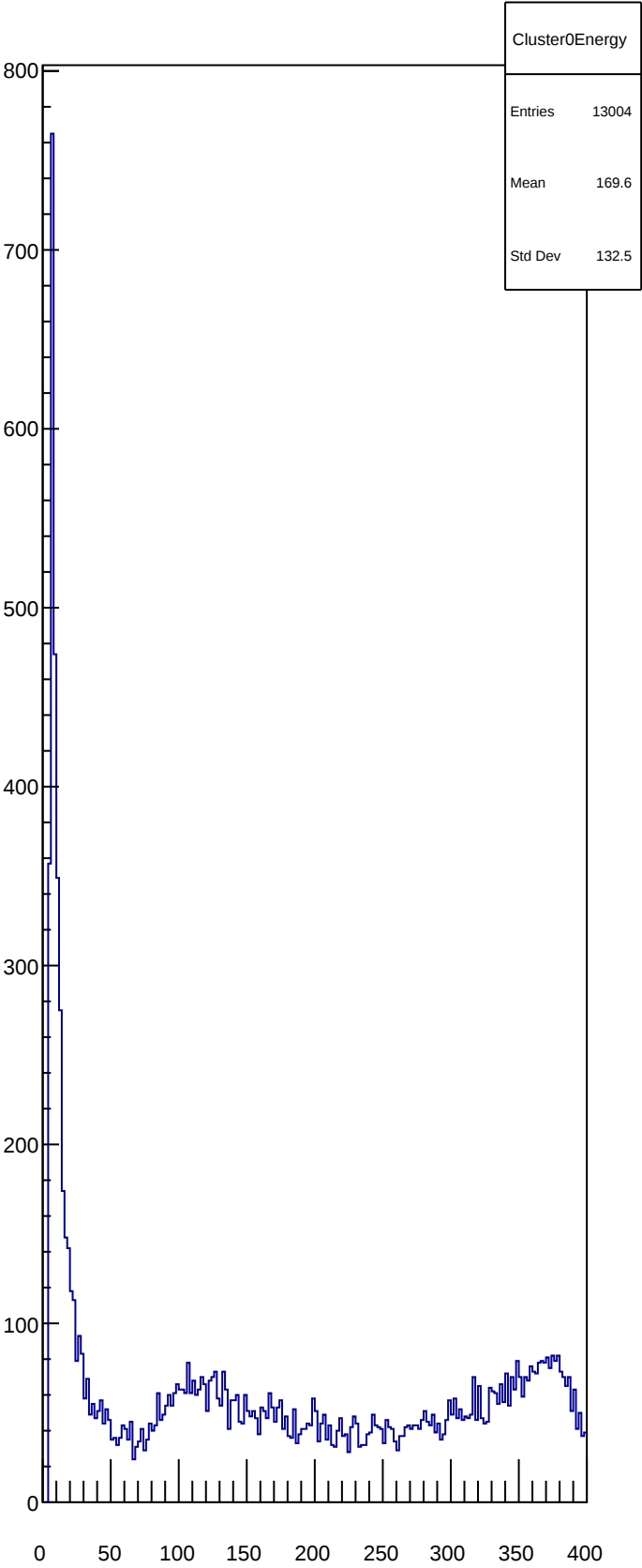
Cluster0Energy
