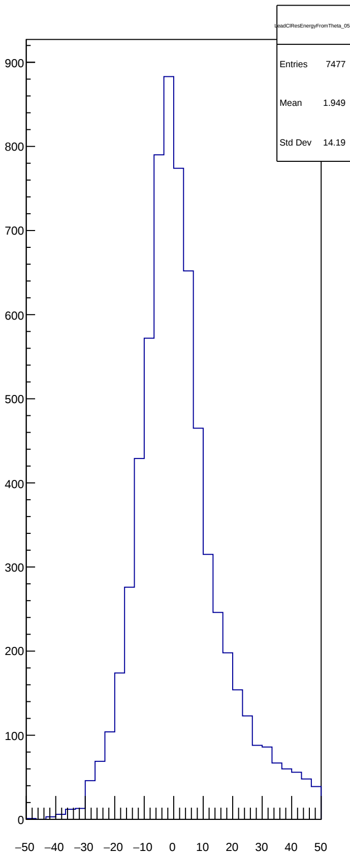
LeadCIResEnergyFromTheta_05
