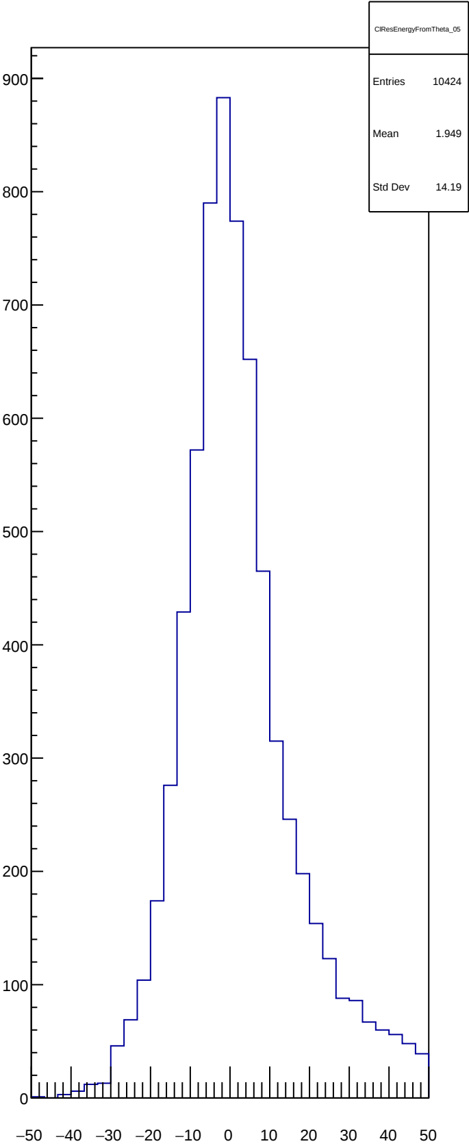
CIResEnergyFromTheta_05
