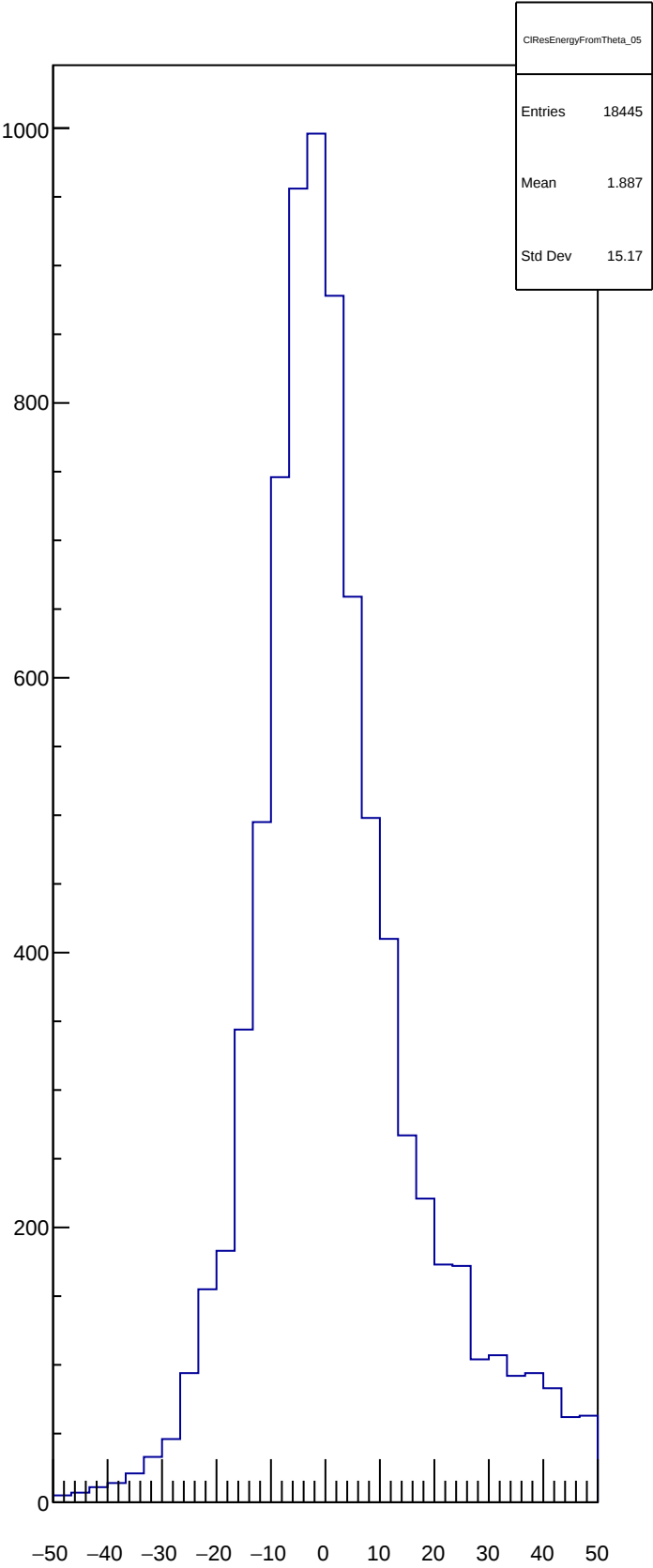
CIResEnergyFromTheta_05
