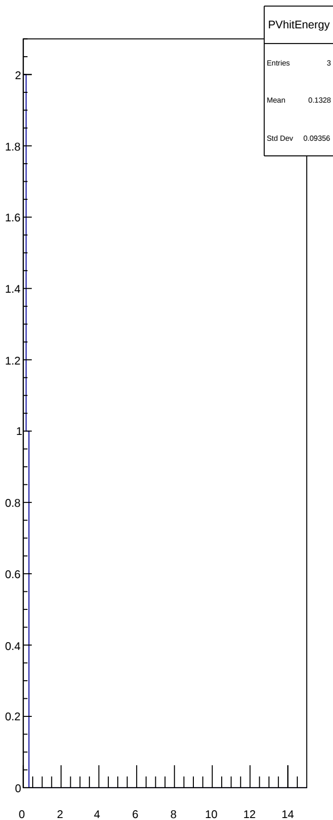
PVhitEnergy
