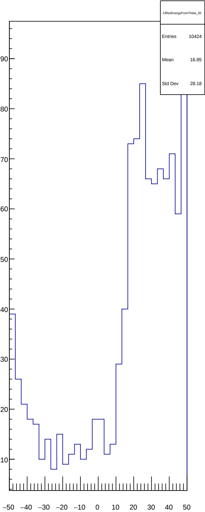
CIResEnergyFromTheta_20
