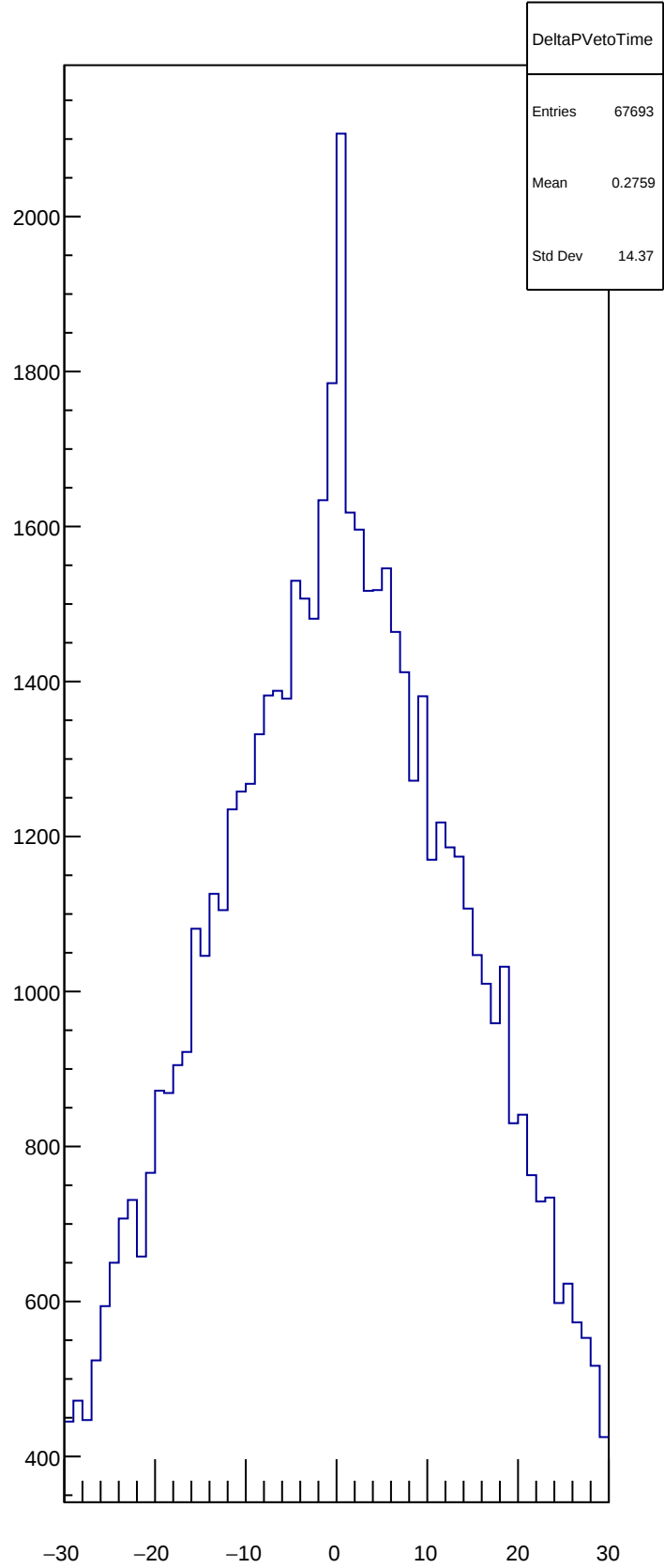
DeltaPVetoTime
