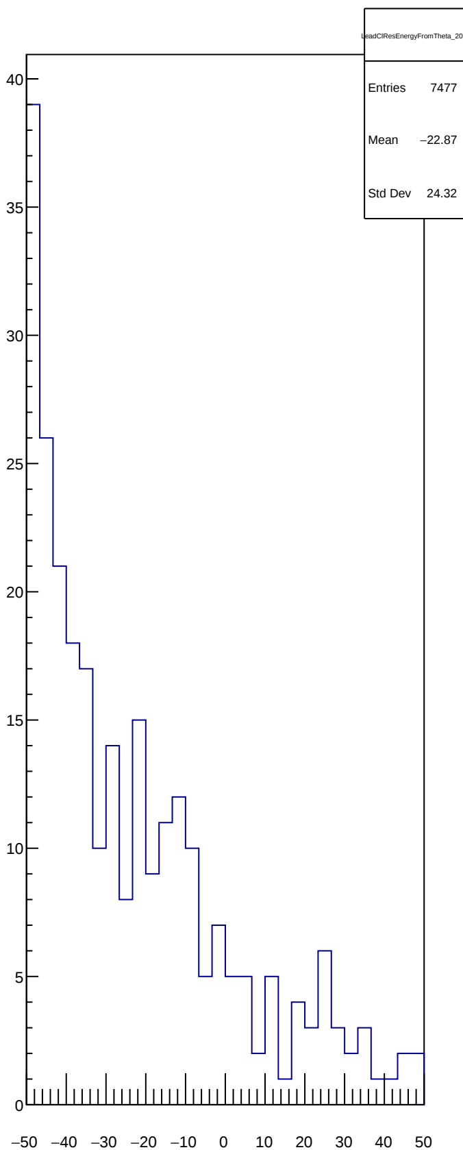
LeadCIResEnergyFromTheta_20
