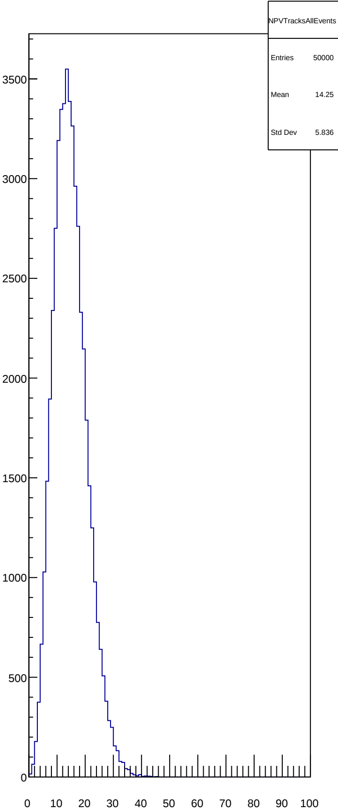
NPVTracksAllEvents
