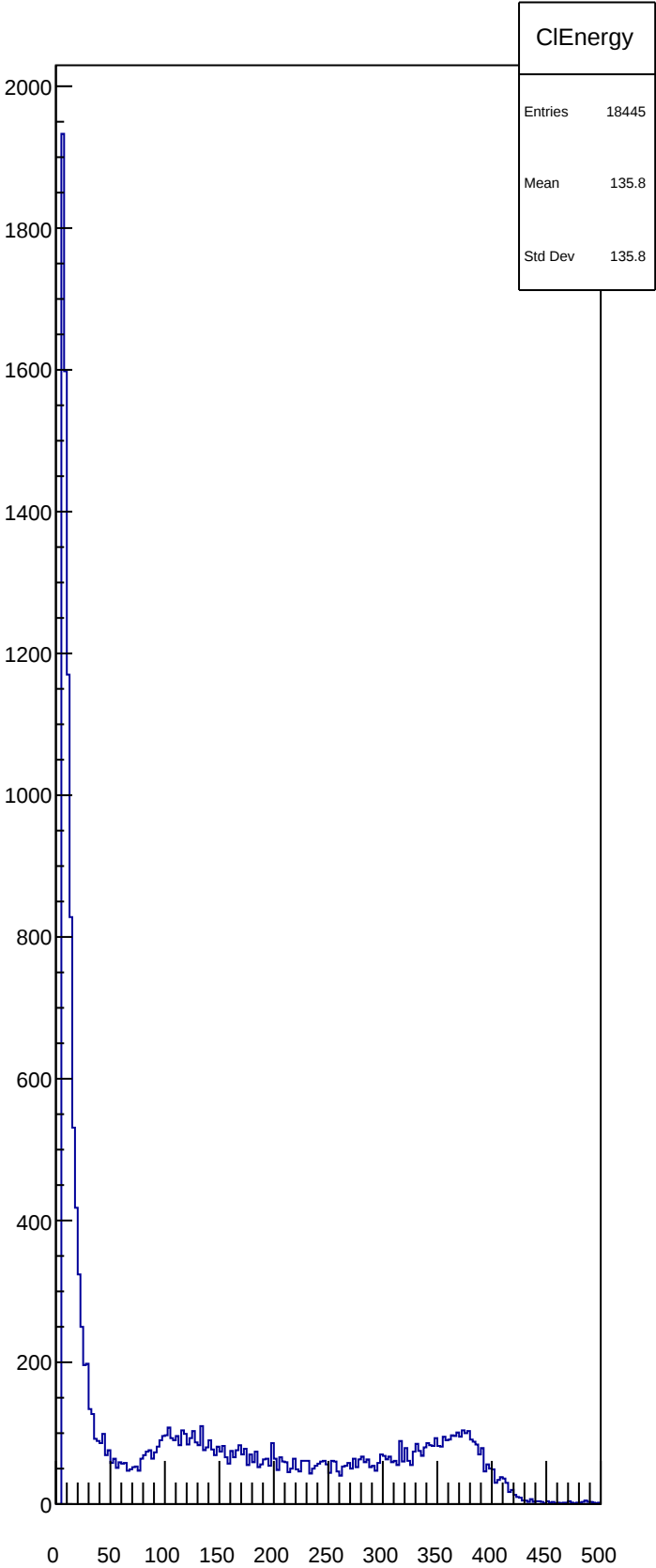
CIEnergy
