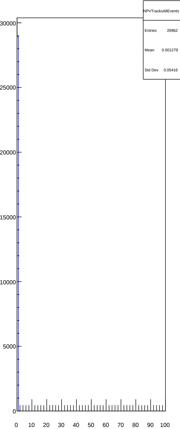
NPVTracksAllEvents
