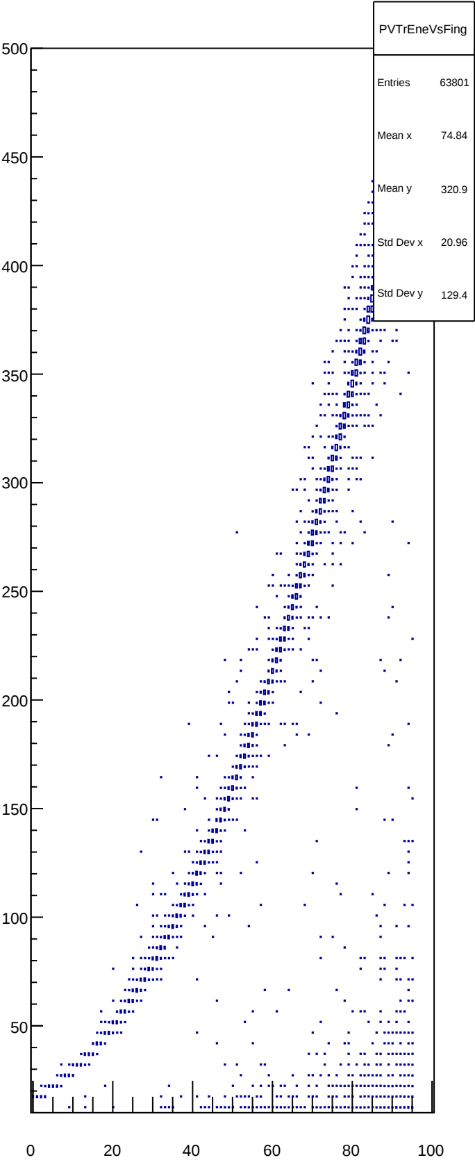
PVTrEneVsFing
