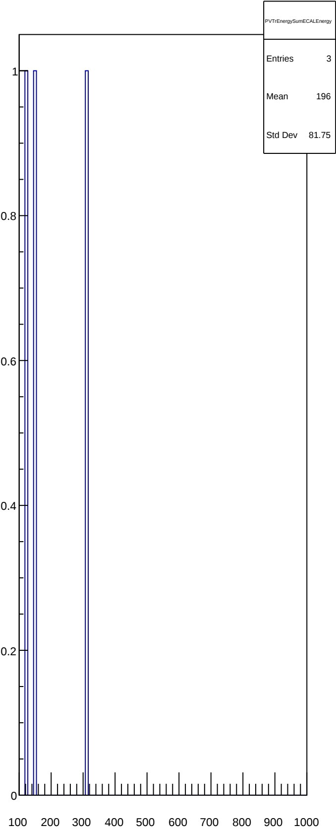
PVTrEnergySumECALEnergy
