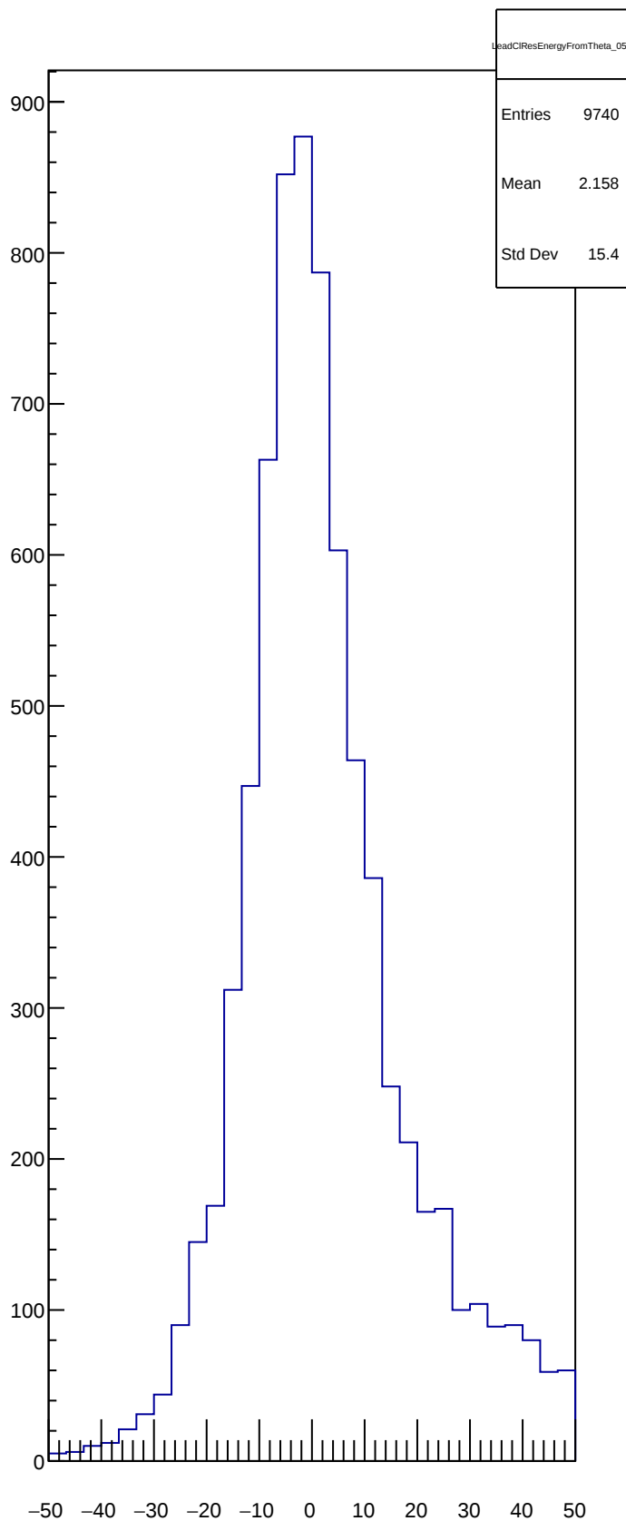
LeadCIResEnergyFromTheta_05
