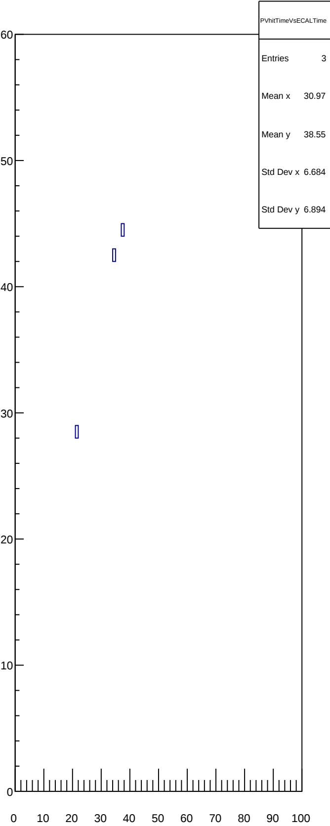
PVhitTimeVsECALTime
