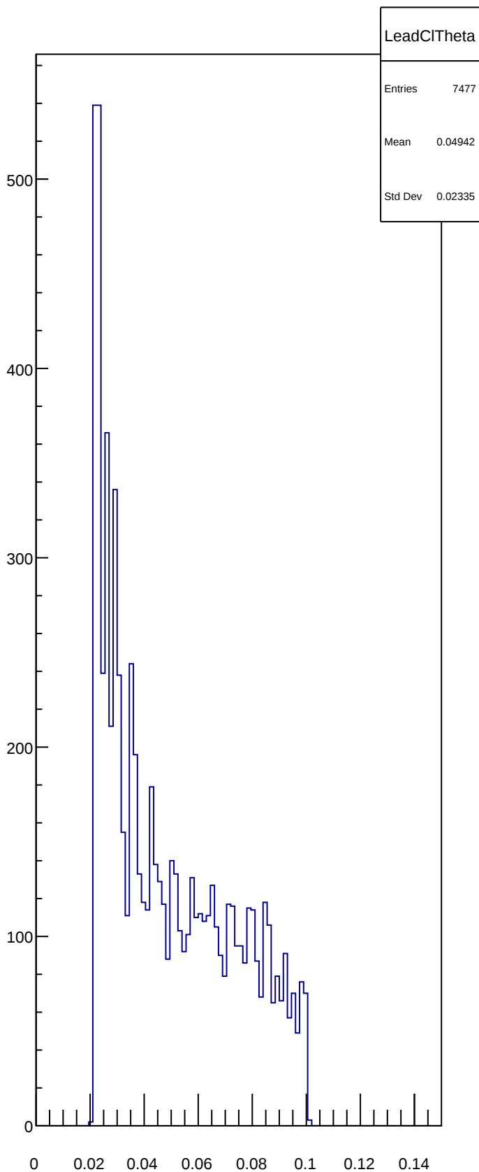
LeadCITheta
