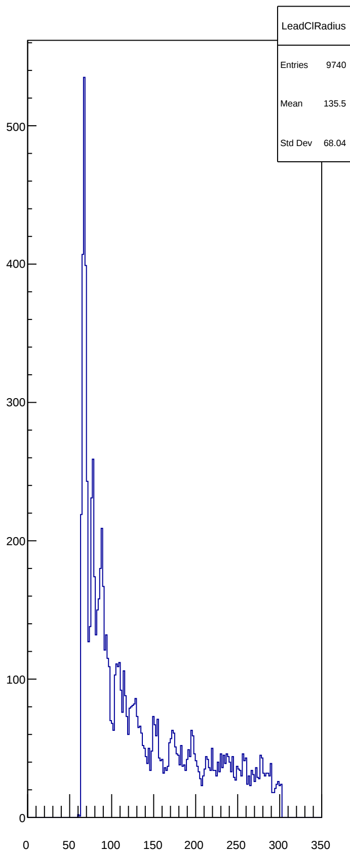
LeadCIRadius
