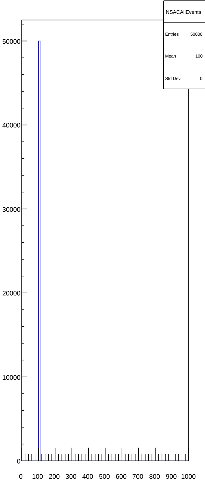
NSACAllEvents
