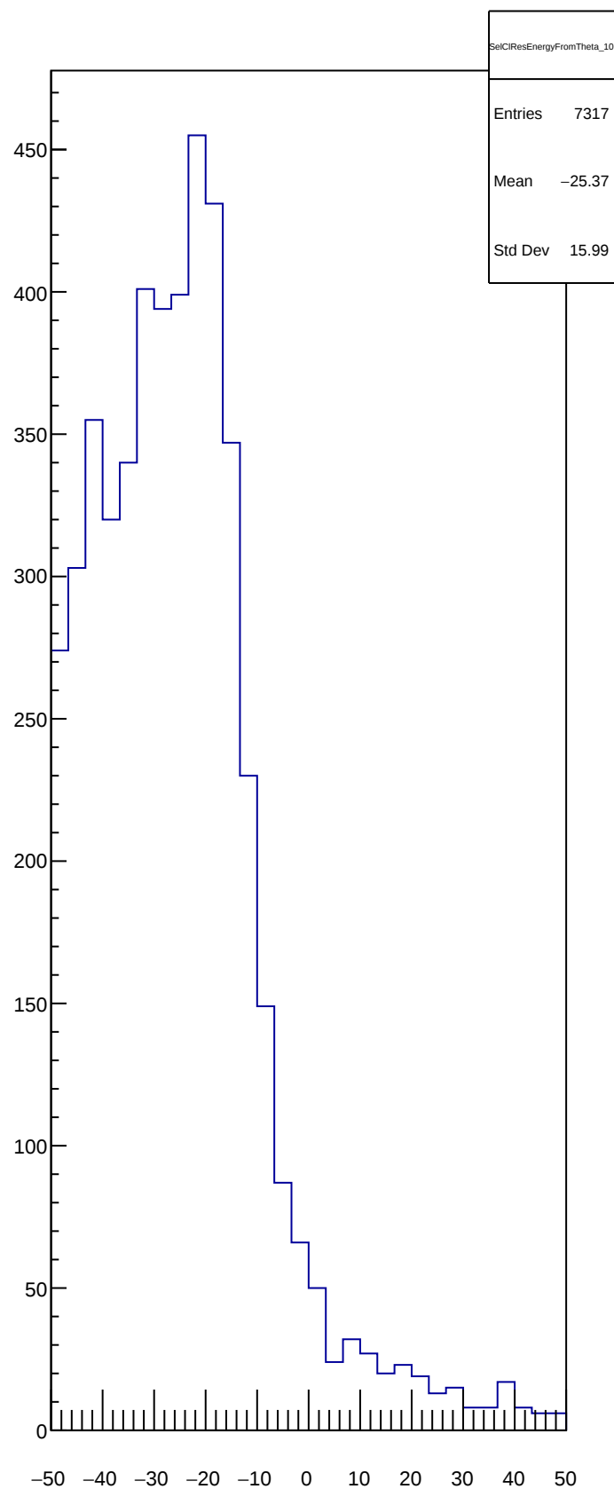
SelClResEnergyFromTheta_10
