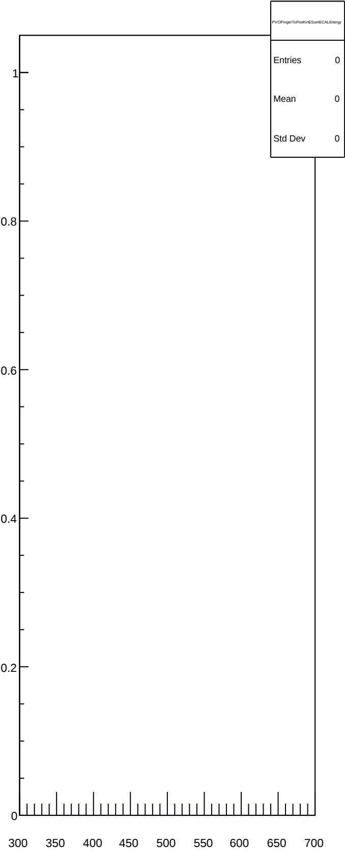
PVCFingerToPosKinESumECALEnergy
