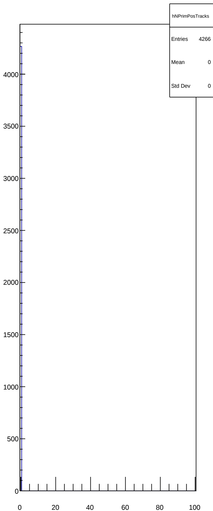
hNPrimPosTracks
