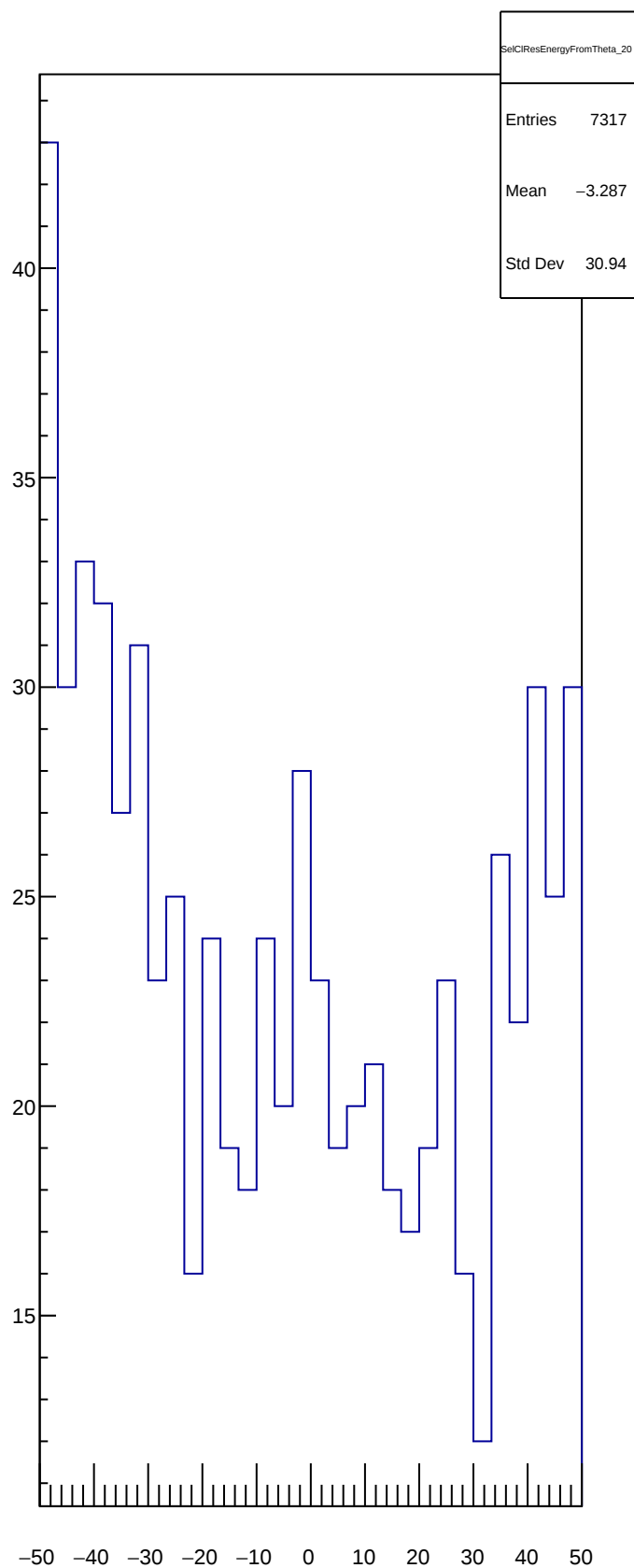
SelClResEnergyFromTheta_20
