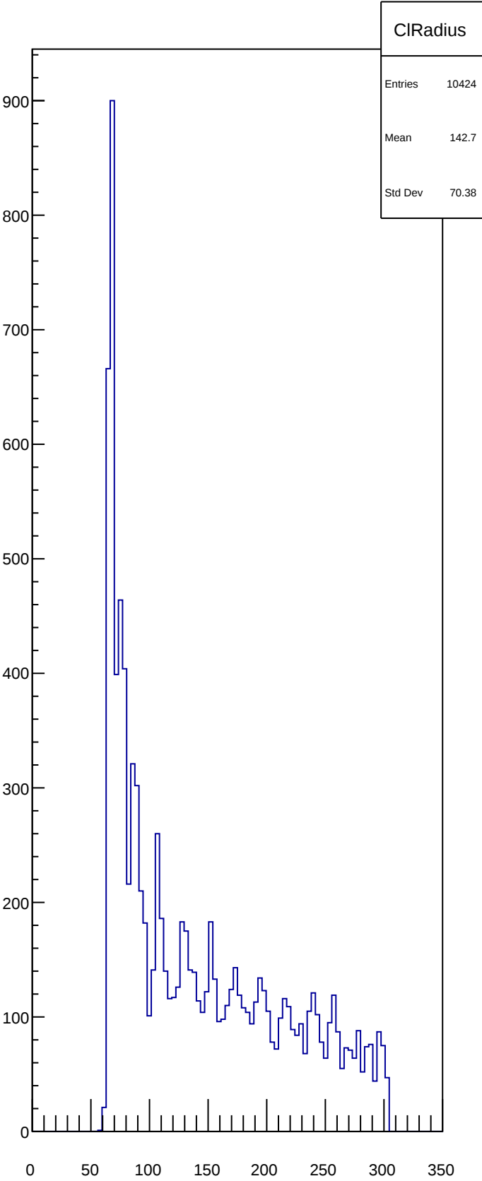
CIRadius
