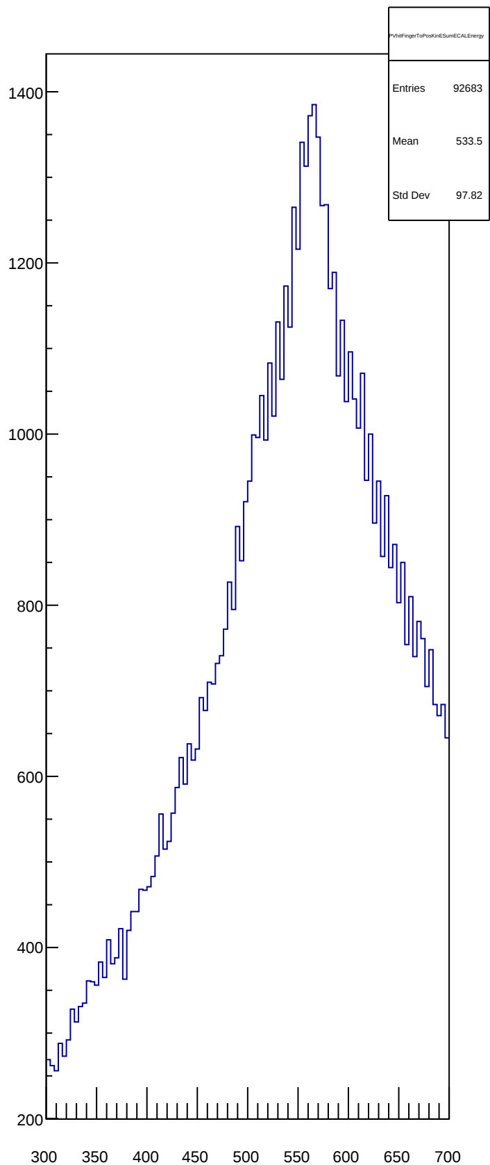
PVhitFingerToPosKinESumECALEnergy
