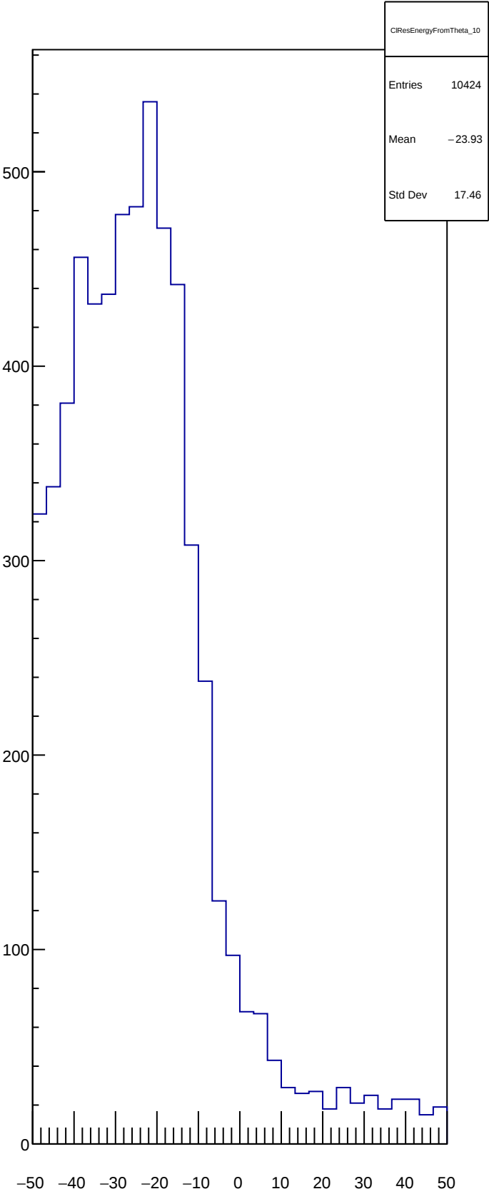
CIResEnergyFromTheta_10
