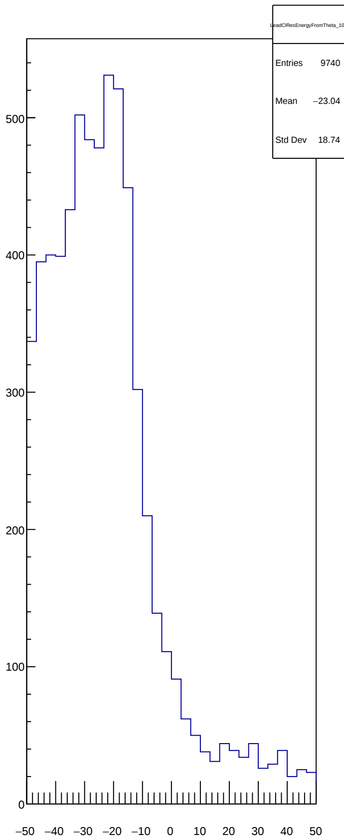
LeadCIResEnergyFromTheta_10
