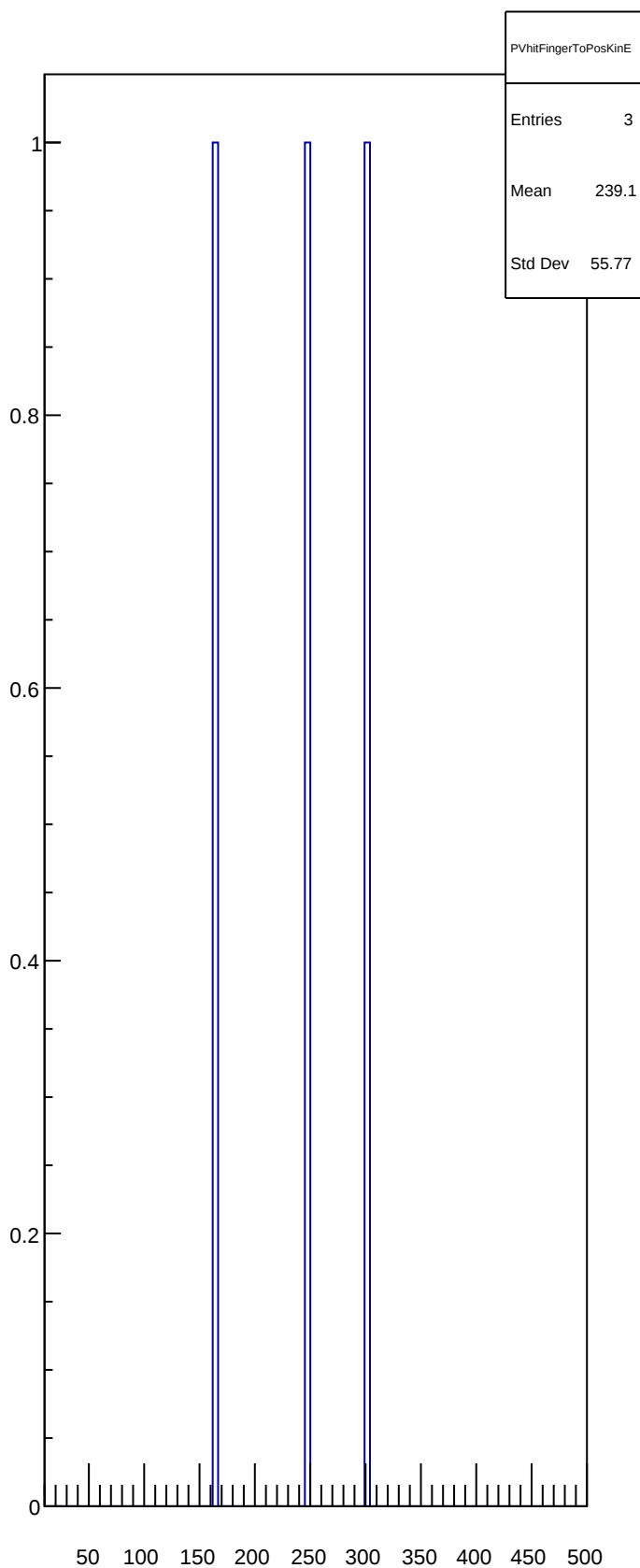
PVhitFingerToPosKinE
