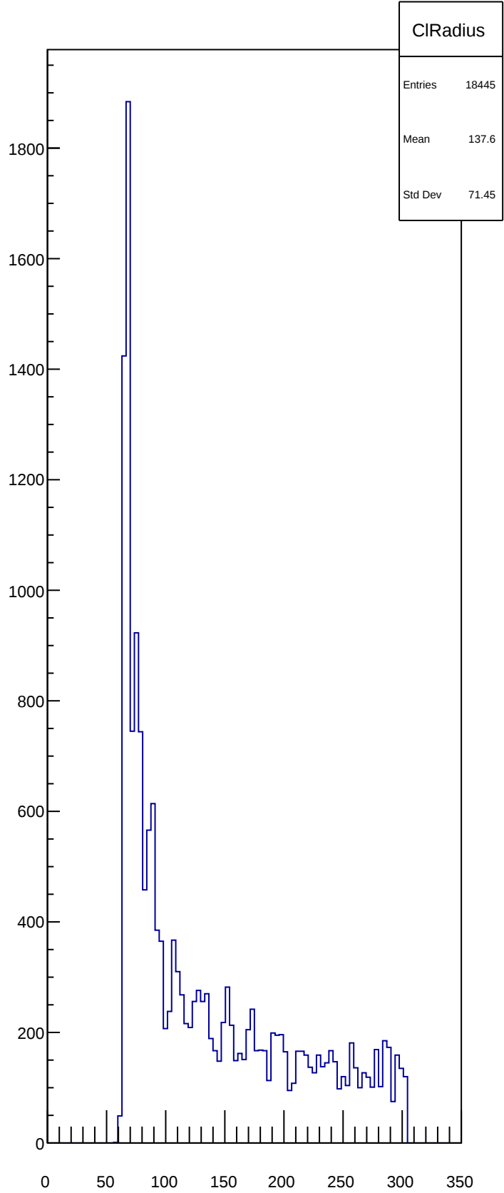
CIRadius
