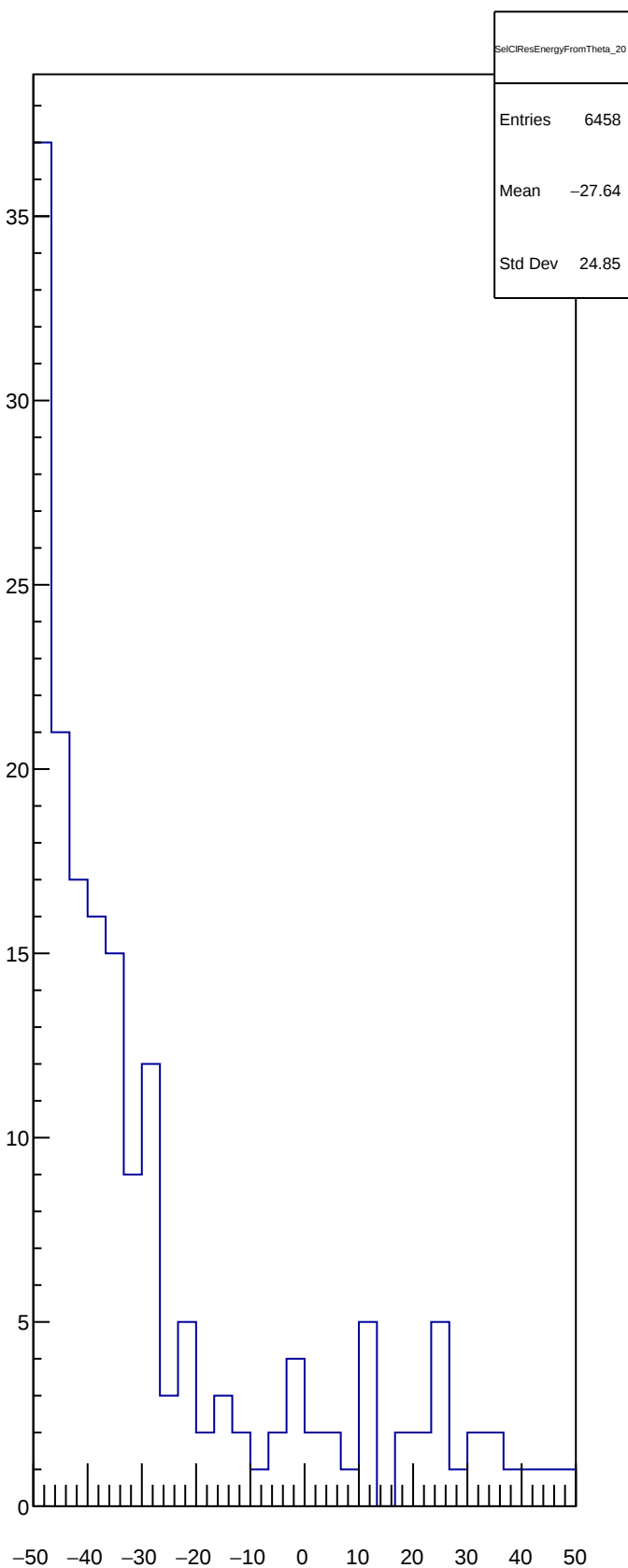
SelClResEnergyFromTheta_20
