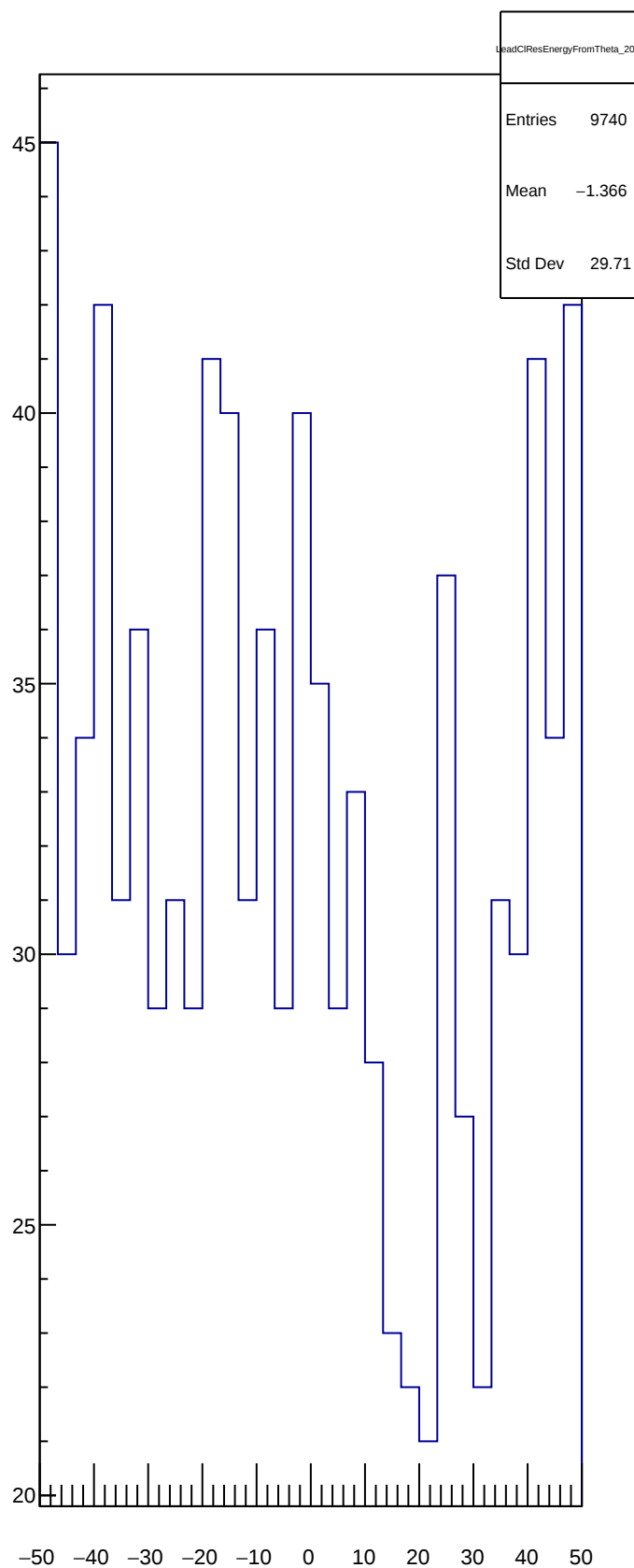
LeadCIResEnergyFromTheta_20
