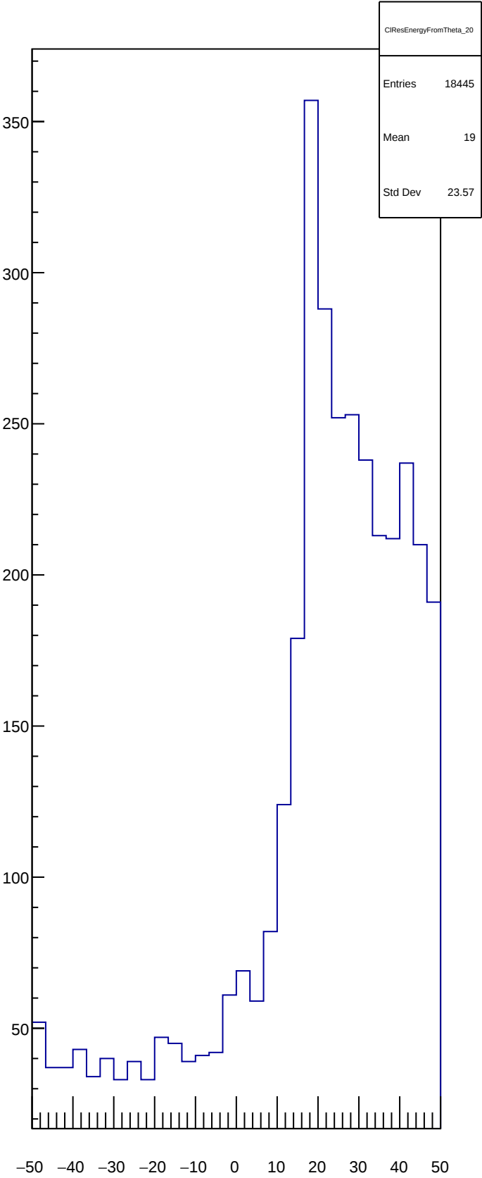
CIResEnergyFromTheta_20
