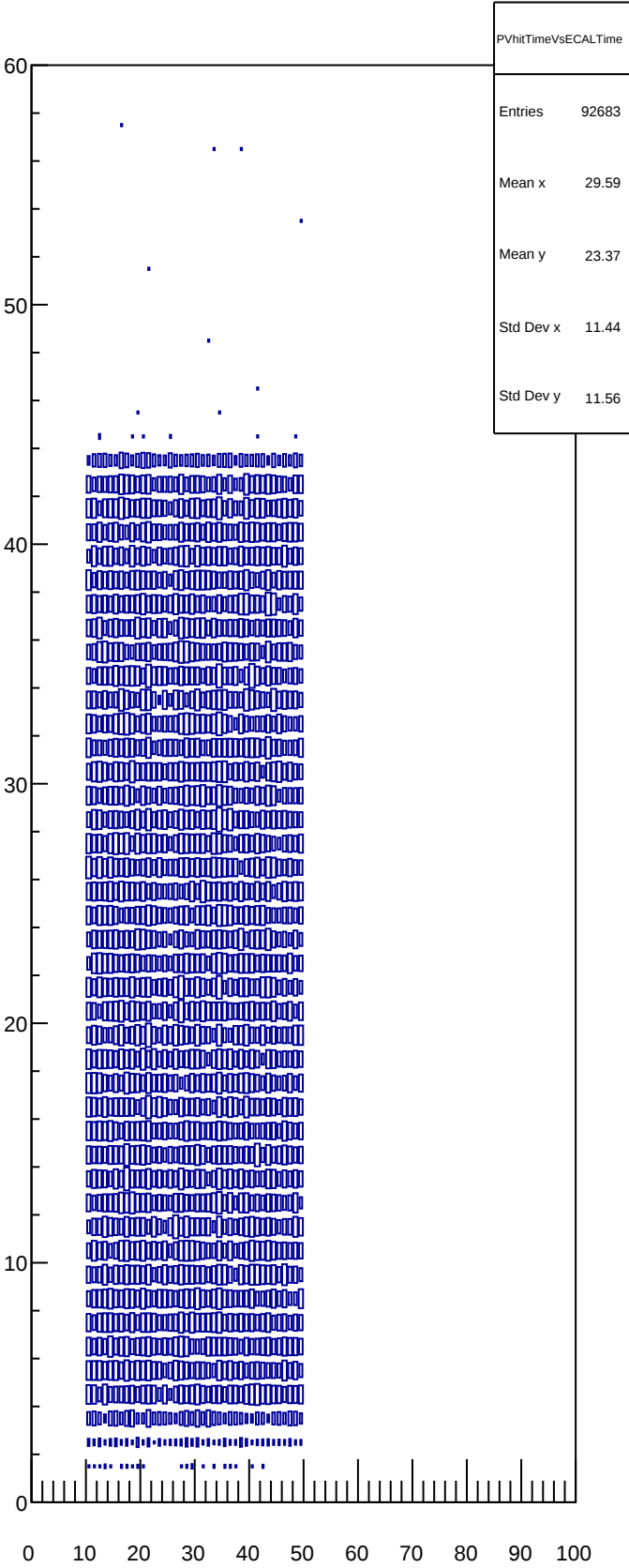
PVhitTimeVsECALTime
