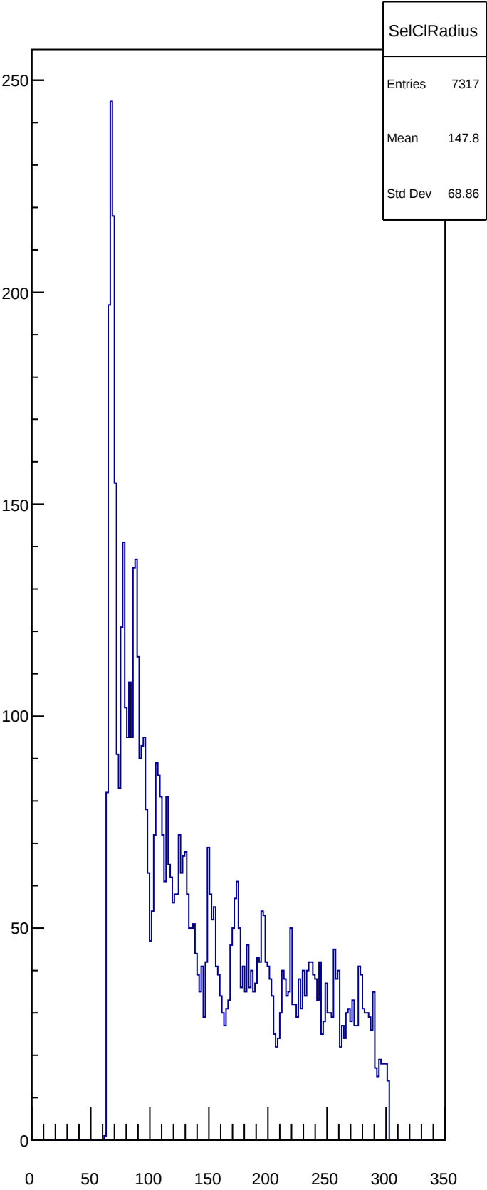
SelCIRadius
