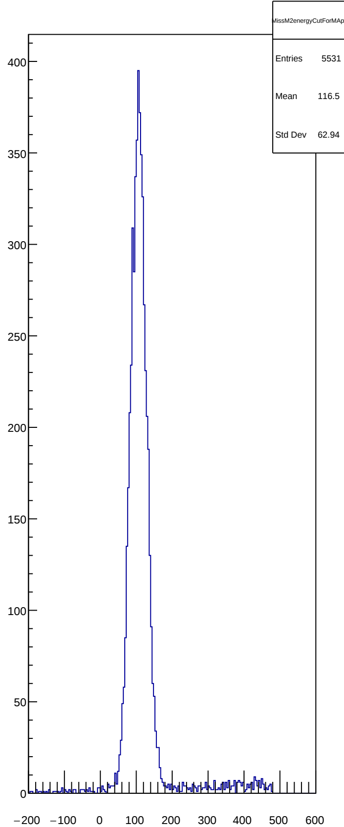
MissM2energyCutForMAp
