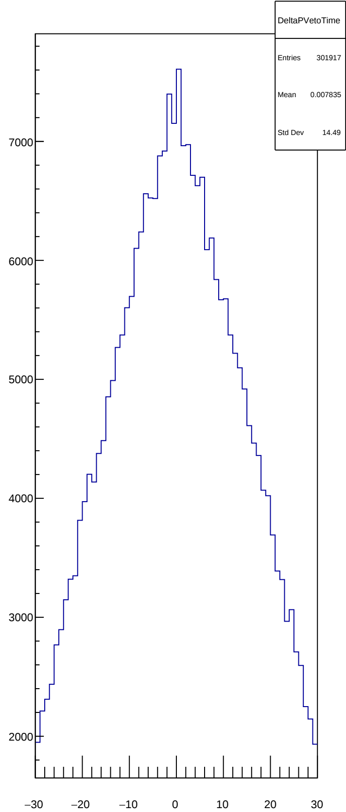
DeltaPVetoTime
