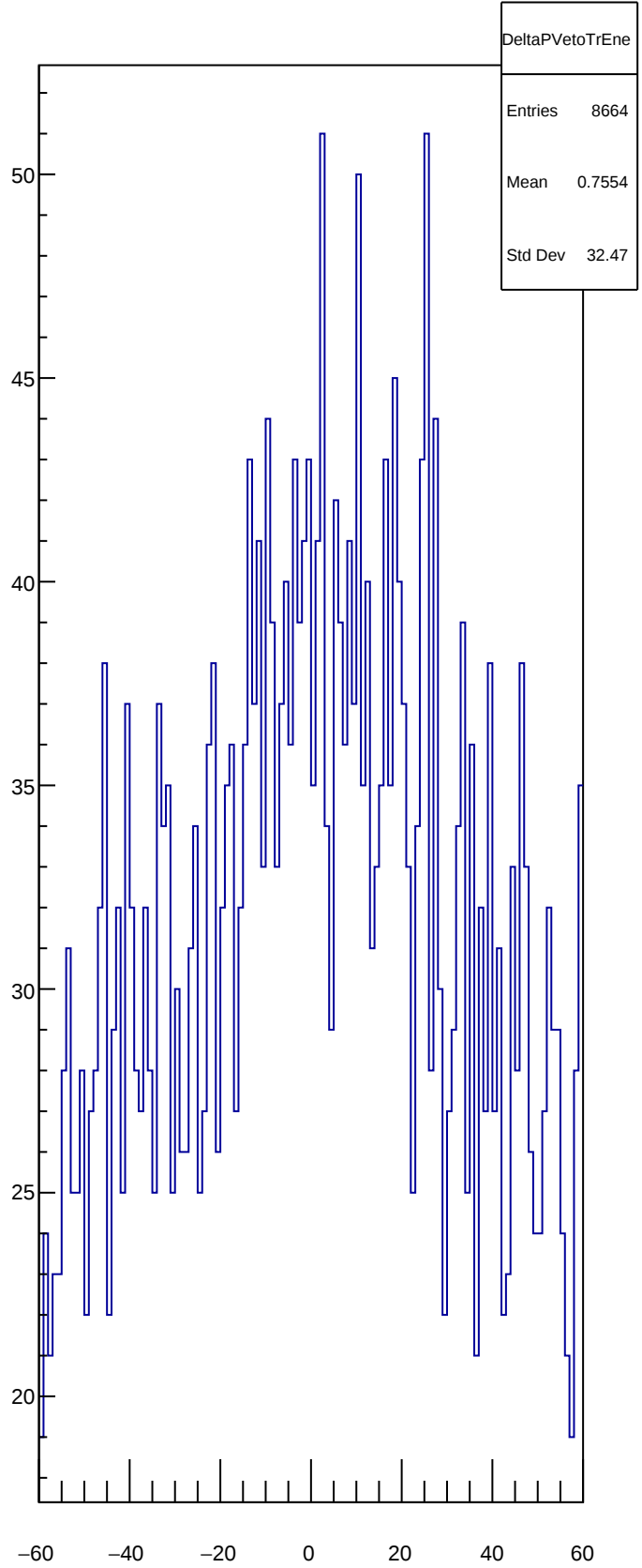
DeltaPVetoTrEne
