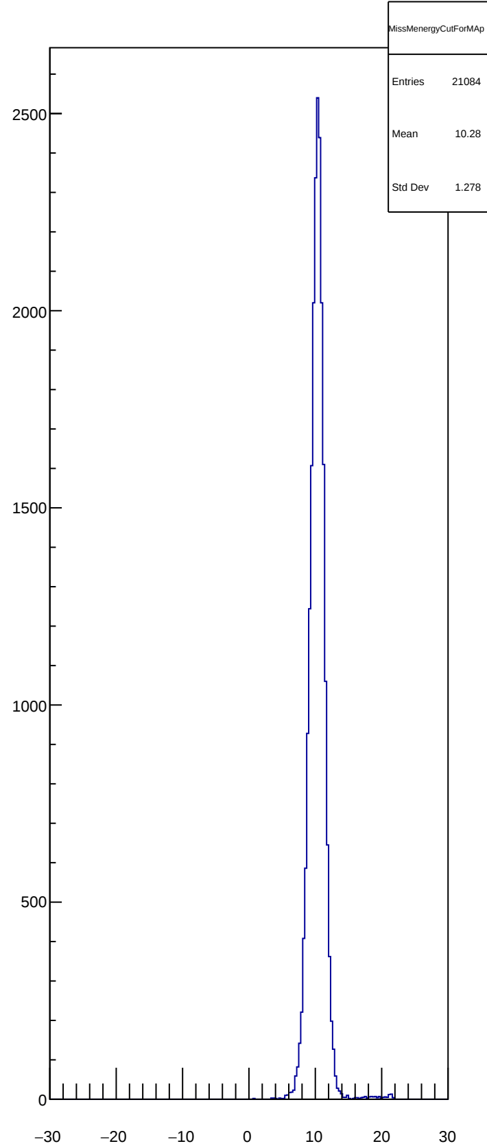
MissMenergyCutForMap
