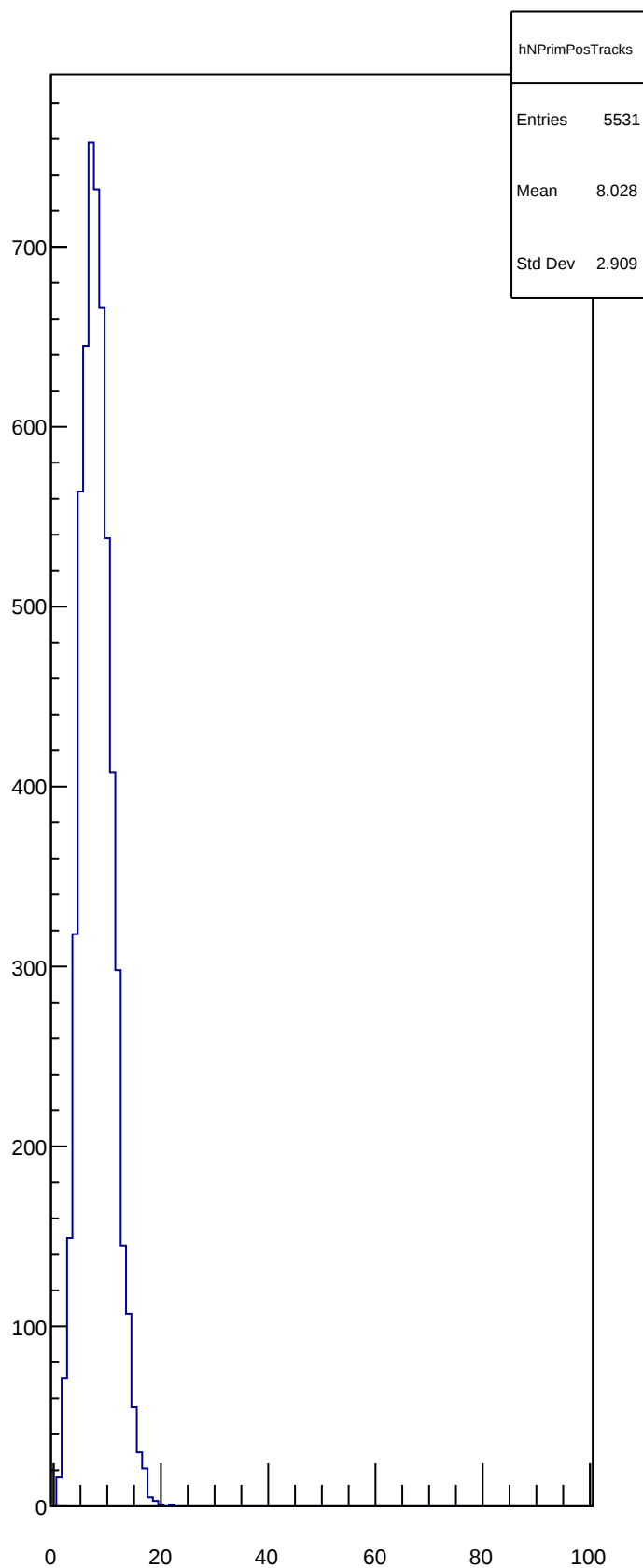
hNPrimPosTracks
