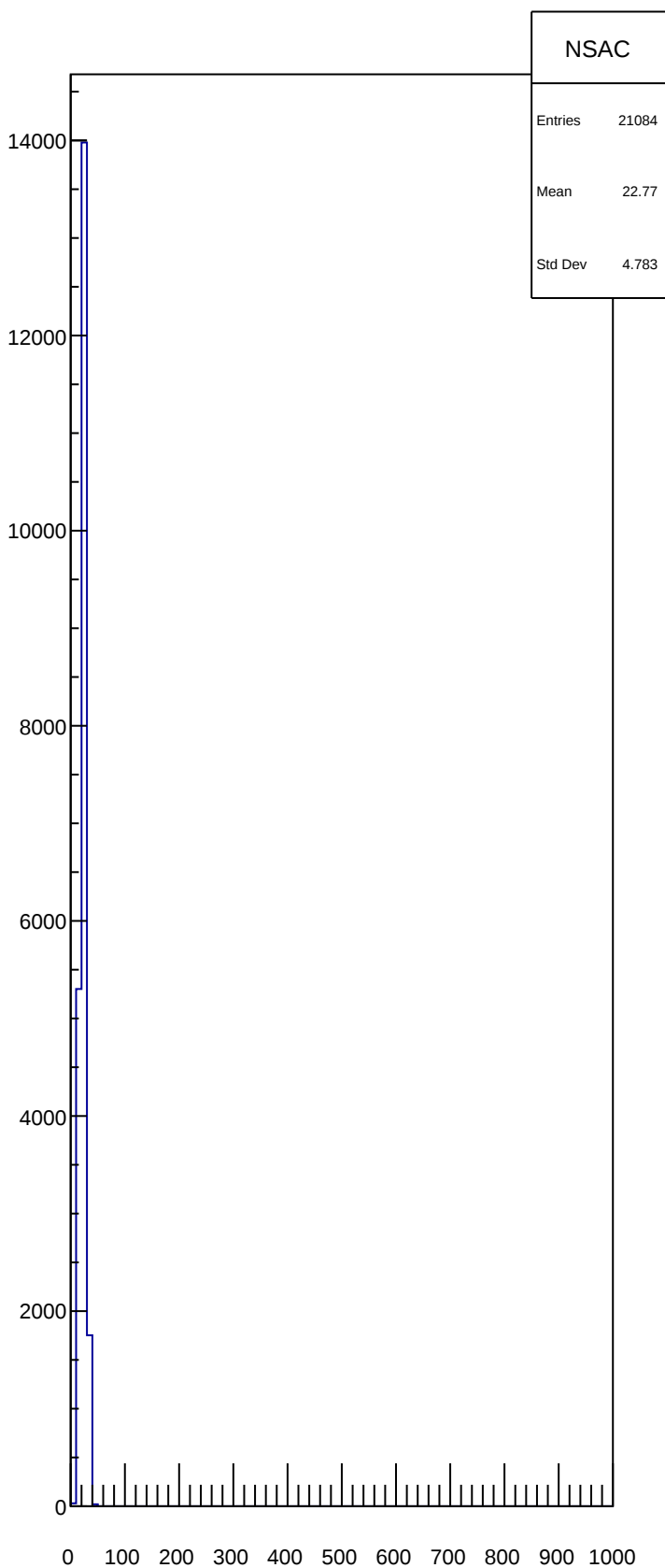
NSAC
