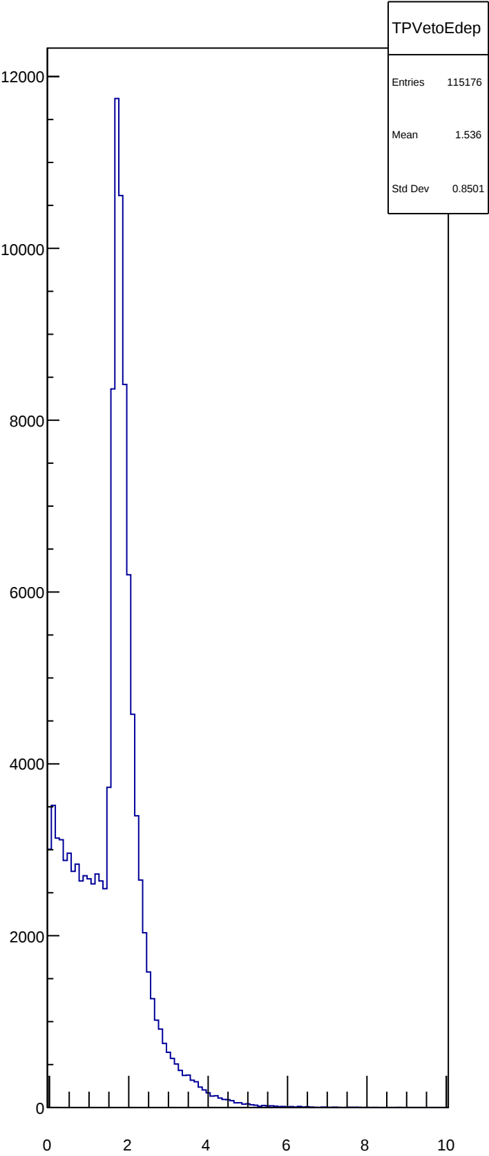
TPVetoEdep
