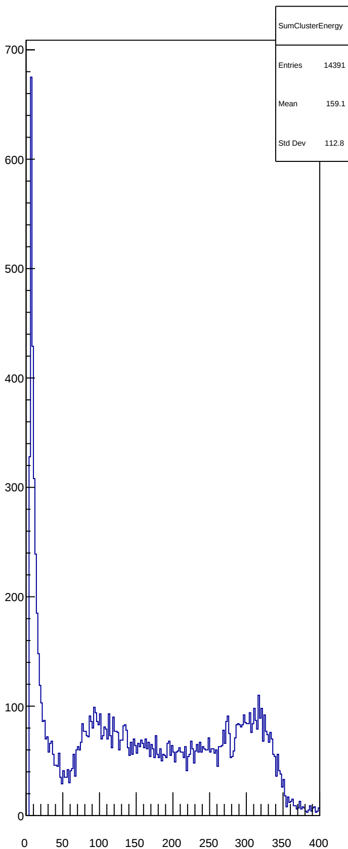
SumClusterEnergy
