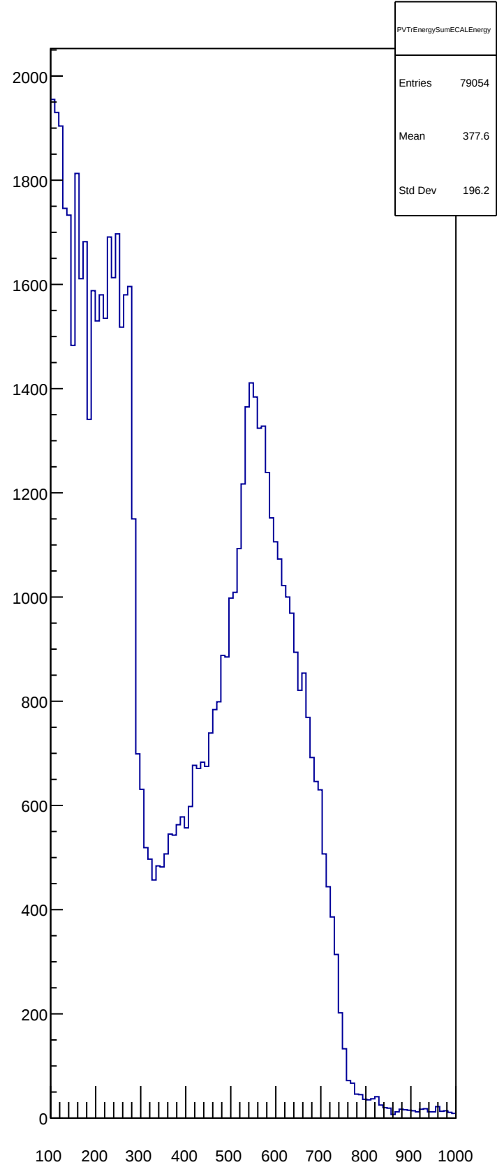
PVTrEnergySumECALEnergy
