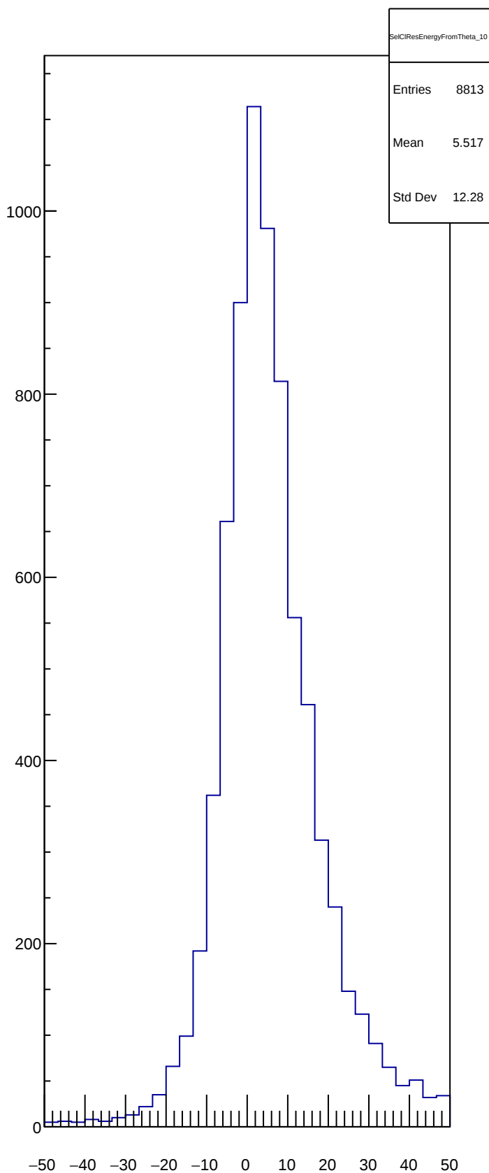
SelClResEnergyFromTheta_10
