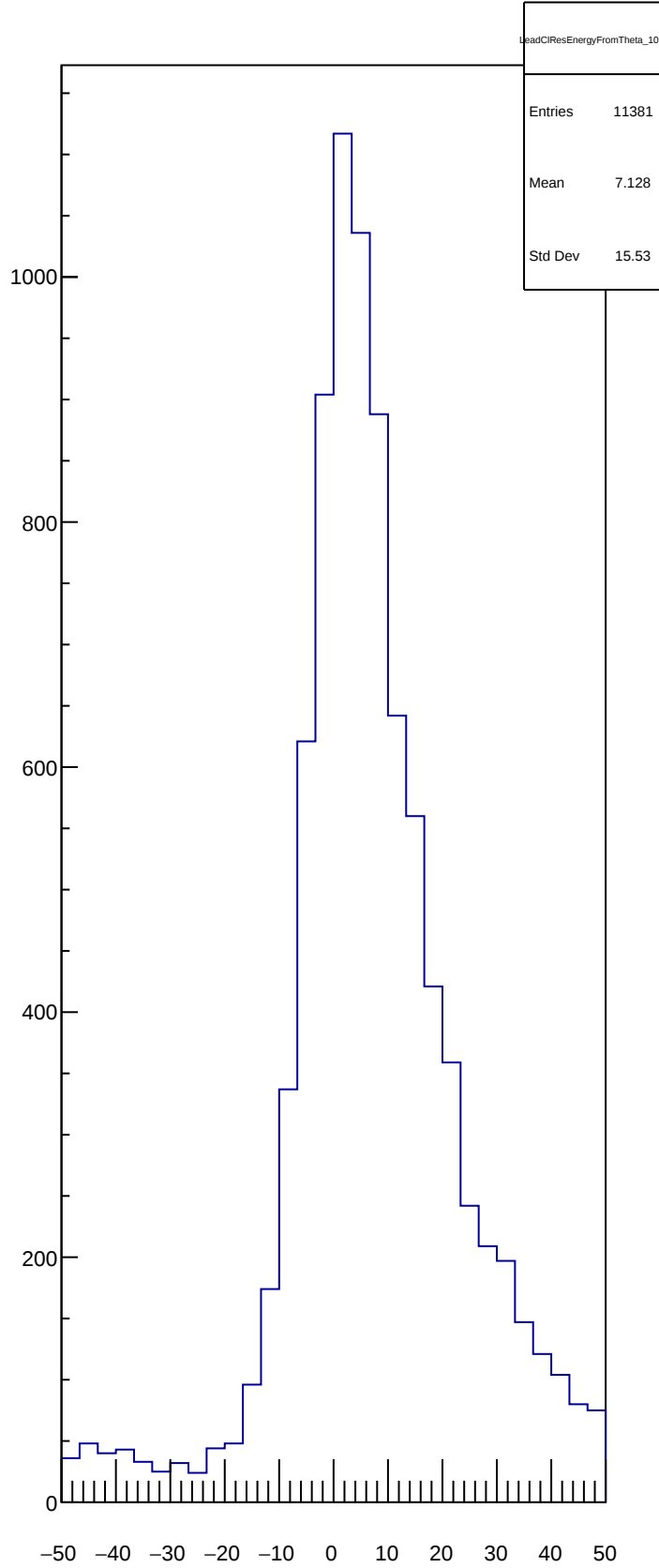
LeadCIResEnergyFromTheta_10
