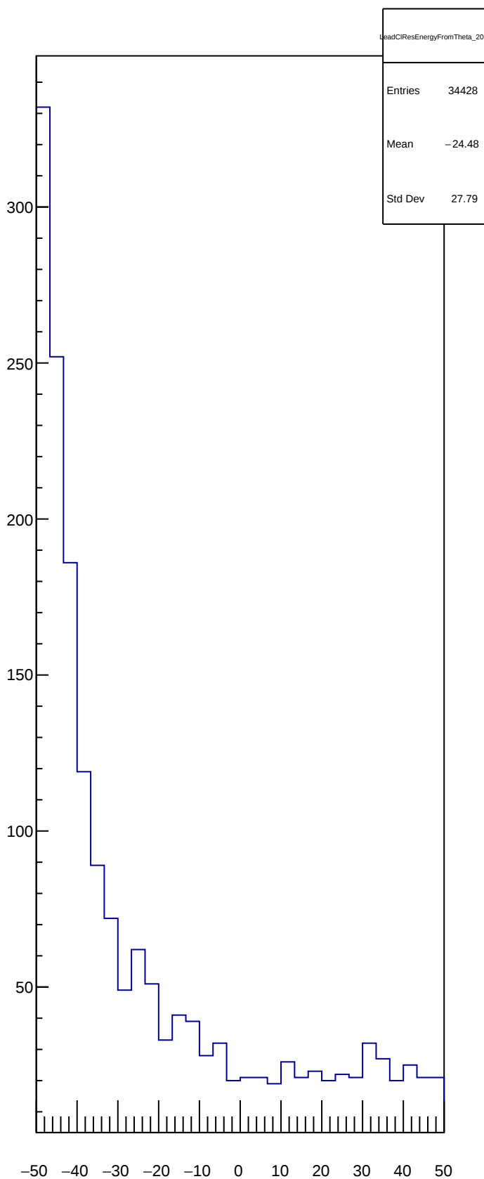
LeadCIResEnergyFromTheta_20
