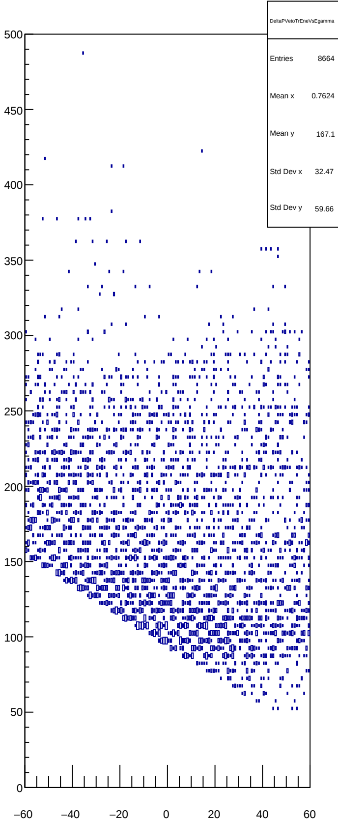
DeltaPVetoTrEneVsEgamma
