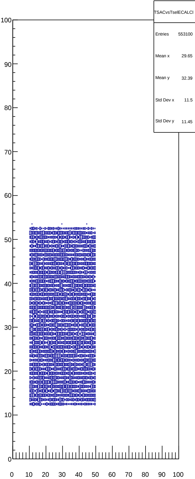
TSACvsTselECALCI
