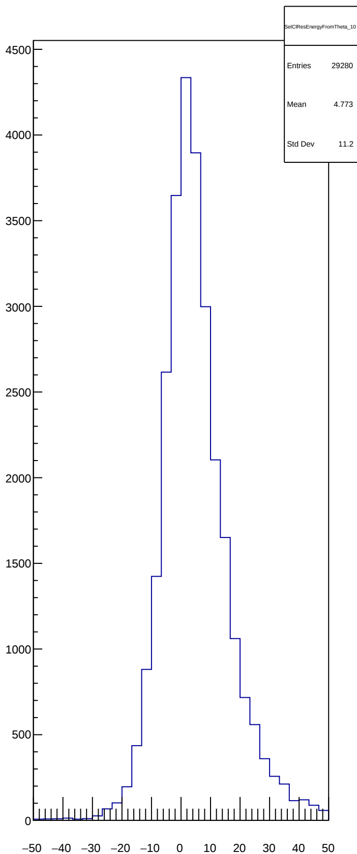
SelClResEnergyFromTheta_10
