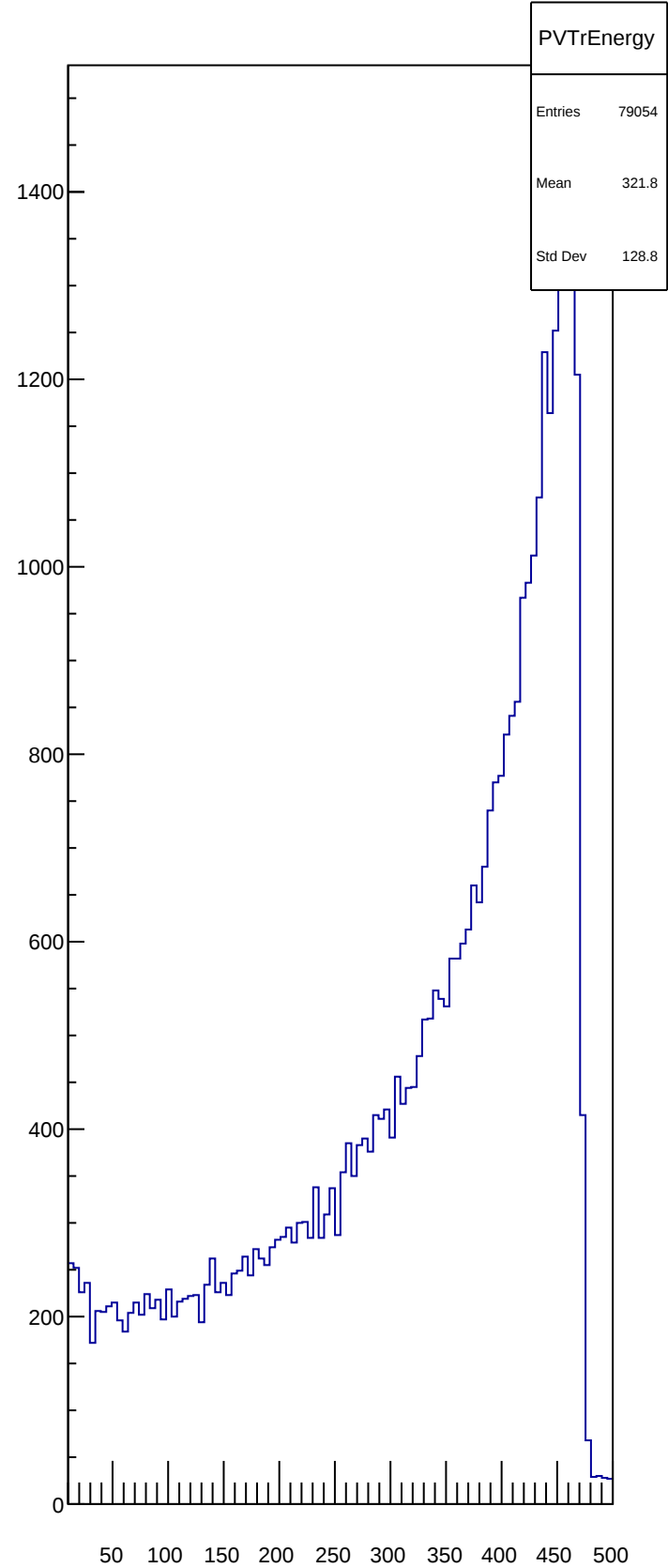
PVTrEnergy
