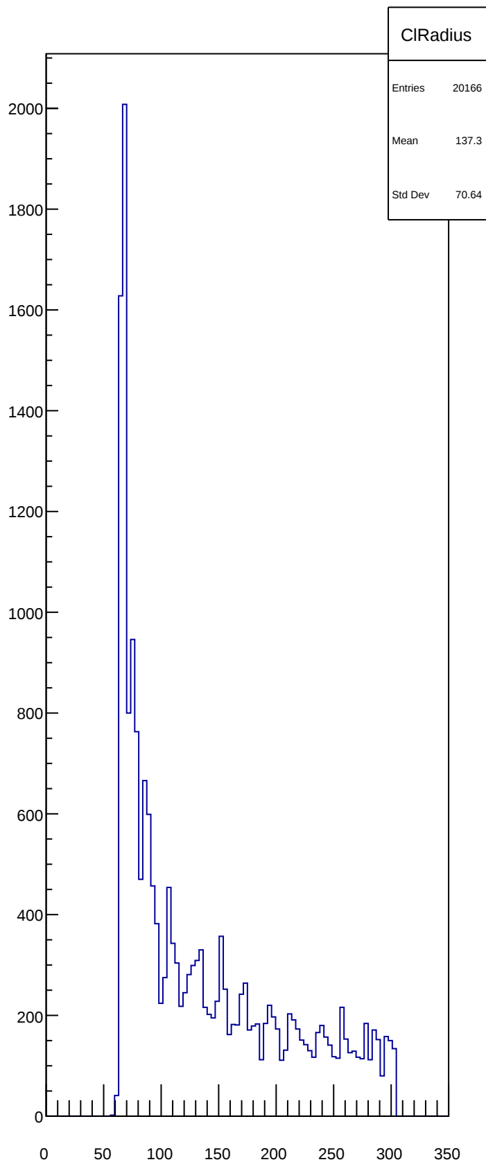
CIRadius
