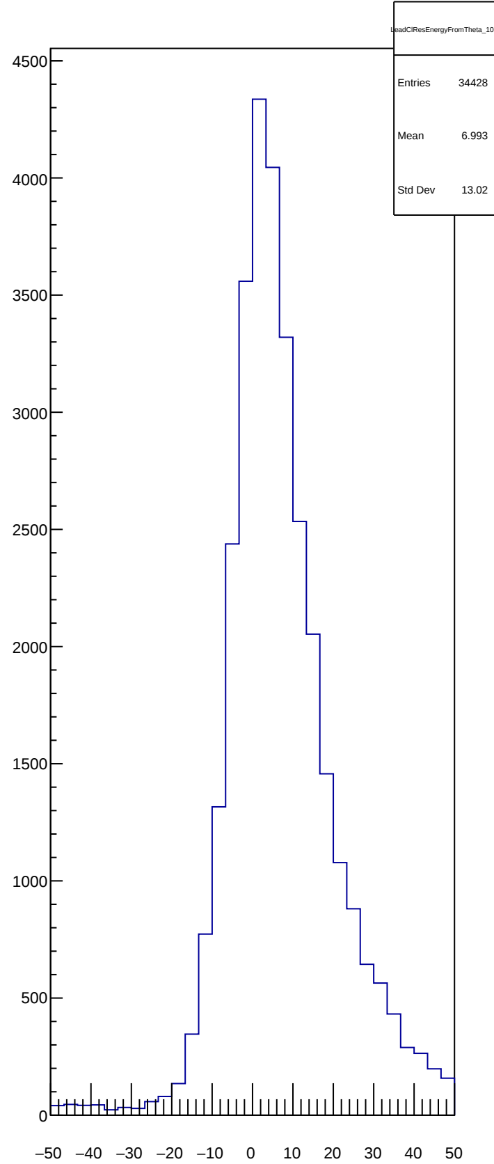
LeadCIResEnergyFromTheta_10
