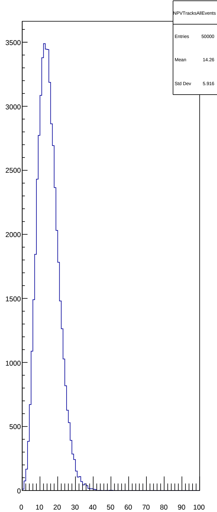
NPVTracksAllEvents
