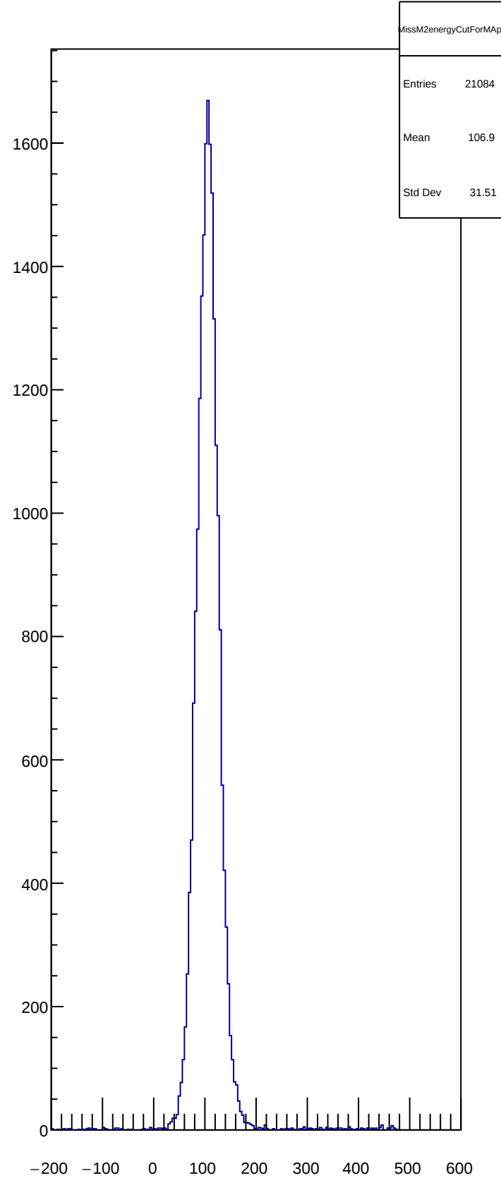
MissM2energyCutForMAp
