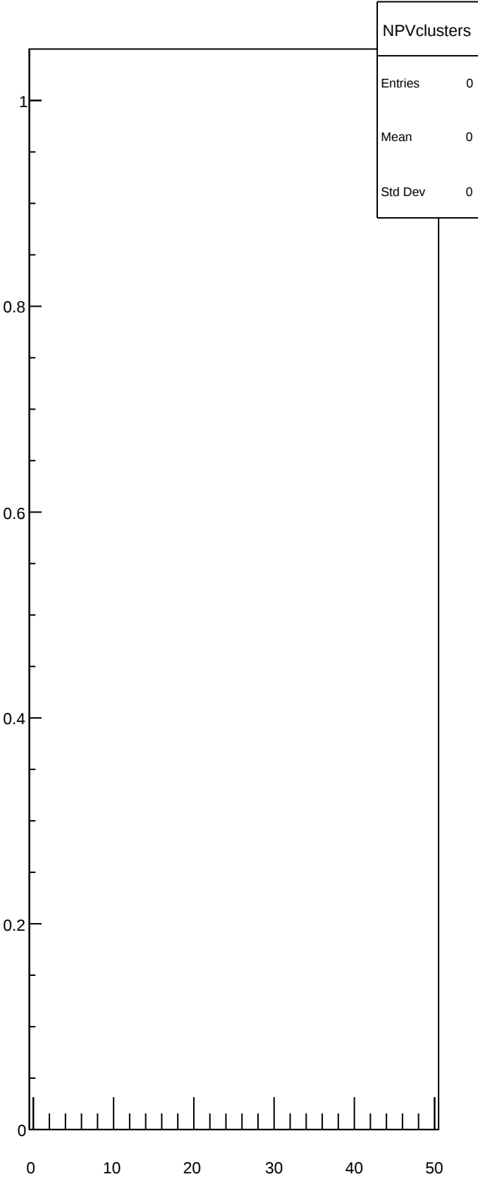
NPVclusters
