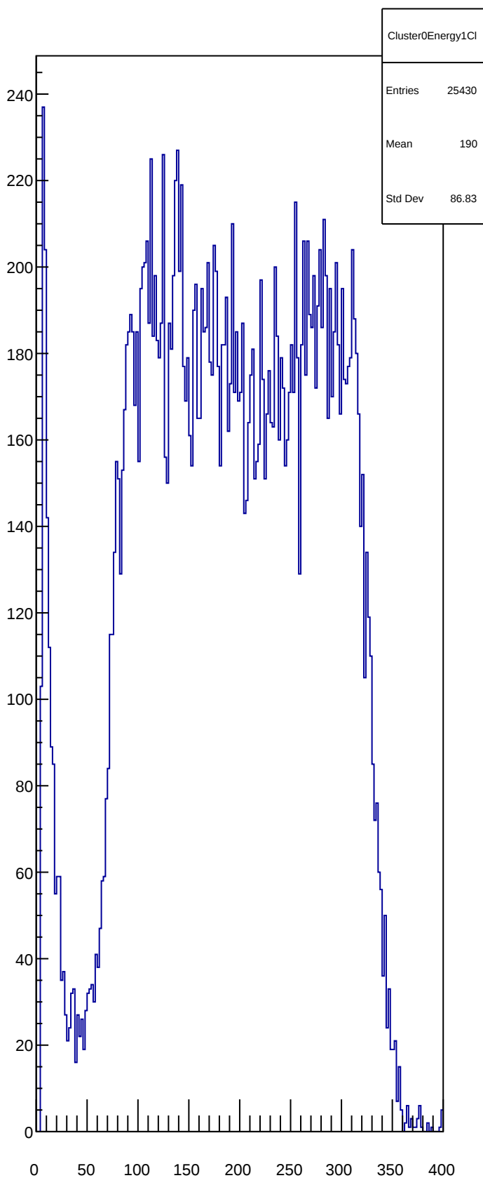
Cluster0Energy1CI
