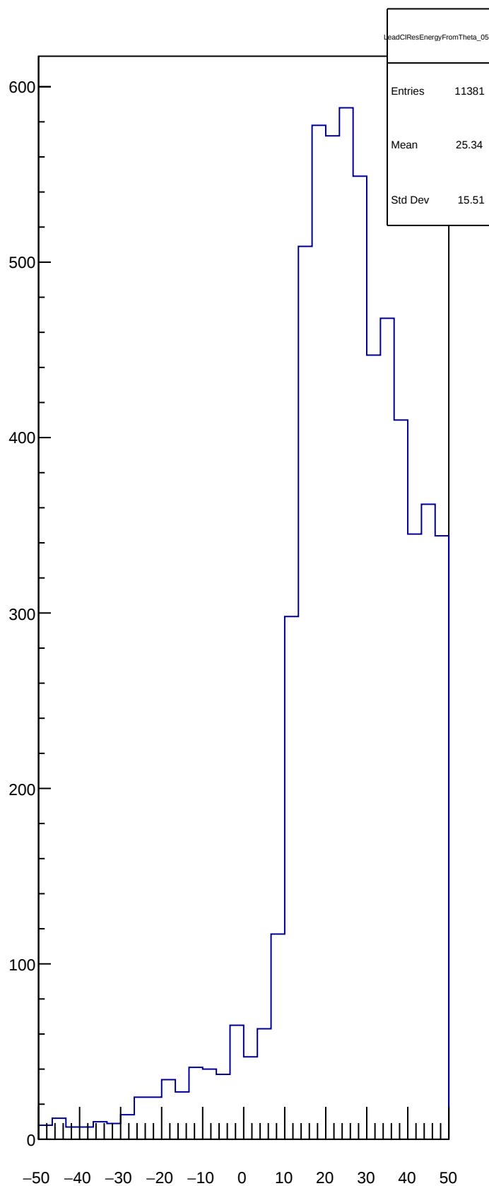
LeadCIResEnergyFromTheta_05
