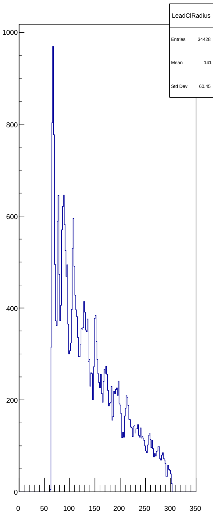
LeadCIRadius
