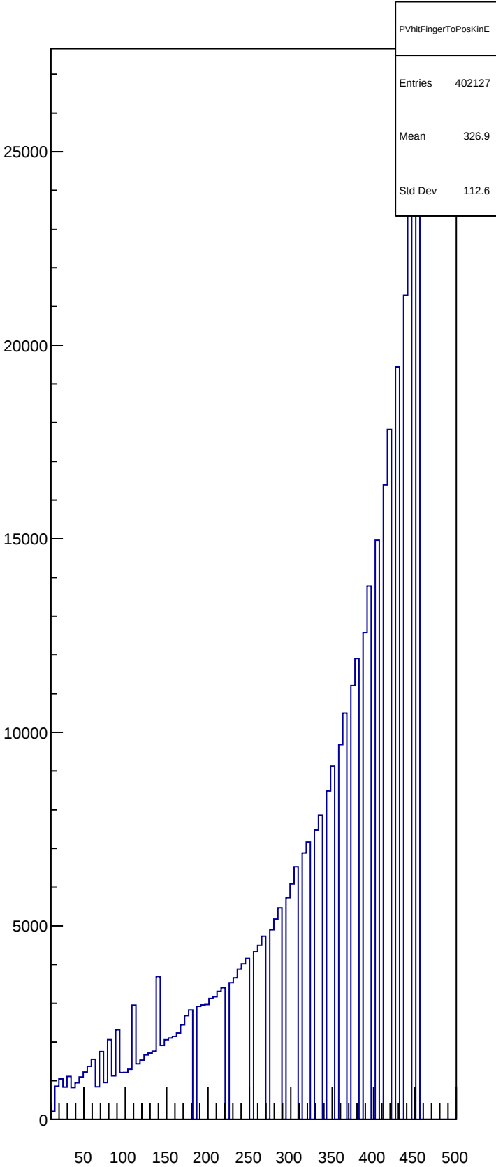
PVhitFingerToPosKinE
