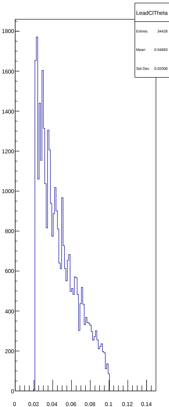
LeadCITheta
