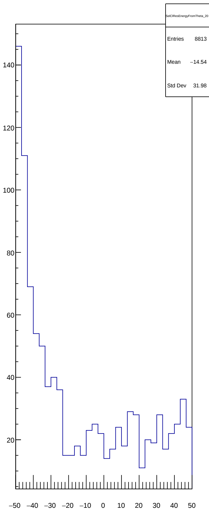
SelClResEnergyFromTheta_20
