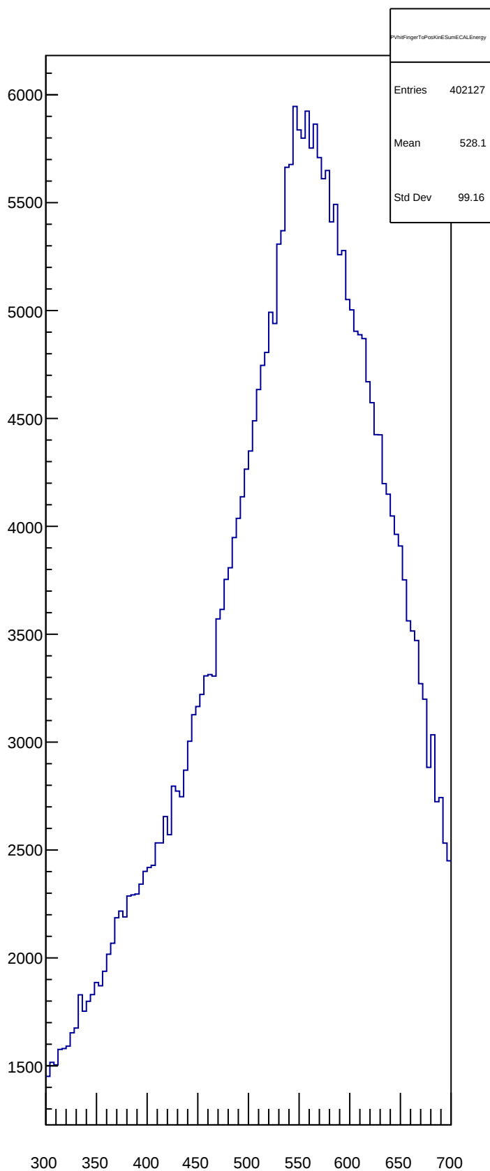
PVhitFingerToPosKinESumECALEnergy
