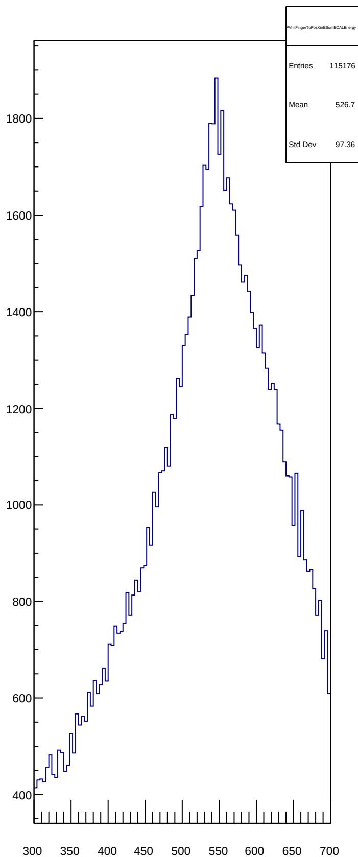
PVhitFingerToPosKinESumECALEnergy
