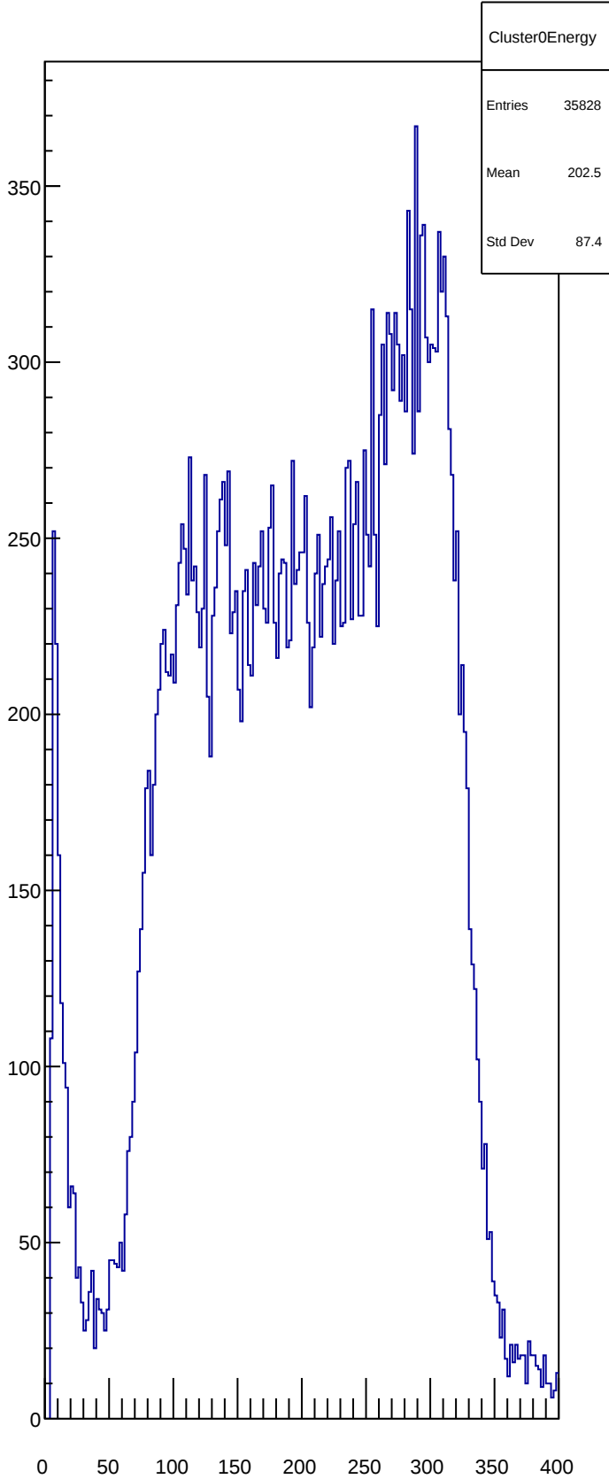
Cluster0Energy
