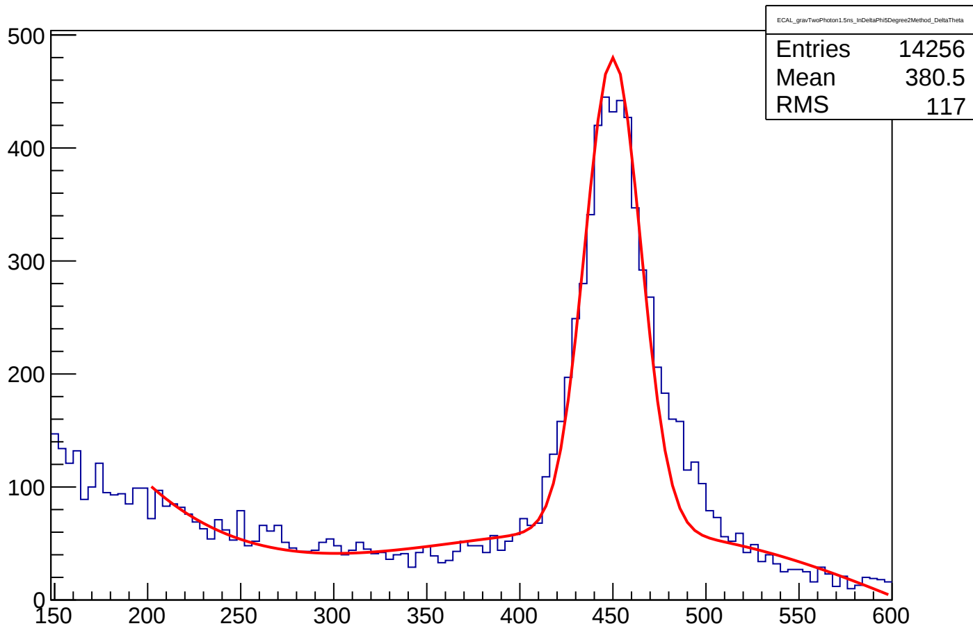
ECAL_gravTwoPhoton1.5ns_InDeltaPhi5Degree2Method_DeltaTheta
