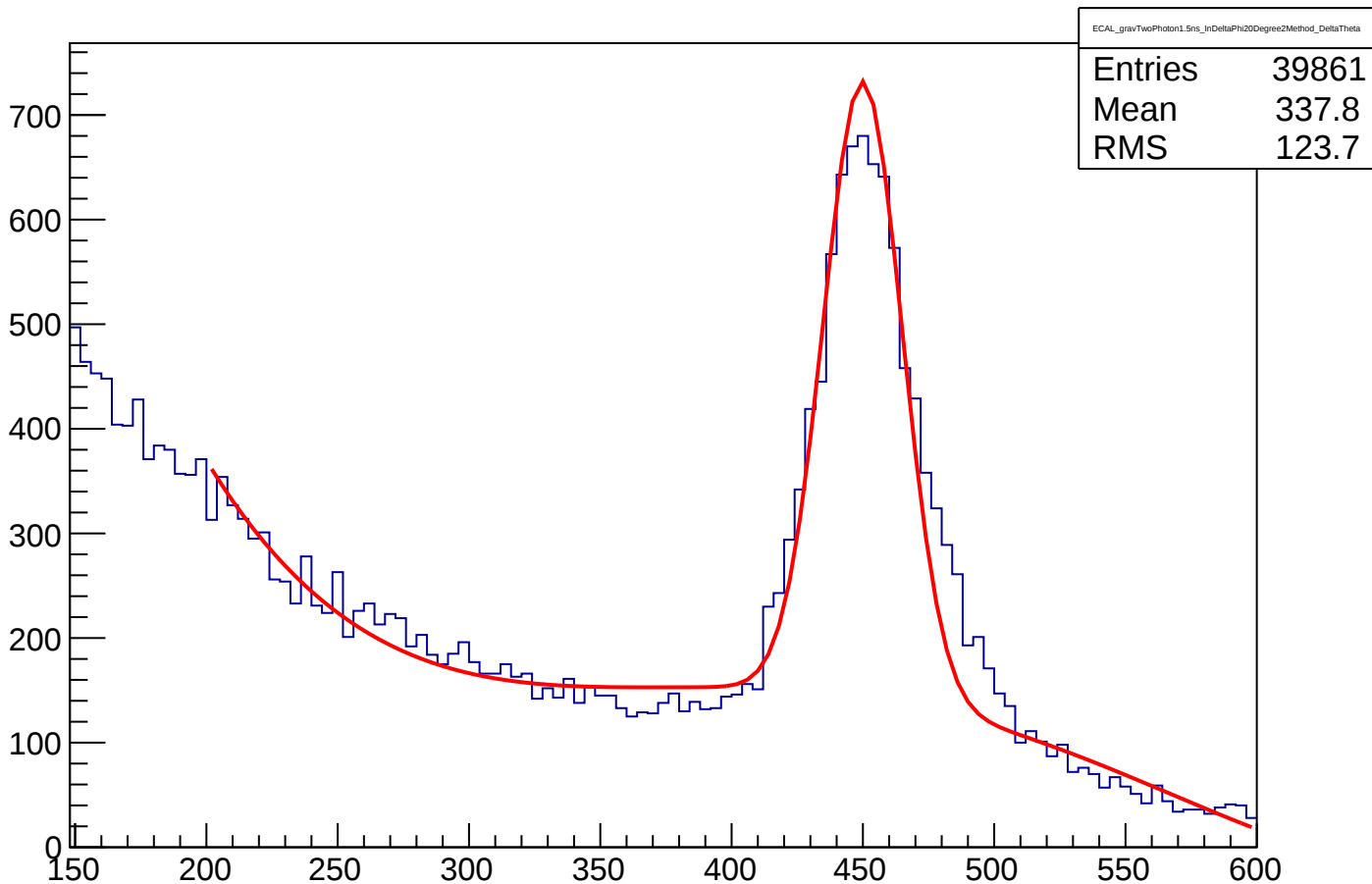
ECAL_gravTwoPhoton1.5ns_InDeltaPhi20Degree2Method_DeltaTheta
