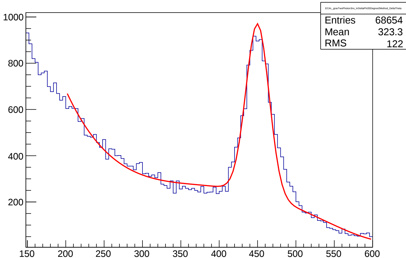
ECAL_gravTwoPhoton3ns_InDeltaPhi20Degree2Method_DeltaTheta
