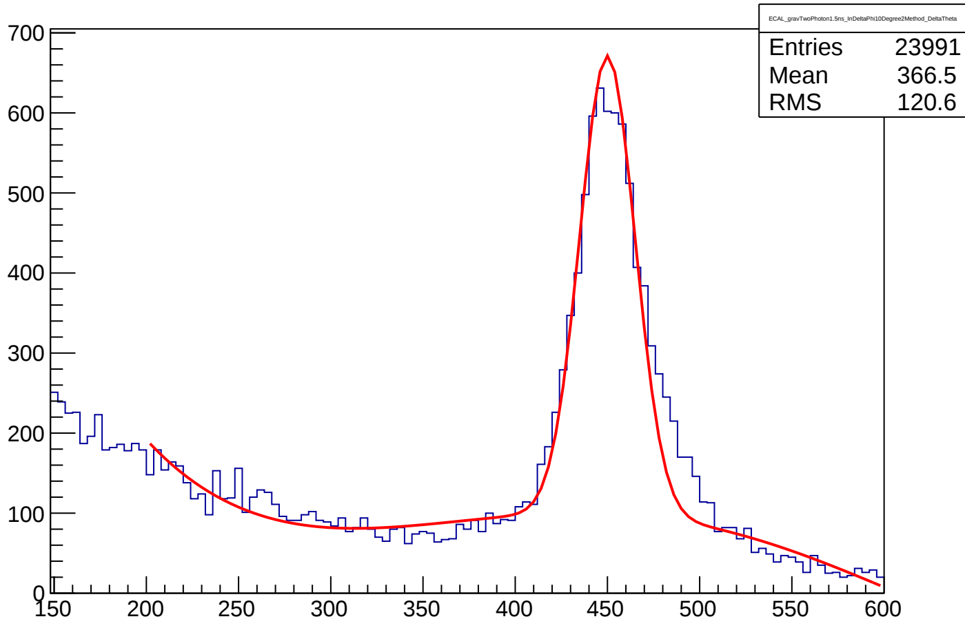
ECAL_gravTwoPhoton1.5ns_InDeltaPhi10Degree2Method_DeltaTheta
