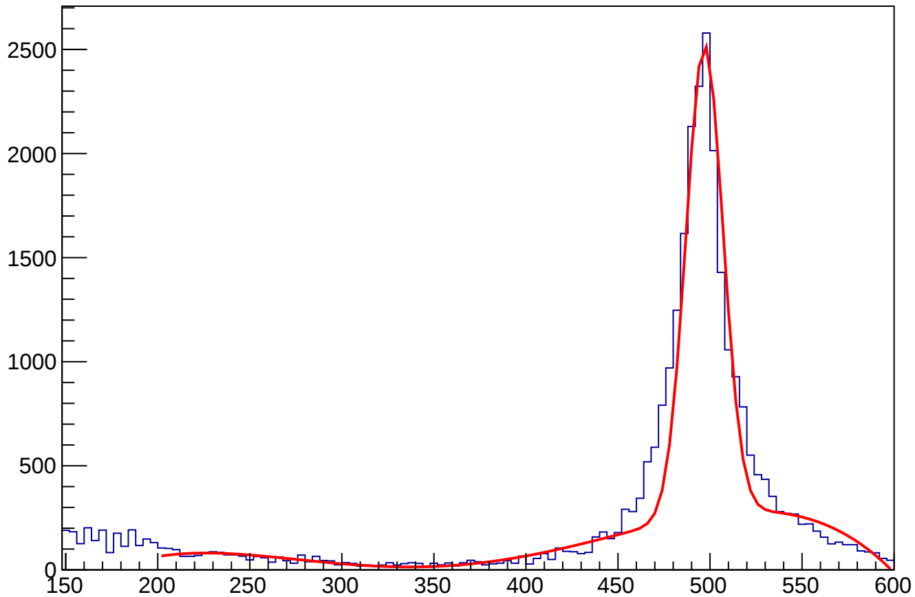
ECAL_gravTwoPhoton1.5ns3cm_InDeltaPhi_withAngleCut
