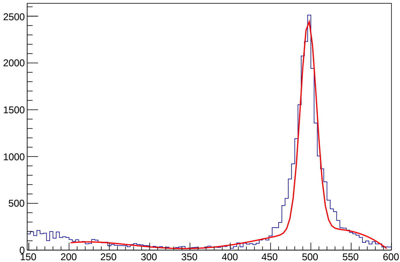
ECAL_gravTwoPhoton3ns2cm_InDeltaPhi_withAngleCut
