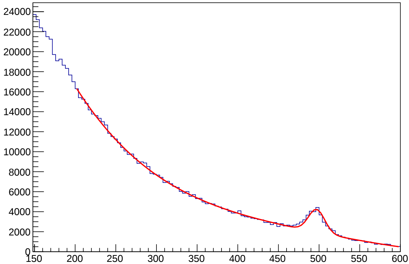
ECAL_twoPhotonInTime1.5ns
