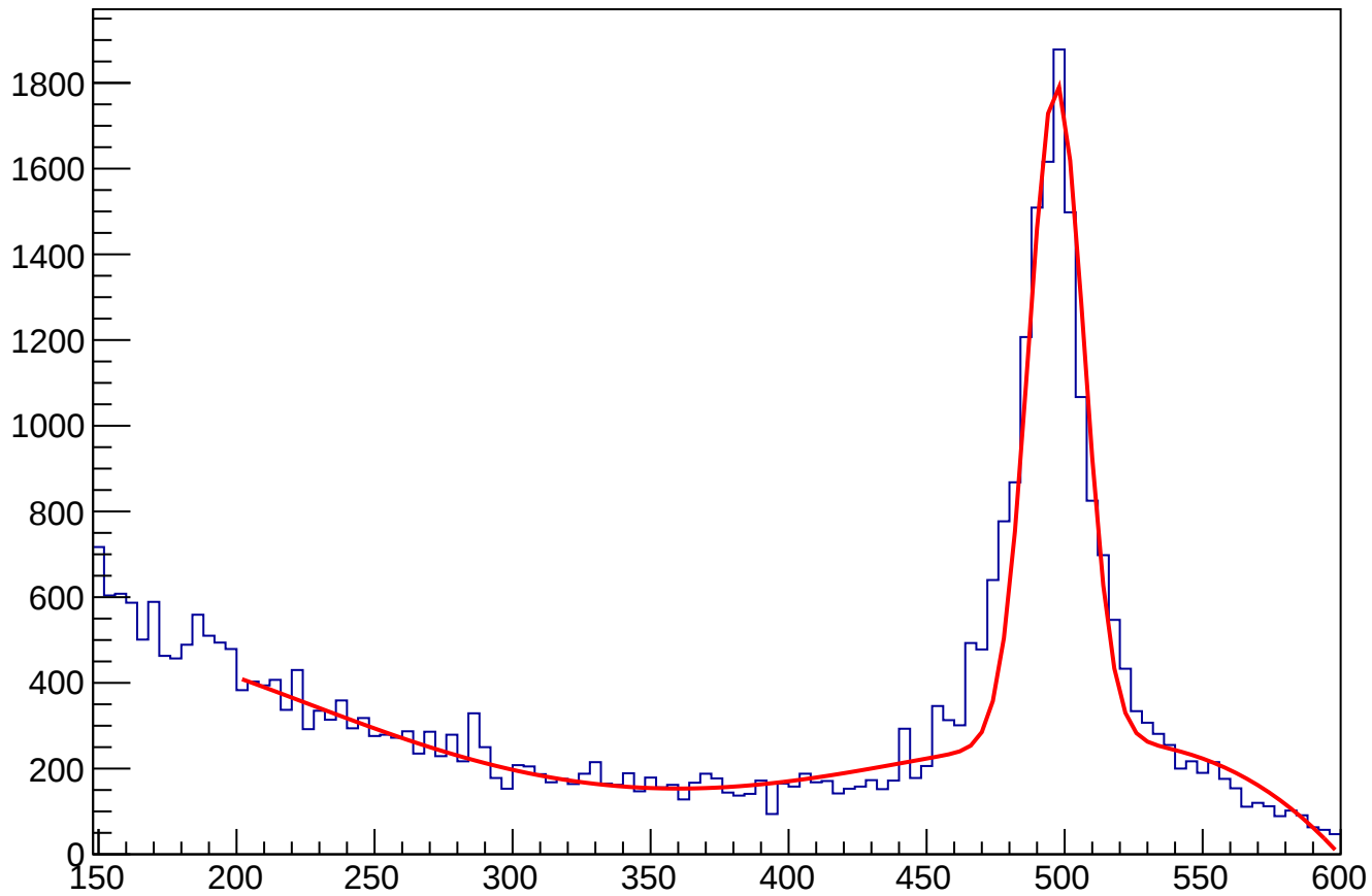
ECAL_gravTwoPhoton1.5ns_InDeltaPhi5Degree2Method
