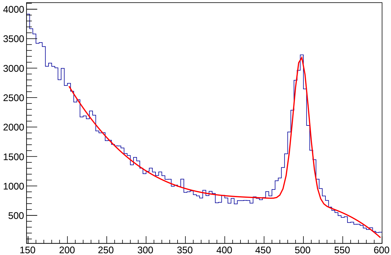
ECAL_gravTwoPhoton3ns_InDeltaPhi20Degree2Method
