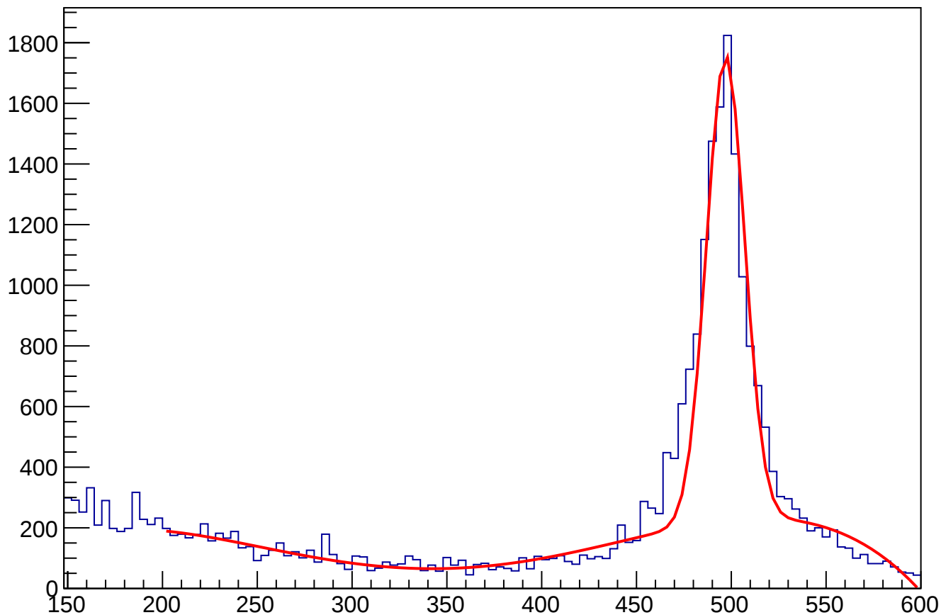
ECAL_gravTwoPhoton1.5ns_InDeltaPhi5Degree2Method_DeltaTheta
