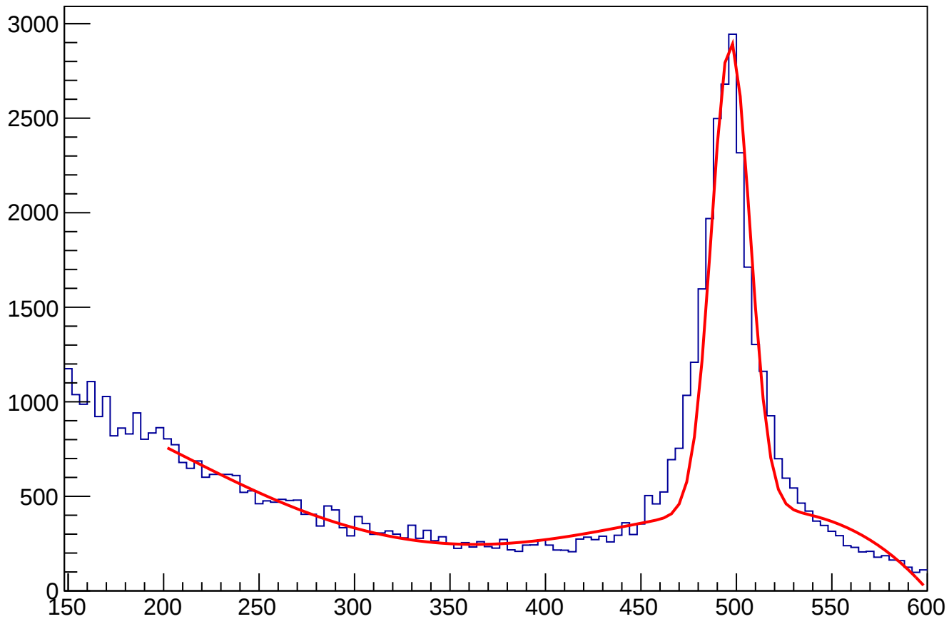
ECAL_gravTwoPhoton1.5ns_InDeltaPhi20Degree2Method_DeltaTheta
