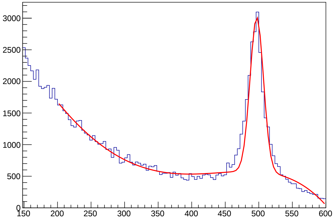
ECAL_gravTwoPhoton1.5ns_InDeltaPhi20Degree2Method
