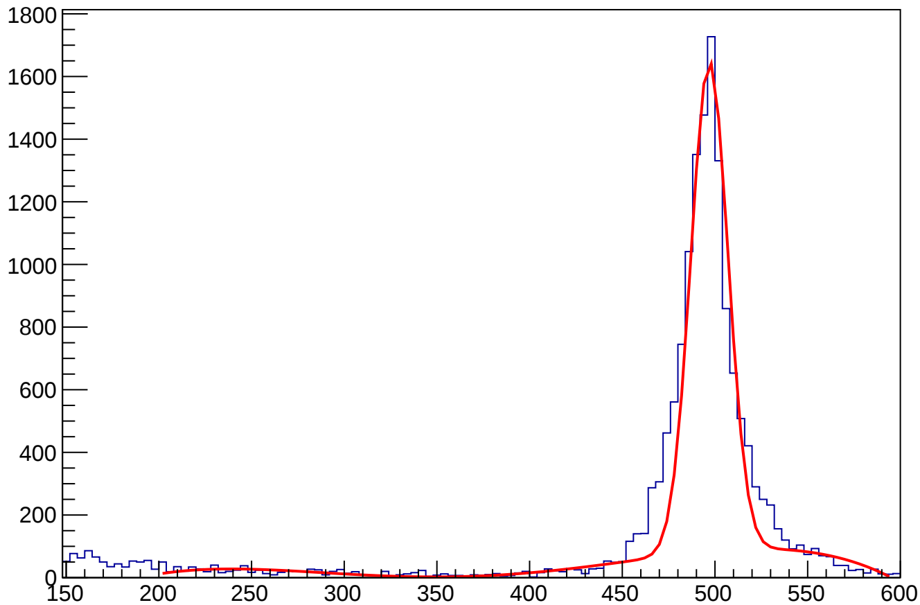
ECAL_gravTwoPhoton3ns1cm_InDeltaPhi_withAngleCut
