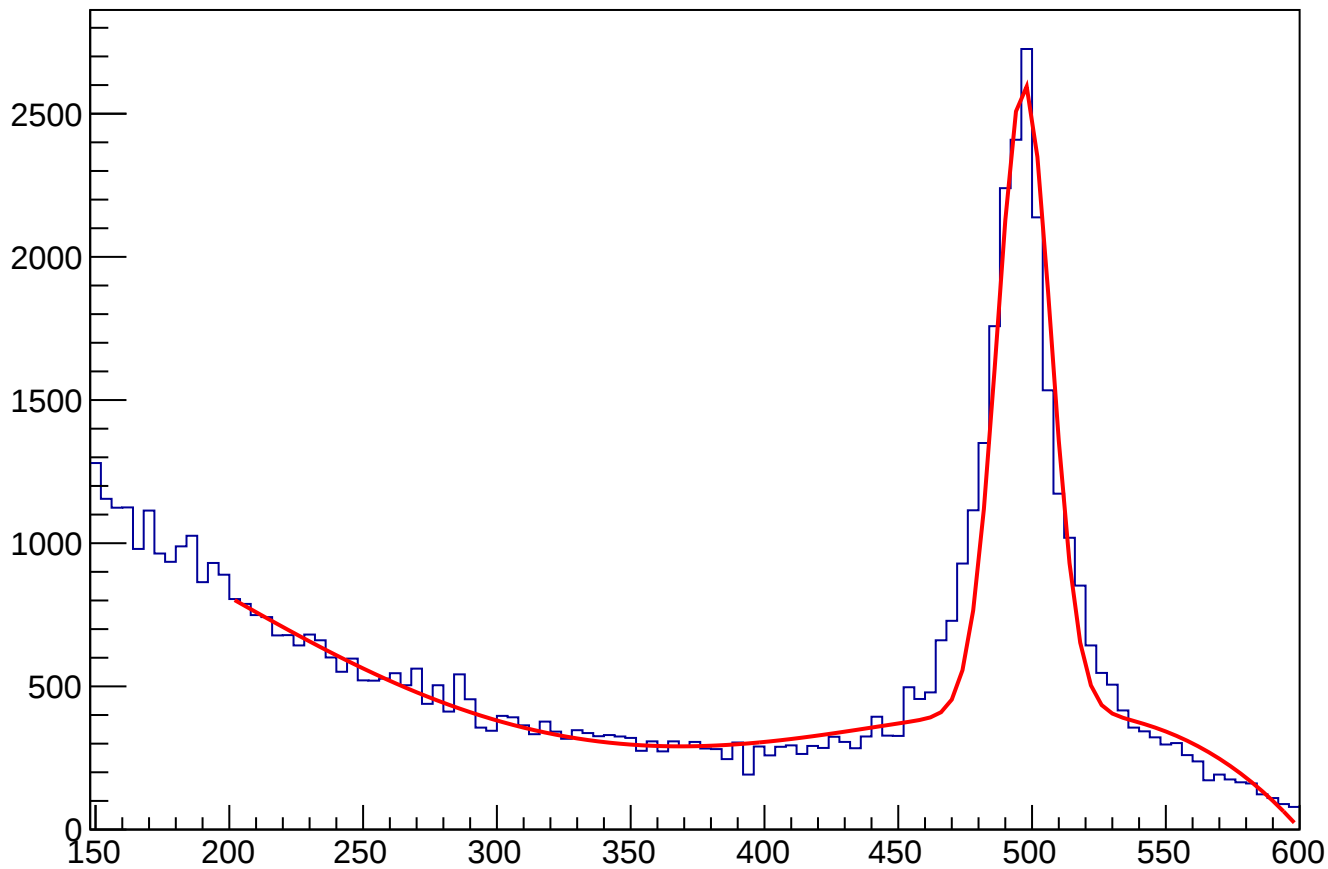
ECAL_gravTwoPhoton1.5ns_InDeltaPhi10Degree2Method
