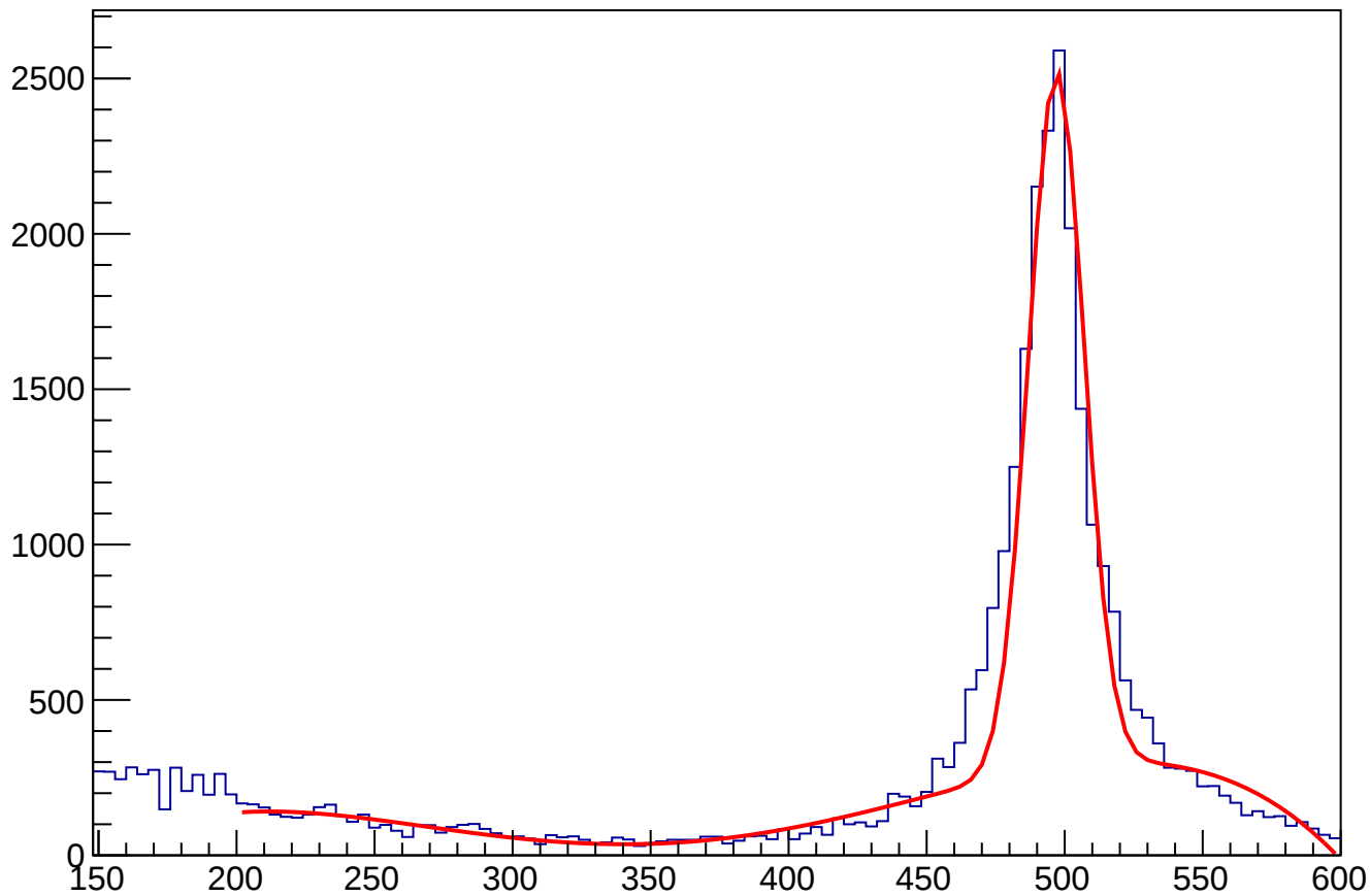
ECAL_gravTwoPhoton3ns3cm_InDeltaPhi_withAngleCut
