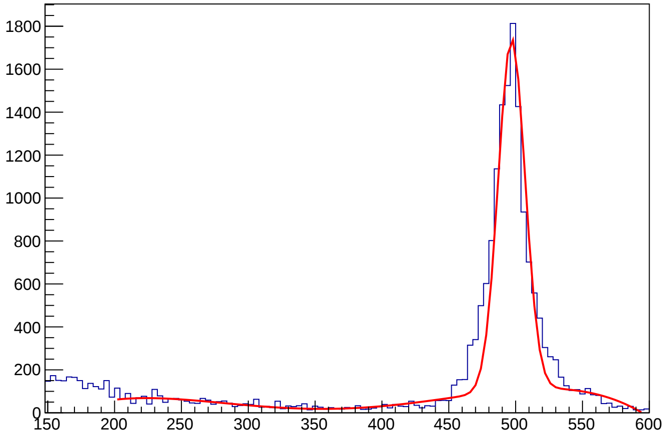
ECAL_gravTwoPhoton3ns1cm_InDeltaPhi
