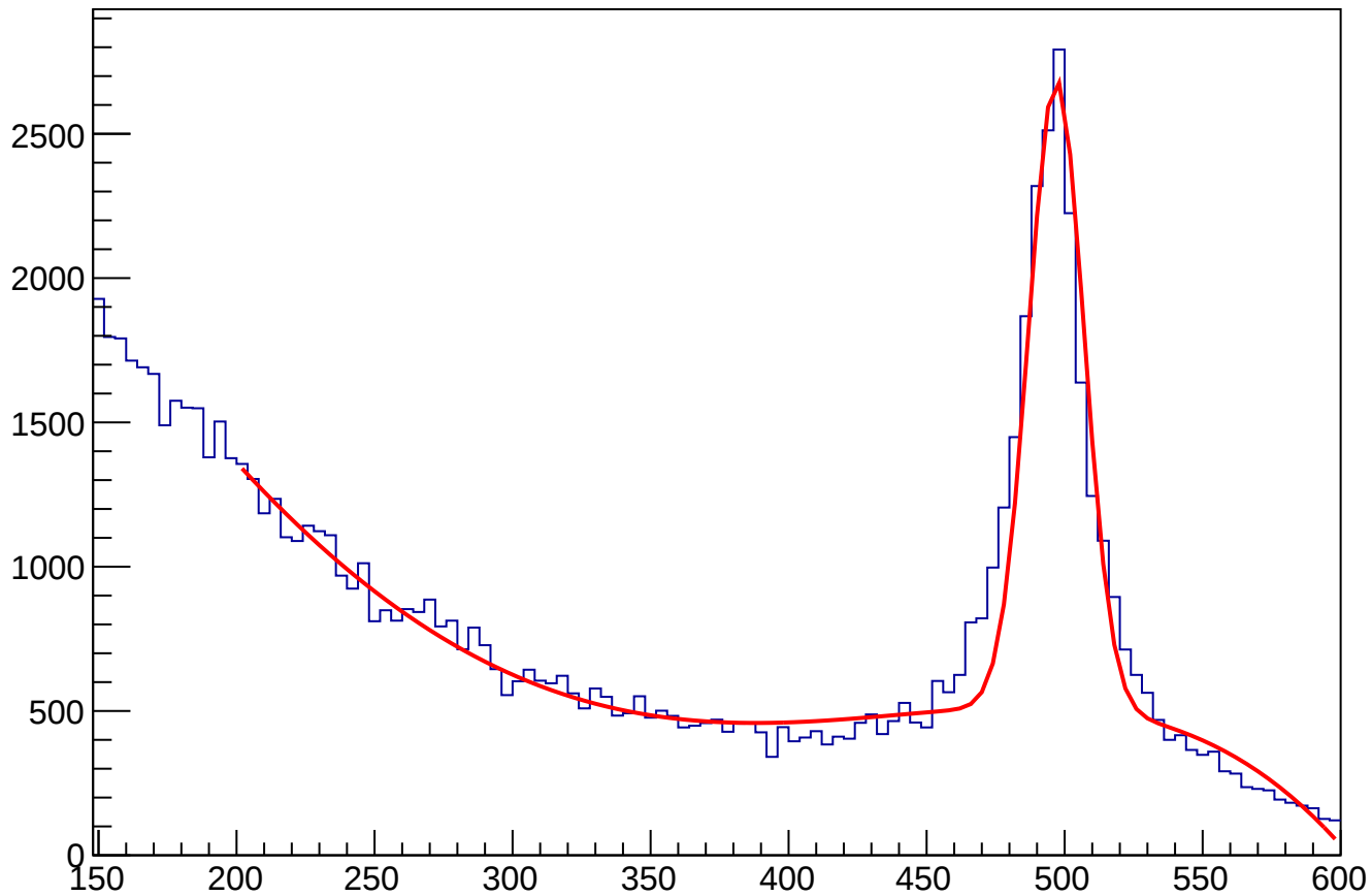
ECAL_gravTwoPhoton3ns_InDeltaPhi10Degree2Method
