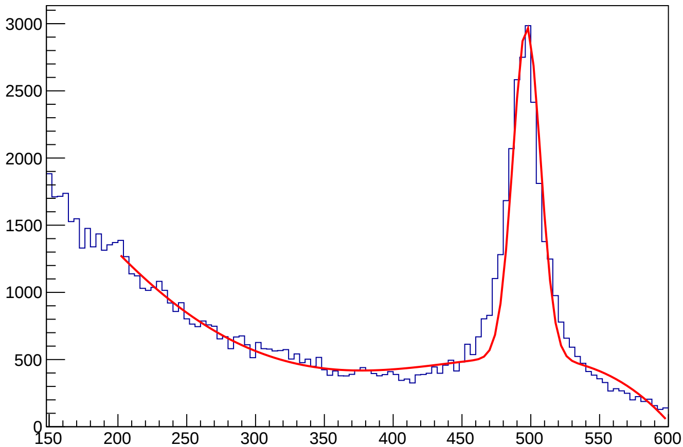
ECAL_gravTwoPhoton3ns_InDeltaPhi20Degree2Method_DeltaTheta
