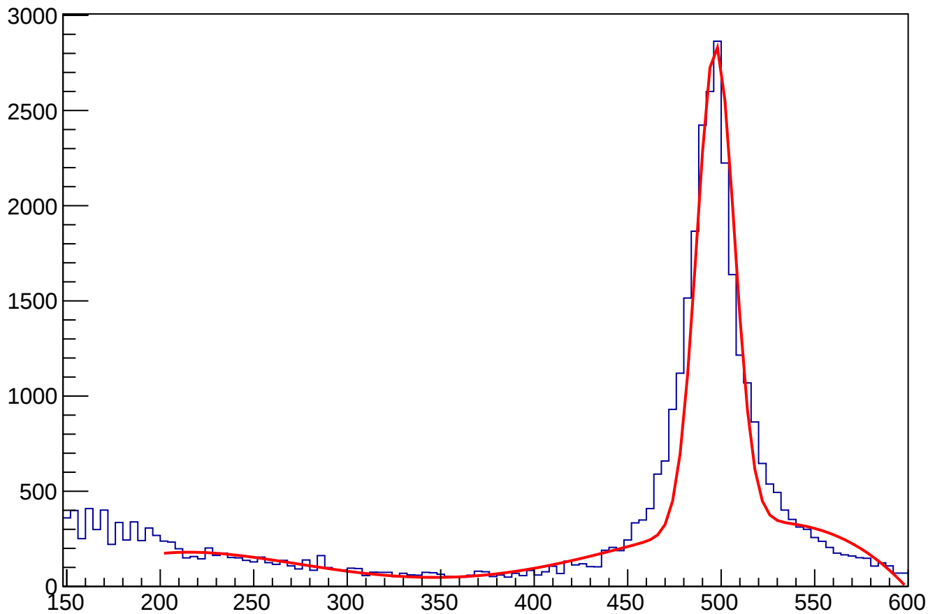
ECAL_gravTwoPhoton1.5ns3cm_withAngleCut
