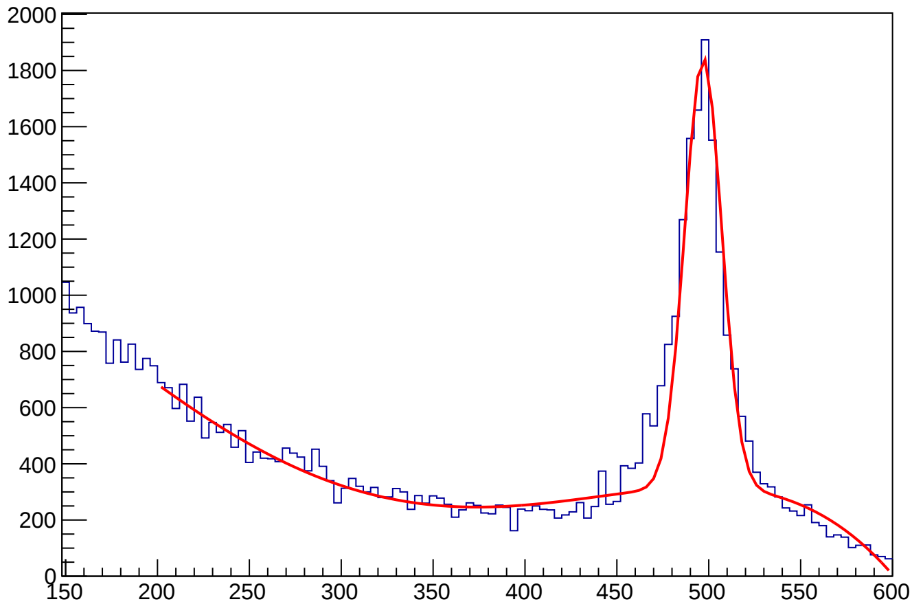
ECAL_gravTwoPhoton3ns_InDeltaPhi5Degree2Method
