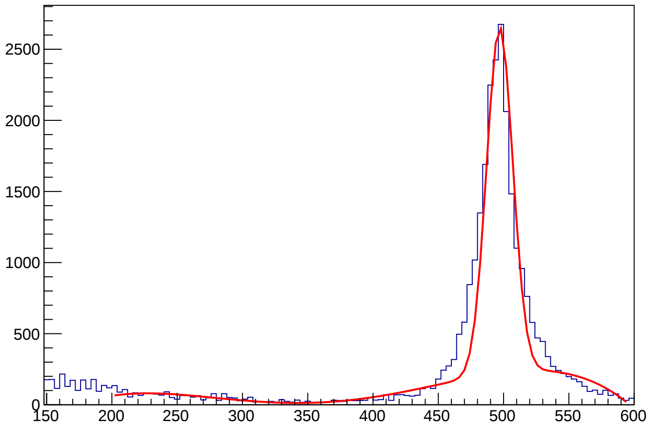
ECAL_gravTwoPhoton1.5ns2cm_withAngleCut
