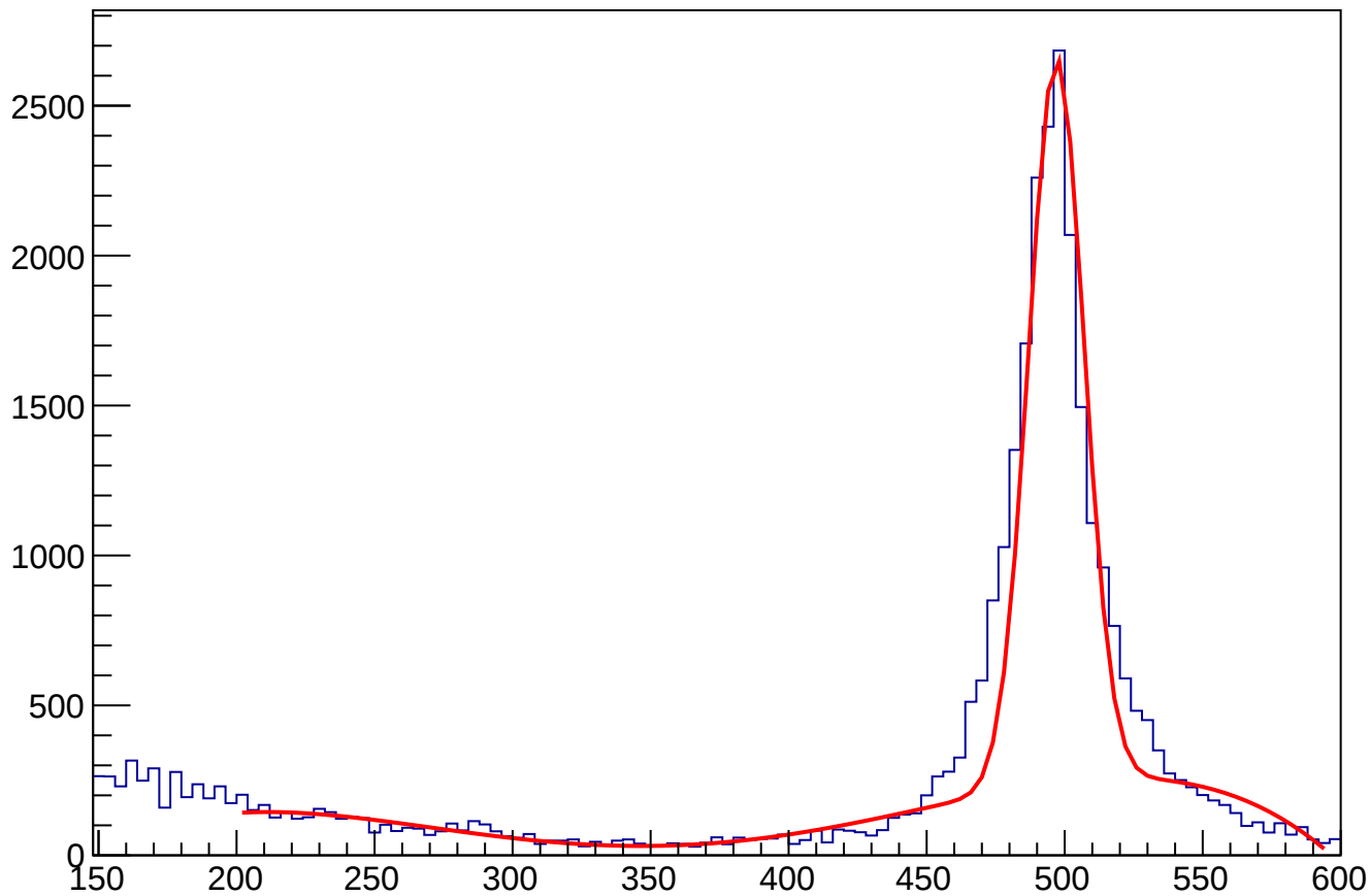
ECAL_gravTwoPhoton3ns2cm_withAngleCut
