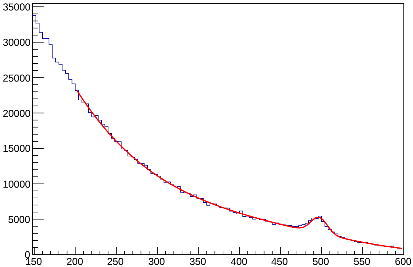
ECAL_twoPhotonInTime3ns
