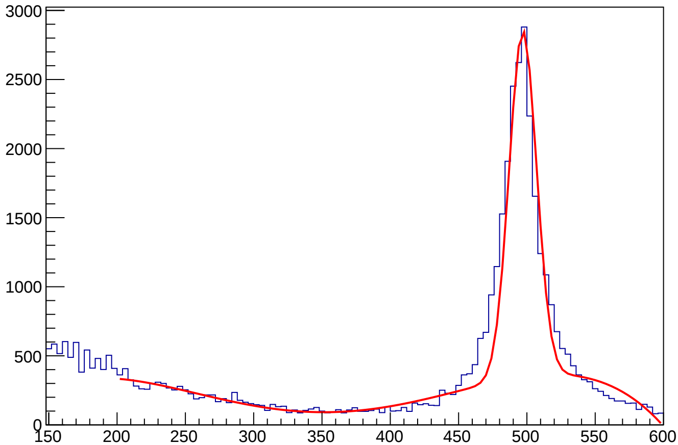
ECAL_gravTwoPhoton3ns3cm_withAngleCut
