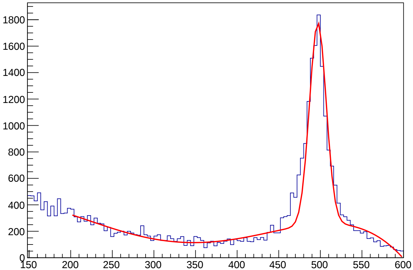
ECAL_gravTwoPhoton3ns_InDeltaPhi5Degree2Method_DeltaTheta
