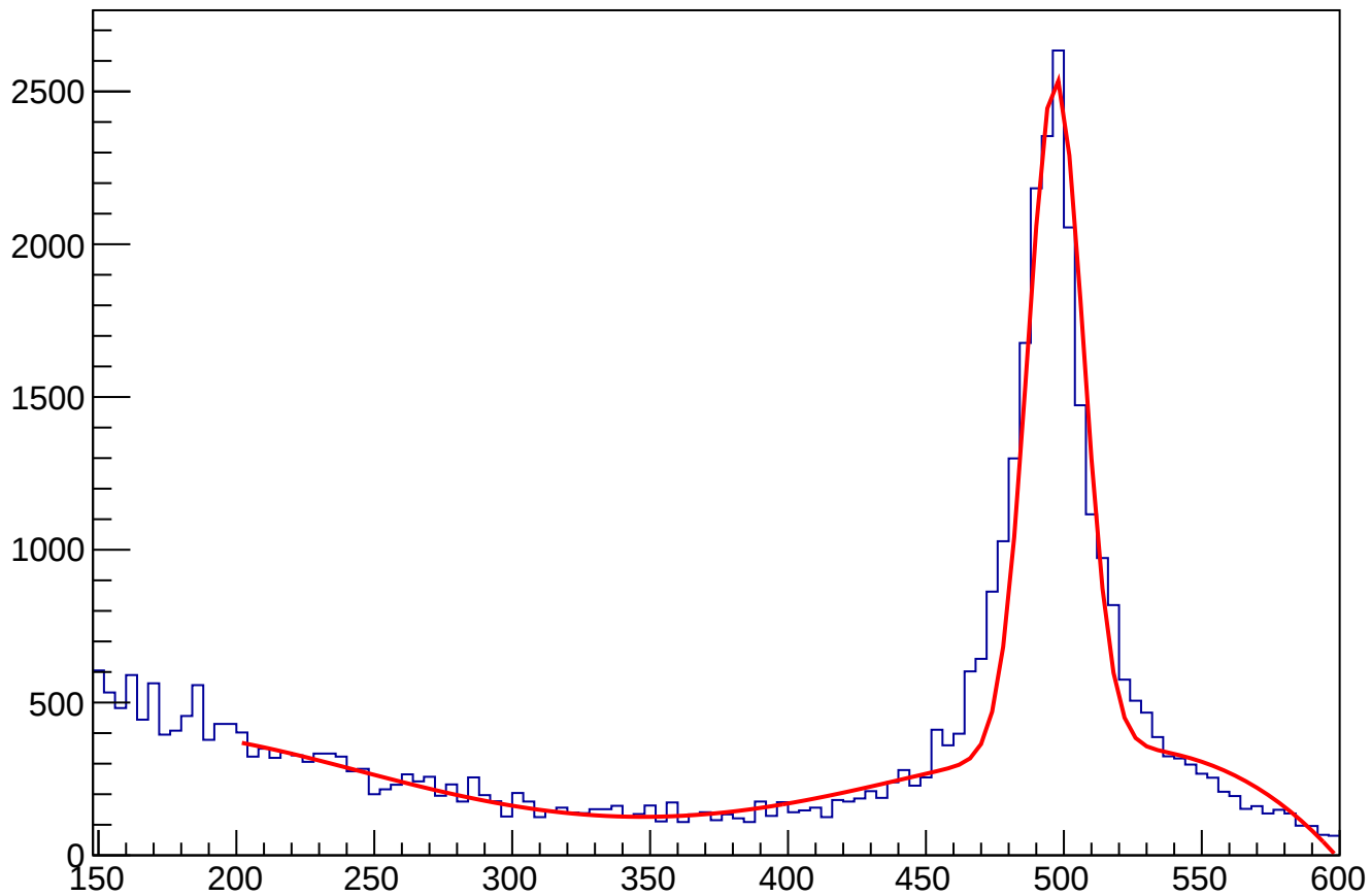
ECAL_gravTwoPhoton1.5ns_InDeltaPhi10Degree2Method_DeltaTheta
