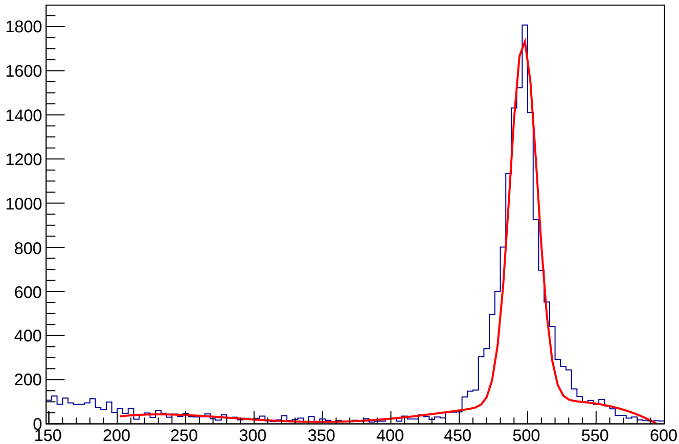
ECAL_gravTwoPhoton1.5ns1cm_InDeltaPhi
