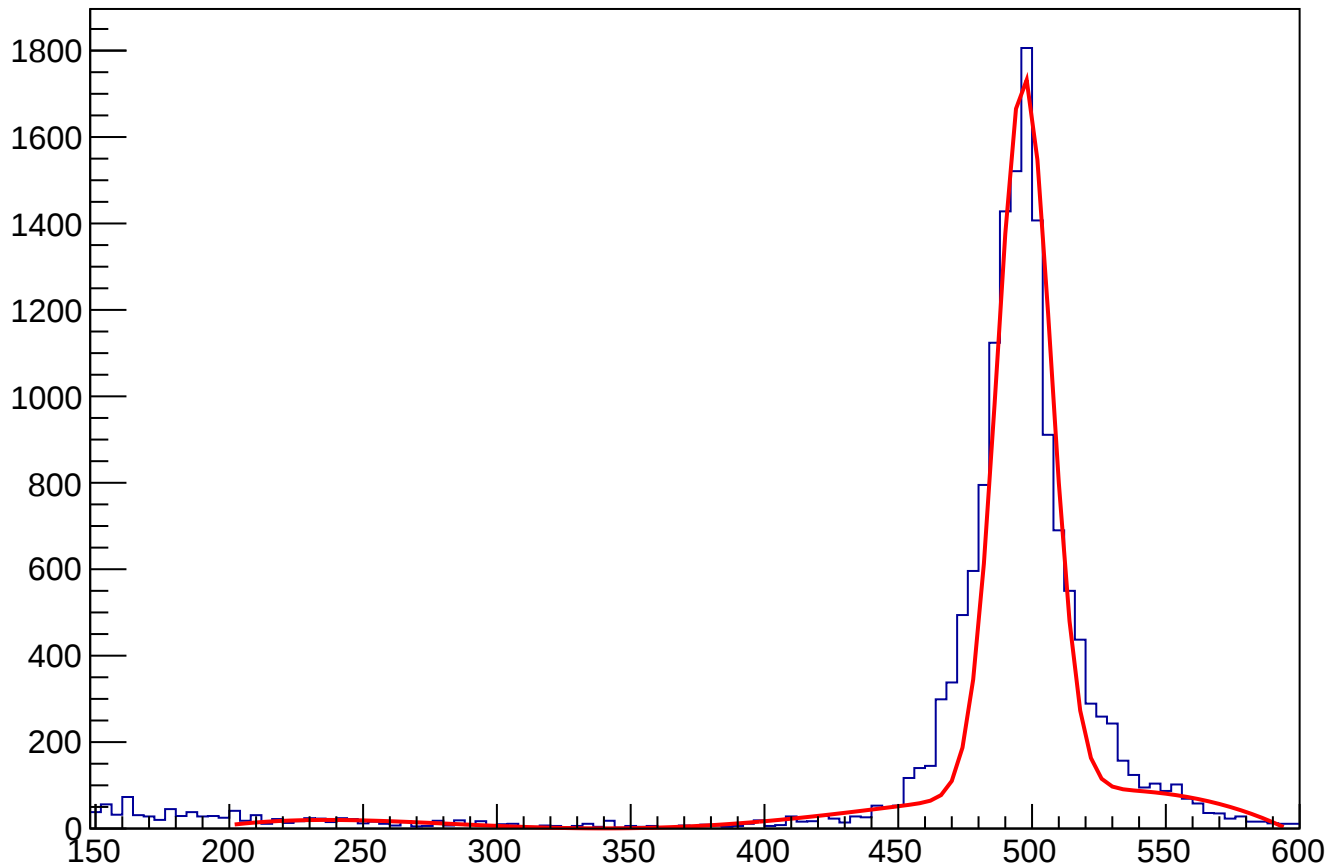
ECAL_gravTwoPhoton1.5ns1cm_InDeltaPhi_withAngleCut
