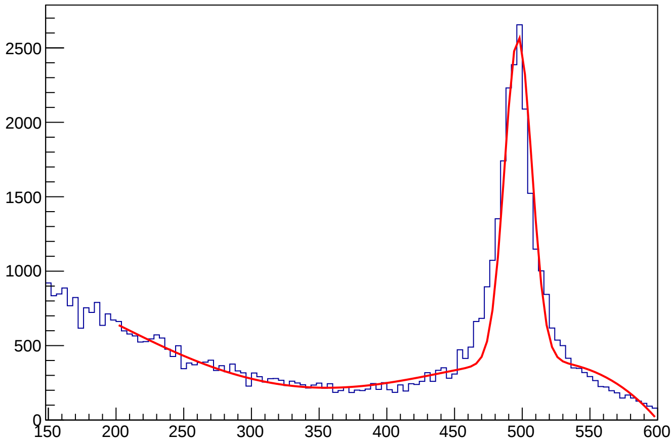
ECAL_gravTwoPhoton3ns_InDeltaPhi10Degree2Method_DeltaTheta
