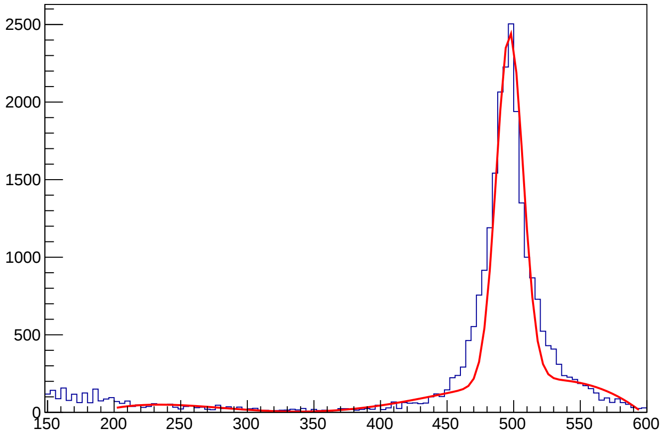
ECAL_gravTwoPhoton1.5ns2cm_InDeltaPhi_withAngleCut
