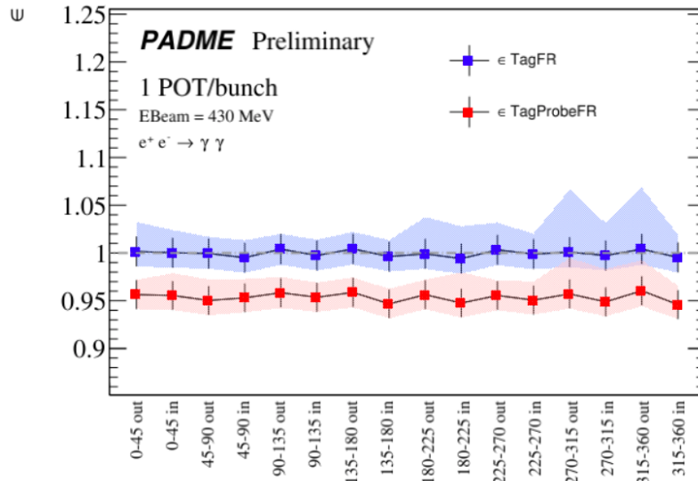
Figure 1.17: Tag and probe efficiency estimated for photons from annihilation events, in the absence of pileup and detector defects. The efficiency is quoted in 8 bins in phi each divided in 2 bins in R . The efficiency is quoted with (red) and without (blue) the requirement that the matched probe belongs to the fiducial region.
