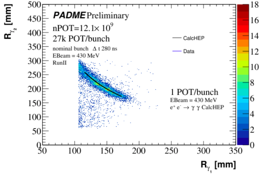
Figure 1.12: Correlation between the radius of the first and second photon. Points are PADME data after a tight selection of annihilation events, corresponding to cuts a,b,c,d,e presented in Section ???. The black line is the same correlation according to MC truth in CalHEP.
