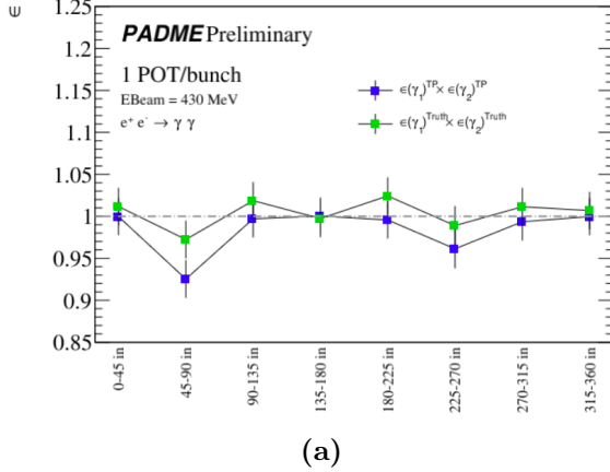
Figure 1.22: Event efficiency given by \epsilon(\gamma_1) \times \epsilon(\gamma_2) . On the right, the clusters used for the truth efficiency have a reconstructed energy above 90 MeV.
