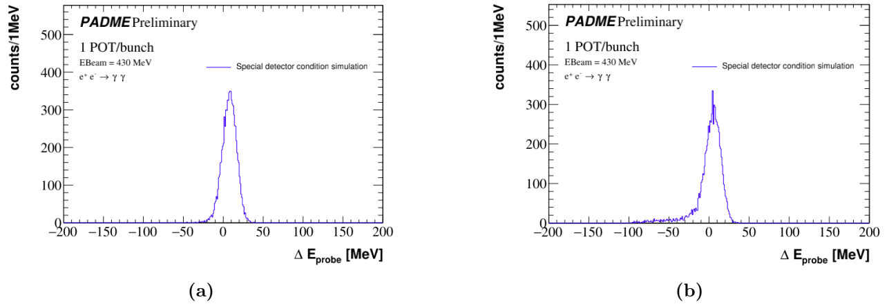
Figure 1.20: \Delta E_{Probe} distribution for the MC simulation of pure annihilation events in a simulation where the detector has dead channels. On the left the distribution is plotted for a bin without dead crystals, on the right the same distribution for tags reconstructed in the bin with dead crystals. add spatial cuts to the plots
