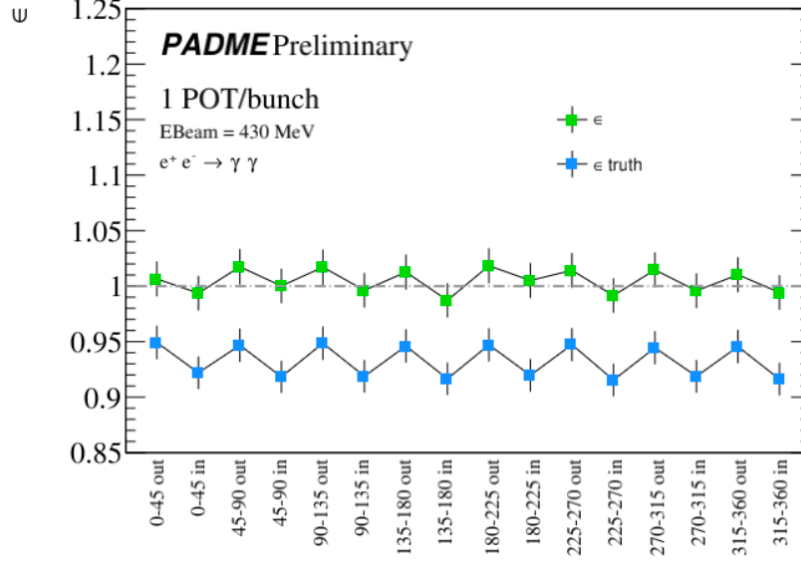
Figure 1.16: True and effective efficiency for photons from annihilation events, in the absence of pileup and detector defects. The efficiency is quoted in 8 bins in \phi each divided in 2 bins in R .
