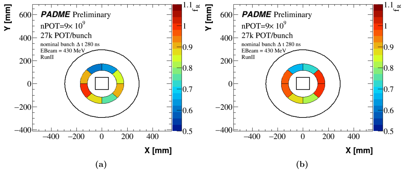
Figure 1.35: (a) Schematic view of the ratio between the bin maximum annihilation yield and the signals observed in each bin f_R . The belonging to this latest is defined by the most energetic photon. (b) f_R observed after the cluster position correction.
