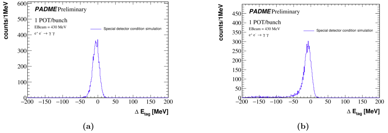
Figure 1.19: \Delta E_{Tag} distribution for the MC simulation of pure annihilation events in a simulation where the detector has dead channels. On the left the distribution is plotted for a bin without dead crystals, on the right the same distribution for tags reconstructed in the bin with dead crystals. add spatial cuts to the plots
