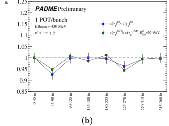
Figure 1.22: Event efficiency given by \epsilon(\gamma_1) \times \epsilon(\gamma_2) . On the right, the clusters used for the truth efficiency have a reconstructed energy above 90 MeV.
