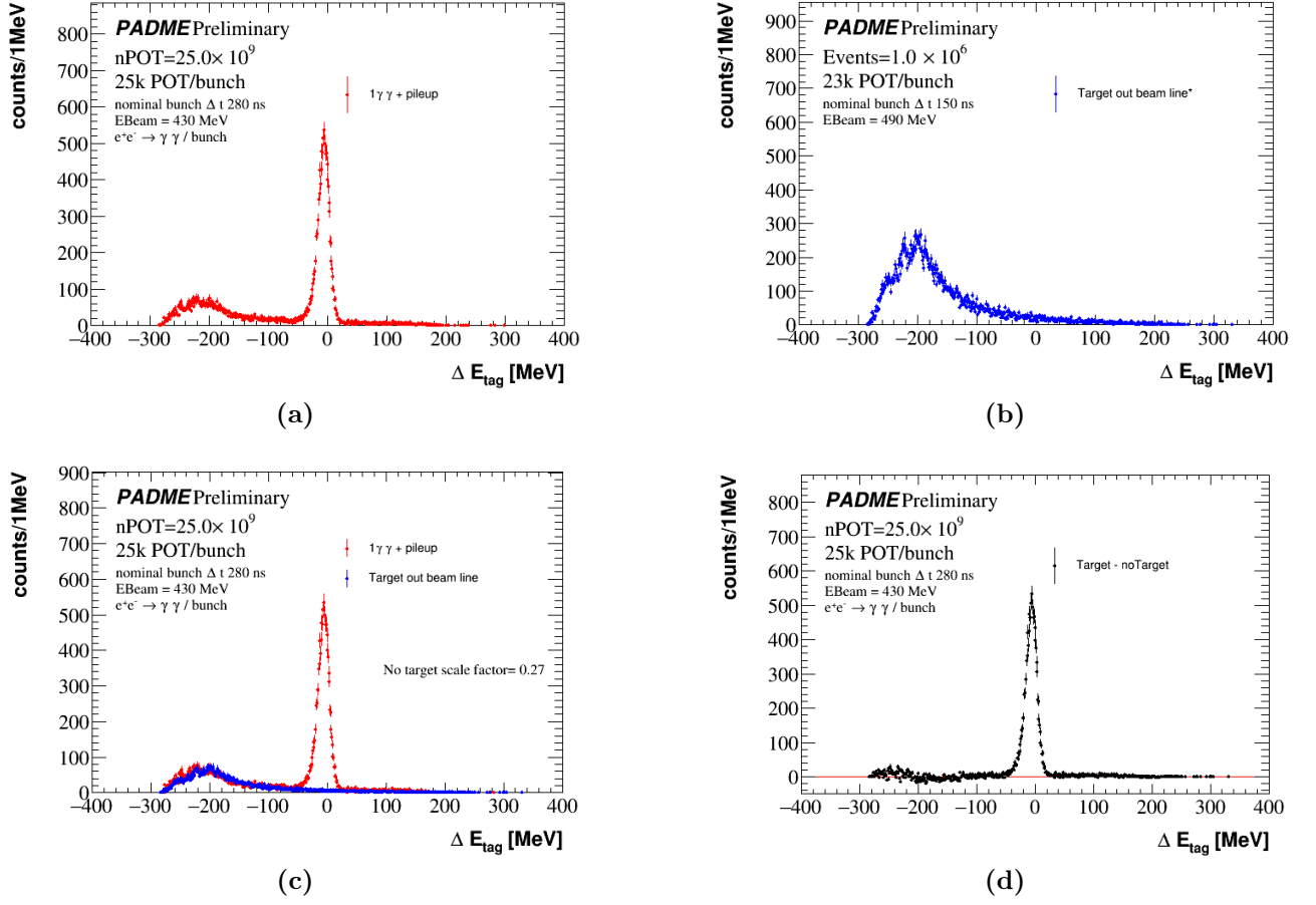
Figure 1.26: (a): Distribution of the \Delta E = E_{cl} - f(\theta) of the tag distribution for the CalcHEP simulation in pileup. (b): Distribution of the \Delta E = E_{cl} - f(\theta) for MC simulation of background (made with the target out of the beam line). (c): Comparison of (a) and scaled (b). (d) : Tag yield, obtained from the subtraction of the background to the signal.
