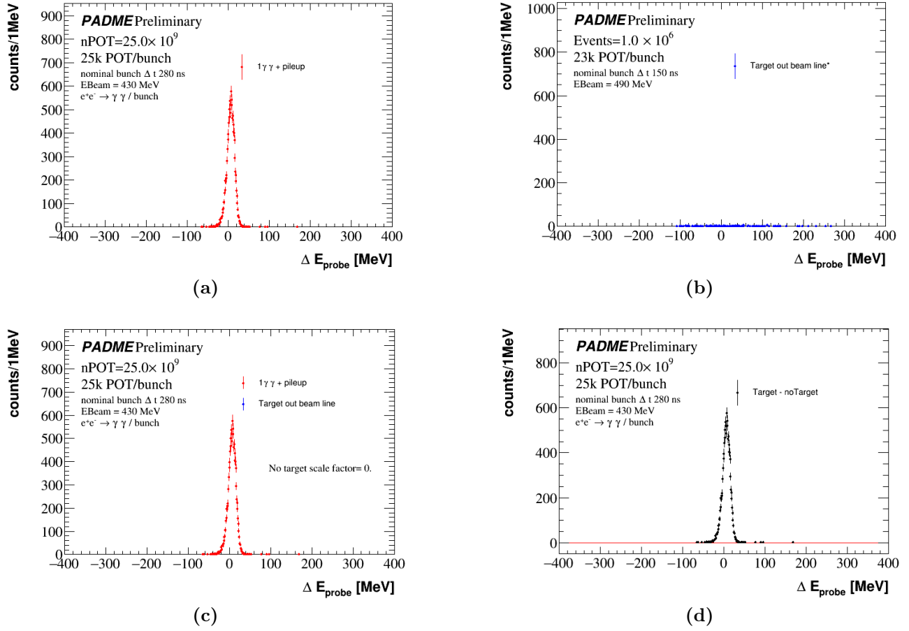
Figure 1.27: P(a): Distribution of the |\Delta E_{\text{Probe}} = E_{\text{cl}} - (E_{\text{Beam}} - f(\theta_{\text{Tag}})) of the probe matched distribution in the CalcHEP simulation with the pileup. (b): Distribution of the \Delta E_{\text{Probe}} for MC background (target out of the beam line). (c): Comparison of (a) and scaled (b). (d) : Probe yield, obtained from the subtraction of the background on the signal.
