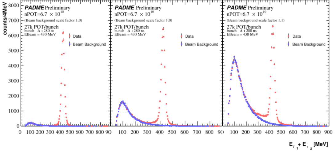
Figure 1.31: Distribution of E_{\gamma_1} + E_{\gamma_2} of the two photons that pass the selection a.b. described in Section ?? for standard run (red dots) and special one with target out of the target beam (blue dots). (a) additional selection CoG cut of 20 mm; (b) additional selection CoG cut of 50 mm; (c) additional selection CoG cut of 80 mm.
