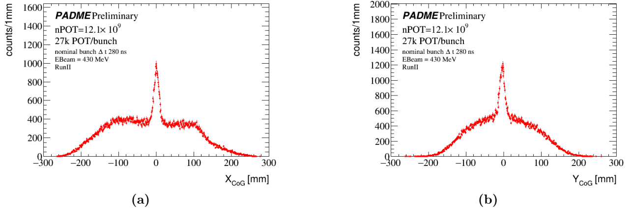
Figure 1.6: Distribution of the Center Of Gravity variables for the events that satisfy the following cuts, described in Table ??: time coincidence and first photon in FR. On the left (a) the distribution of X_{CoG} , on the right (b) the distribution of the Y_{CoG} .
