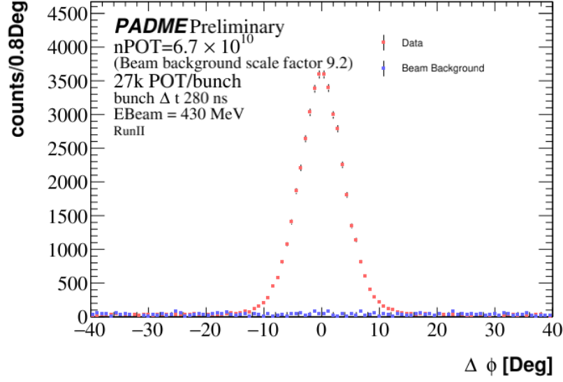
Figure 1.32: Distribution of \Delta\phi = \phi_{\gamma_1} - \phi_{\gamma_2} - 180 Deg of the two photons that pass the selection a.b.c. described in Section ?? for standard run (red dots) and special one with target out of the target beam (blue dots).
