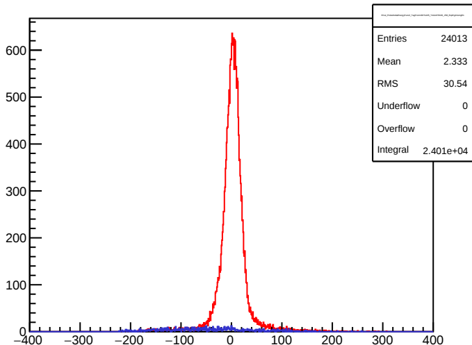
ECal_ProbeDeltaEnergyFunc2_TagFrom180To225_TAGinFR106_258_ExpEg2UsingE1
