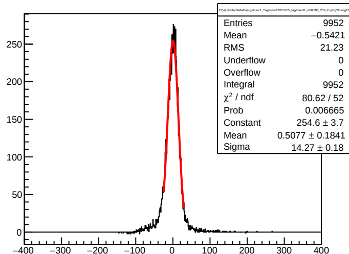
ECal_ProbeDeltaEnergyFunc2_TagFrom270To315_tagInnerR_inFR106_258_ExpEg2UsingE1
