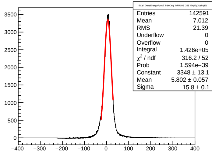
ECal_DeltaEnergyFunc2_in90Deg_inFR106_258_ExpEg2UsingE1
