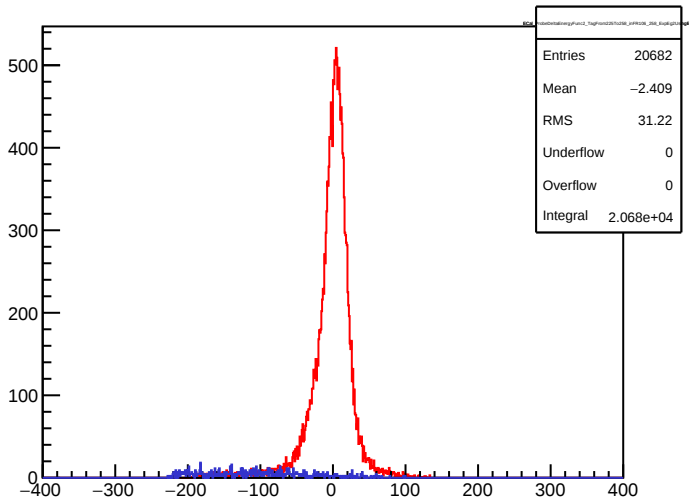
ECal_ProbeDeltaEnergyFunc2_TagFrom225To258_inFR106_258_ExpEg2UsingE1
