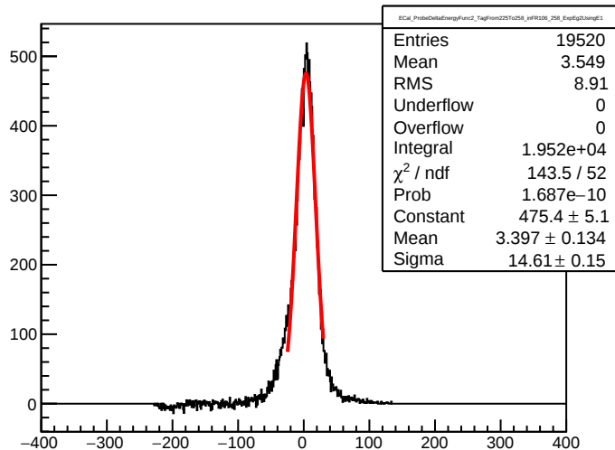
ECal_ProbeDeltaEnergyFunc2_TagFrom225To258_inFR106_258_ExpEg2UsingE1
