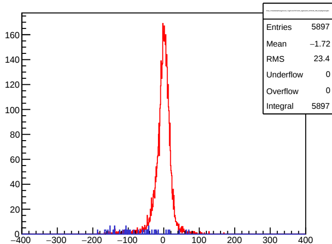
ECal_ProbeDeltaEnergyFunc2_TagFrom270To315_tagOuterR_inFR106_258_ExpEg2UsingE1
