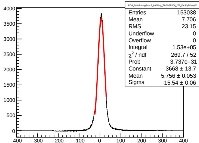
ECal_DeltaEnergyFunc2_in45Deg_TAGinFR106_258_ExpEg2UsingE1
