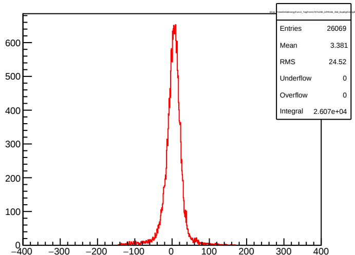
ECal_ProbeDeltaEnergyFunc2_TagFrom175To200_inFR106_258_ExpEg2UsingE1
