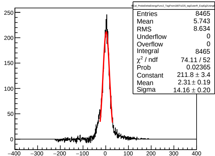
ECal_ProbeDeltaEnergyFunc2_TagFrom180To225_tagOuterR_ExpEg2UsingE1
