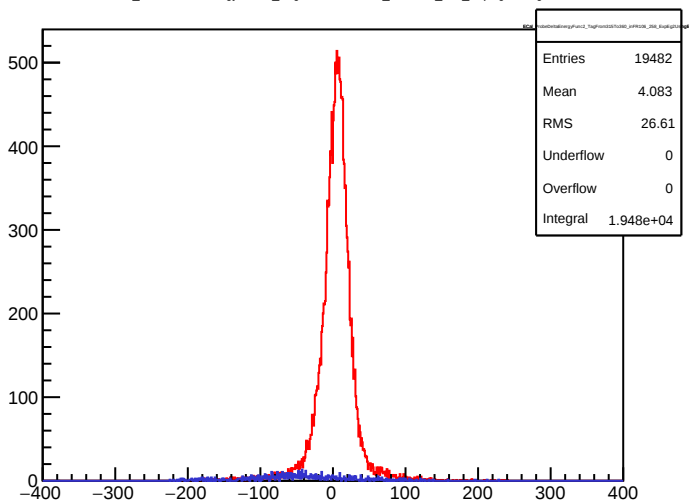
ECal_ProbeDeltaEnergyFunc2_TagFrom315To360_inFR106_258_ExpEg2UsingE1
