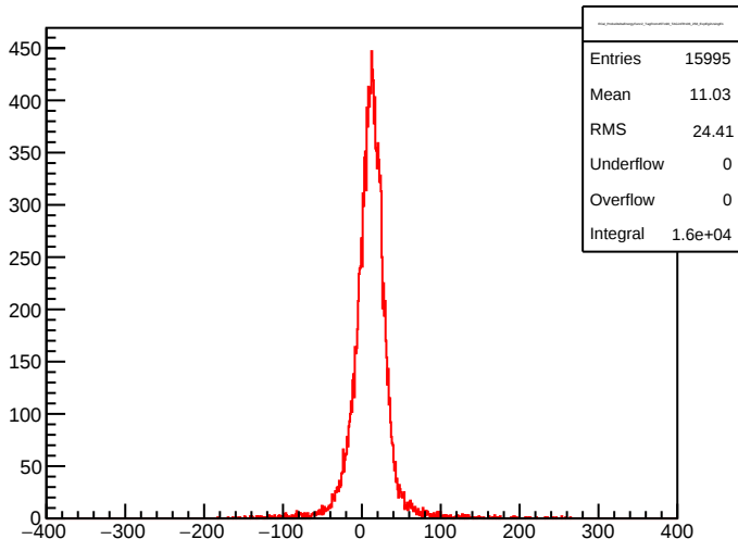
ECal_ProbeDeltaEnergyFunc2_TagFrom45To90_TAGinFR106_258_ExpEg2UsingE1
