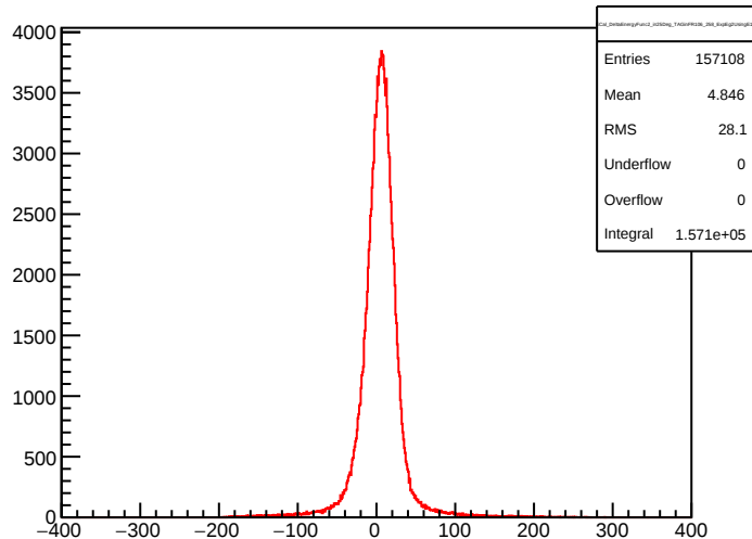
ECal_DeltaEnergyFunc2_in25Deg_TAGinFR106_258_ExpEg2UsingE1
