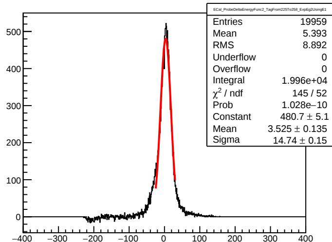
ECal_ProbeDeltaEnergyFunc2_TagFrom225To258_ExpEg2UsingE1
