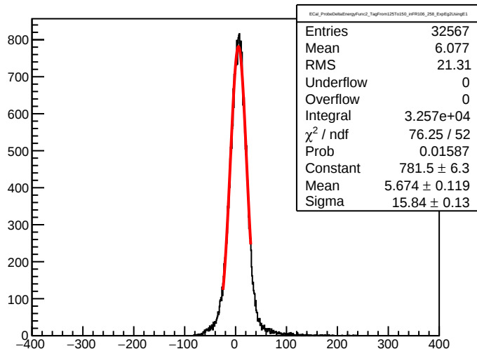
ECal_ProbeDeltaEnergyFunc2_TagFrom125To150_inFR106_258_ExpEg2UsingE1
