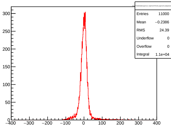
ECal_ProbeDeltaEnergyFunc2_TagFrom270To315_tagInnR_ExpEg2UsingE1
