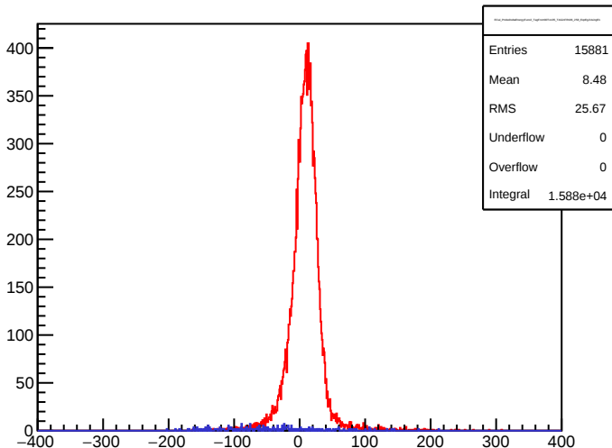
ECal_ProbeDeltaEnergyFunc2_TagFrom90To135_TAGinFR106_258_ExpEg2UsingE1
