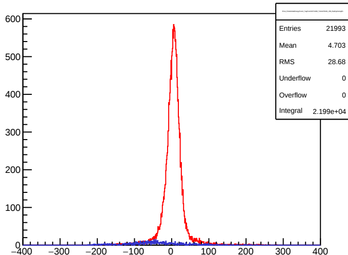
ECal_ProbeDeltaEnergyFunc2_TagFrom315To360_TAGinFR106_258_ExpEg2UsingE1
