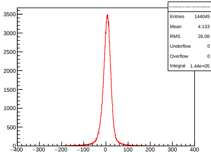
ECal_DeltaEnergyFunc2_in30Deg_inFR106_258_ExpEg2UsingE1
