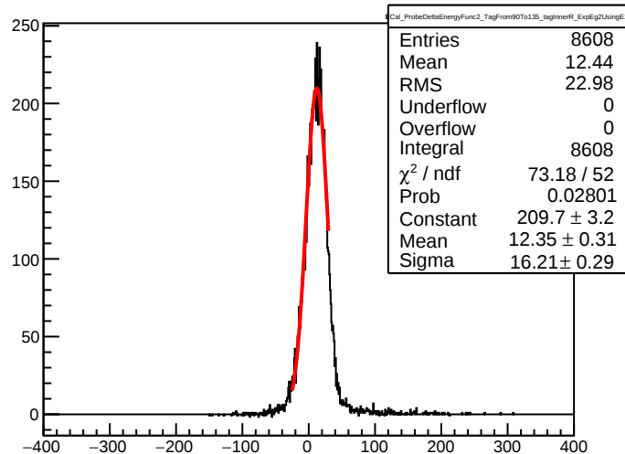
ECal_ProbeDeltaEnergyFunc2_TagFrom90To135_tagInnerR_ExpEq2UsingE1
