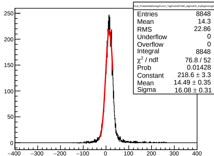
ECal_ProbeDeltaEnergyFunc2_TagFrom45To90_tagInnerR_ExpEg2UsingE1
