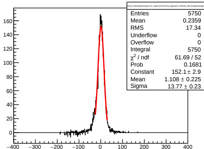
ECal_ProbeDeltaEnergyFunc2_TagFrom270To315_tagOuterR_inFR106_258_ExpEg2UsingE1
