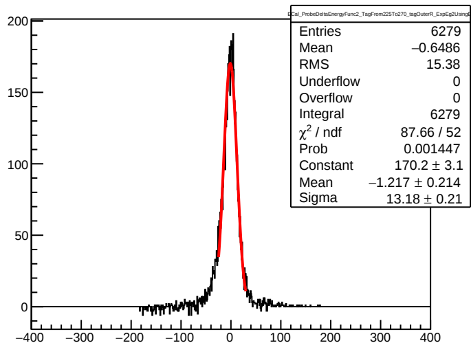
ECal_ProbeDeltaEnergyFunc2_TagFrom225To270_tagOuterR_ExpEg2UsingE1
