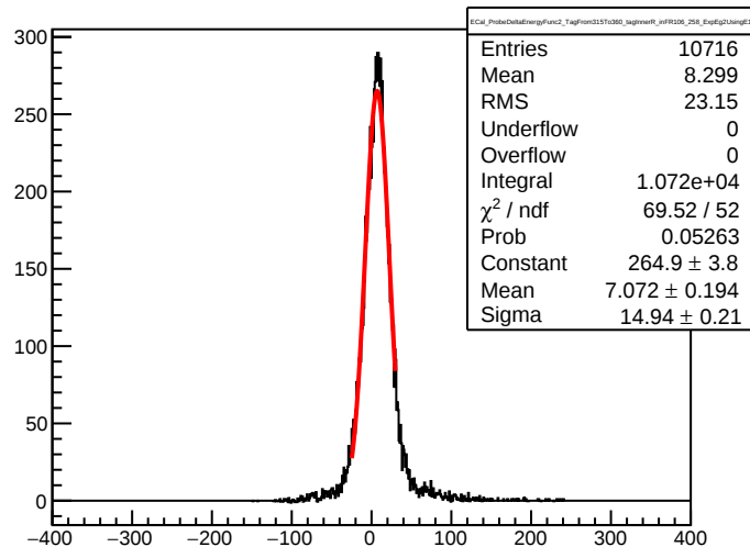
ECal_ProbeDeltaEnergyFunc2_TagFrom315To360_tagInnerR_inFR106_258_ExpEg2UsingE1
