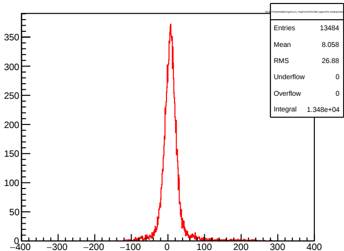
ECal_ProbeDeltaEnergyFunc2_TagFrom315To360_tagInnerR_ExpEg2UsingE1
