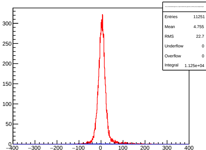
ECal_ProbeDeltaEnergyFunc2_TagFrom180To225_tagInnerR_inFR106_258_ExpEg2UsingE1
