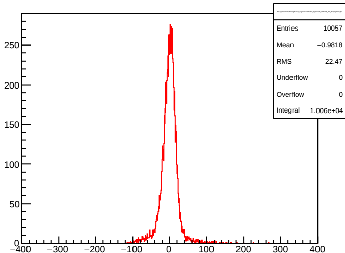
ECal_ProbeDeltaEnergyFunc2_TagFrom270To315_tagInnerR_inFR106_258_ExpEg2UsingE1
