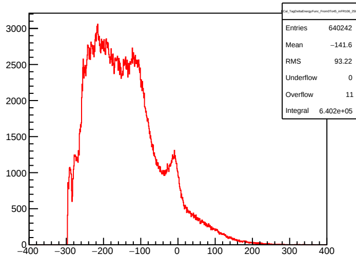
ECal_TagDeltaEnergyFunc_From0To45_inFR106_258
