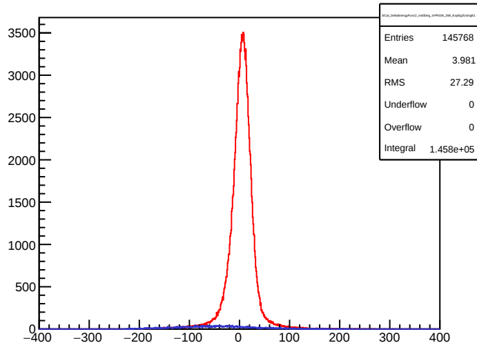
ECal_DeltaEnergyFunc2_in40Deg_inFR106_258_ExpEg2UsingE1
