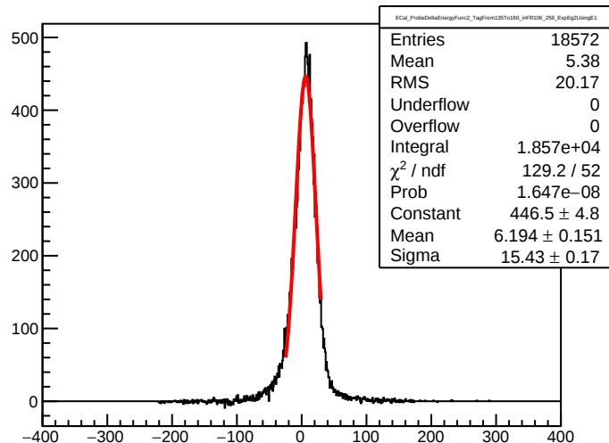
ECal_ProbeDeltaEnergyFunc2_TagFrom135To180_inFR106_258_ExpEg2UsingE1
