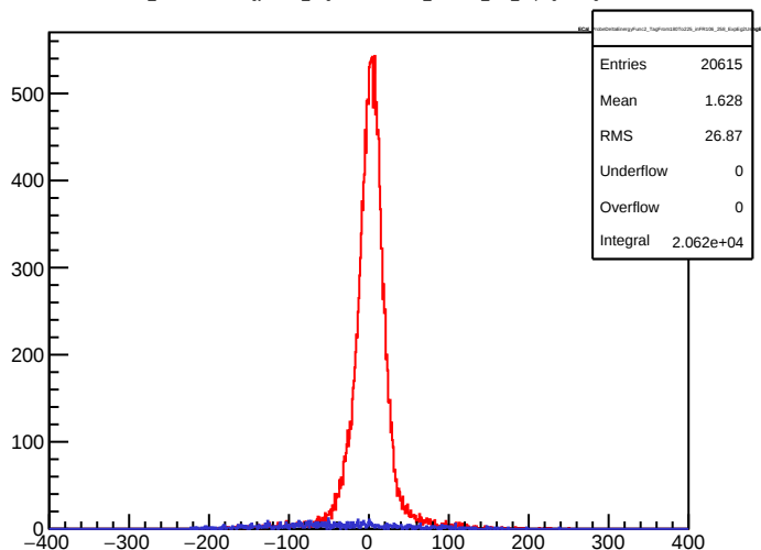
ECal_ProbeDeltaEnergyFunc2_TagFrom180To225_inFR106_258_ExpEg2UsingE1
