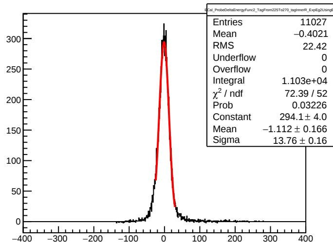
ECal_ProbeDeltaEnergyFunc2_TagFrom225To270_tagInnnerR_ExpEg2UsingE1
