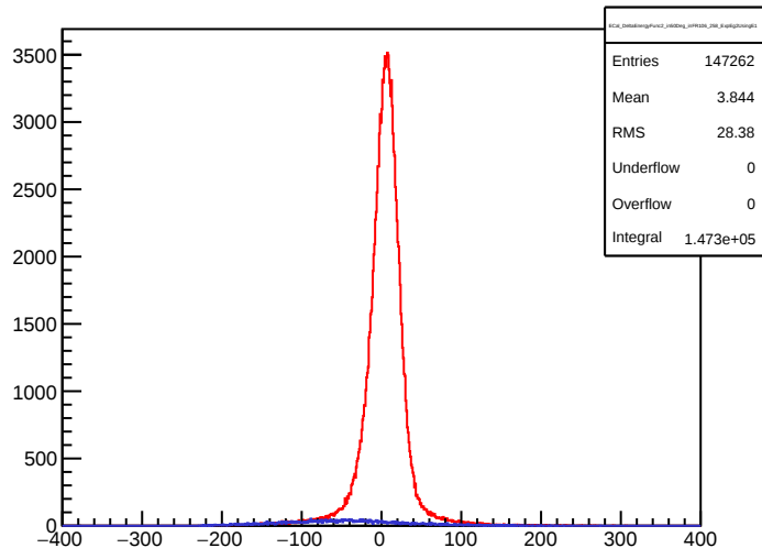
ECal_DeltaEnergyFunc2_in50Deg_inFR106_258_ExpEg2UsingE1
