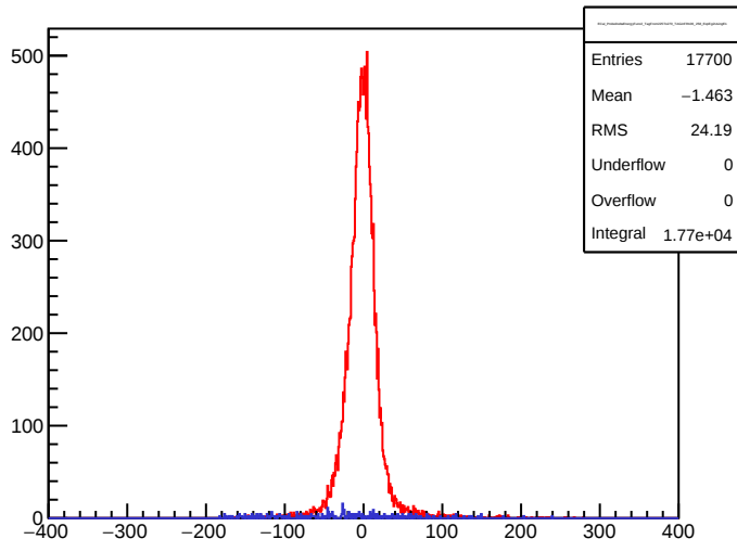
ECal_ProbeDeltaEnergyFunc2_TagFrom225To270_TAGinFR106_258_ExpEg2UsingE1
