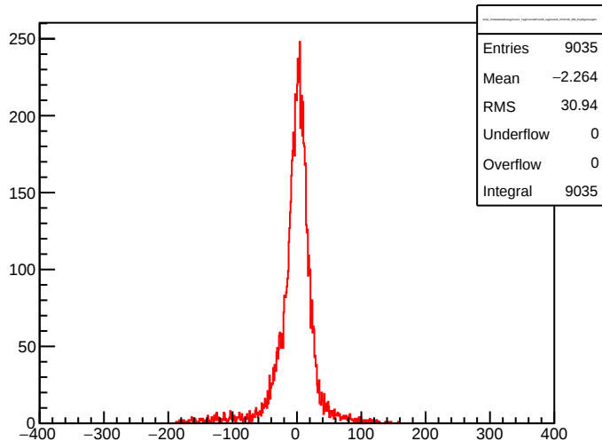
ECal_ProbeDeltaEnergyFunc2_TagFrom180to225_tagOuterR_inFR106_258_ExpEg2UsingE1
