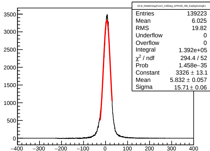
ECal_DeltaEnergyFunc2_in35Deg_inFR106_258_ExpEg2UsingE1
