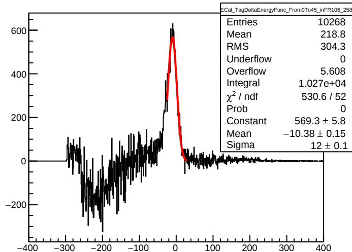
ECal_TagDeltaEnergyFunc_From0To45_inFR106_258
