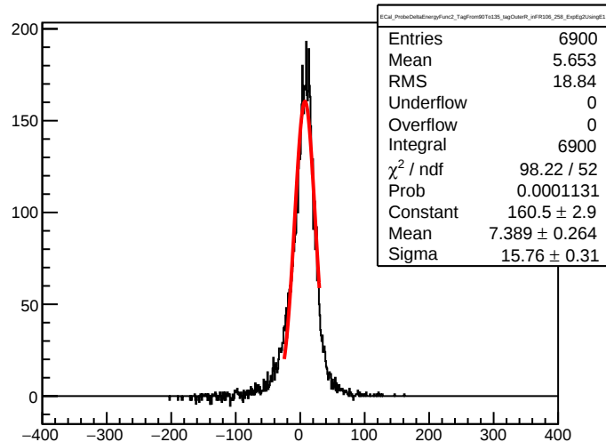
ECal_ProbeDeltaEnergyFunc2_TagFrom90To135_tagOuterR_inFR106_258_ExpEg2UsingE1
