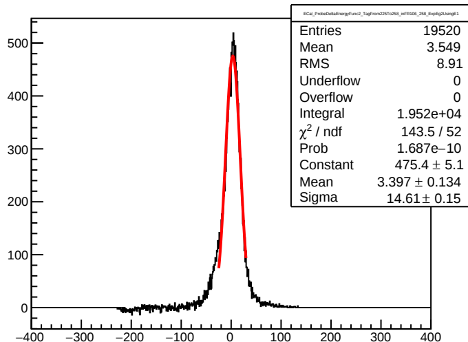
ECal_ProbeDeltaEnergyFunc2_TagFrom225To258_inFR106_258_ExpEg2UsingE1
