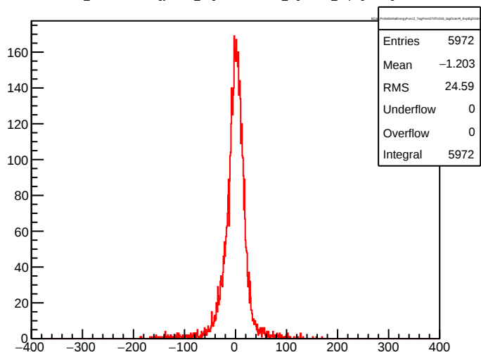
ECal_ProbeDeltaEnergyFunc2_TagFrom270To315_tagOuterR_ExpEg2UsingE1
