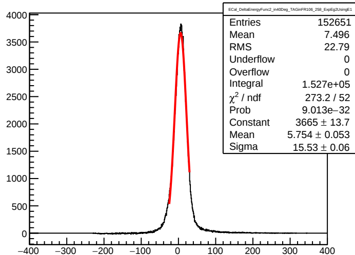
ECal_DeltaEnergyFunc2_in40Deg_TAGinFR106_258_ExpEg2UsingE1
