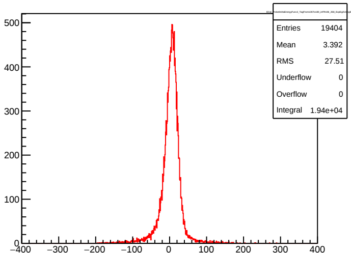
ECal_ProbeDeltaEnergyFunc2_TagFrom135To180_inFR106_258_ExpEg2UsingE1
