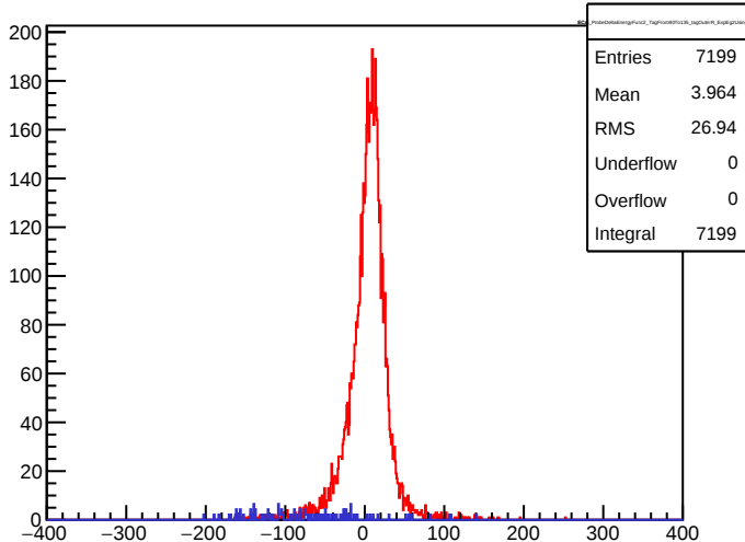
ECal_ProbeDeltaEnergyFunc2_TagFrom90To135_tagOuterR_ExpEg2UsingE1
