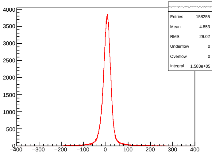
ECal_DeltaEnergyFunc2_in30Deg_TAGinFR106_258_ExpEg2UsingE1
