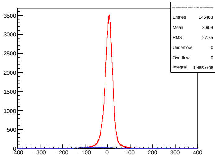
ECal_DeltaEnergyFunc2_in45Deg_inFR106_258_ExpEg2UsingE1
