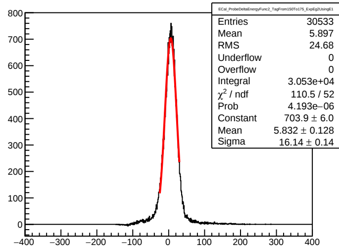
ECal_ProbeDeltaEnergyFunc2_TagFrom150To175_ExpEg2UsingE1
