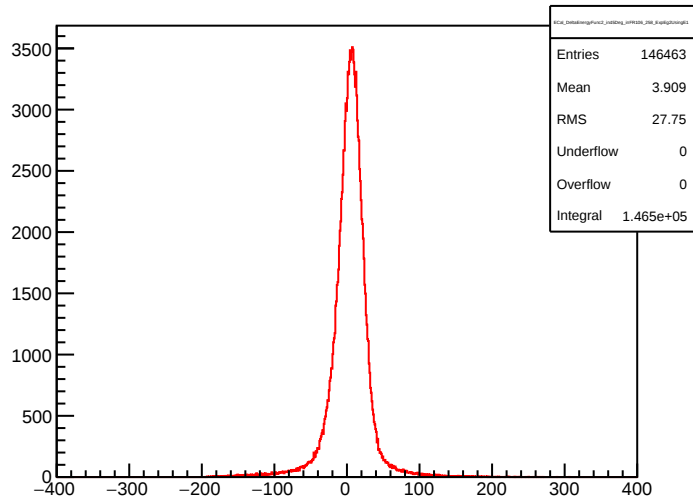
ECal_DeltaEnergyFunc2_in45Deg_inFR106_258_ExpEg2UsingE1
