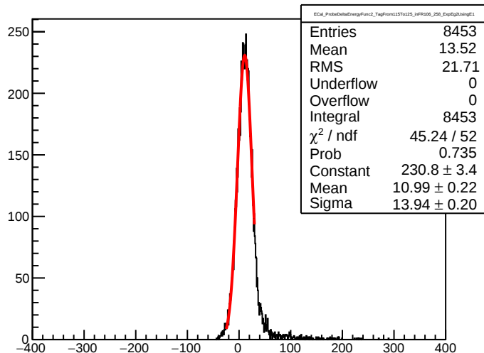
ECal_ProbeDeltaEnergyFunc2_TagFrom115To125_inFR106_258_ExpEg2UsingE1
