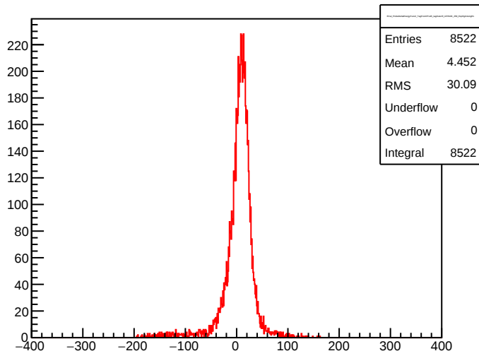
ECal_ProbeDeltaEnergyFunc2_TagFrom0To45_tagOuterR_inFR106_258_ExpEg2UsingE1
