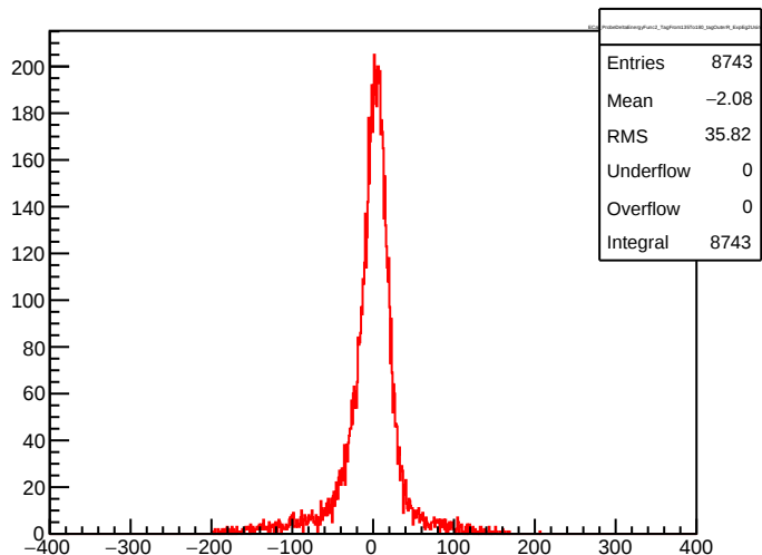
ECal_ProbeDeltaEnergyFunc2_TagFrom135To180_tagOuterR_ExpEg2UsingE1
