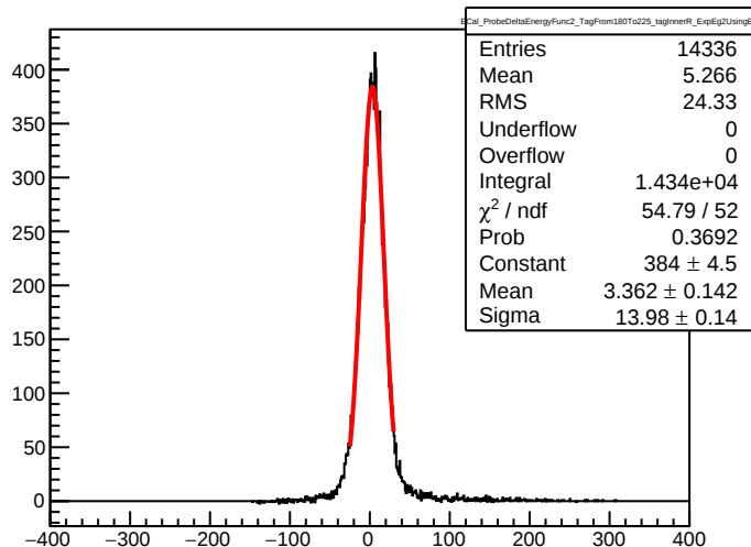
ECa1_ProbeDeltaEnergyFunc2_TagFrom180To225_tagInnerR_ExpEg2UsingE1
