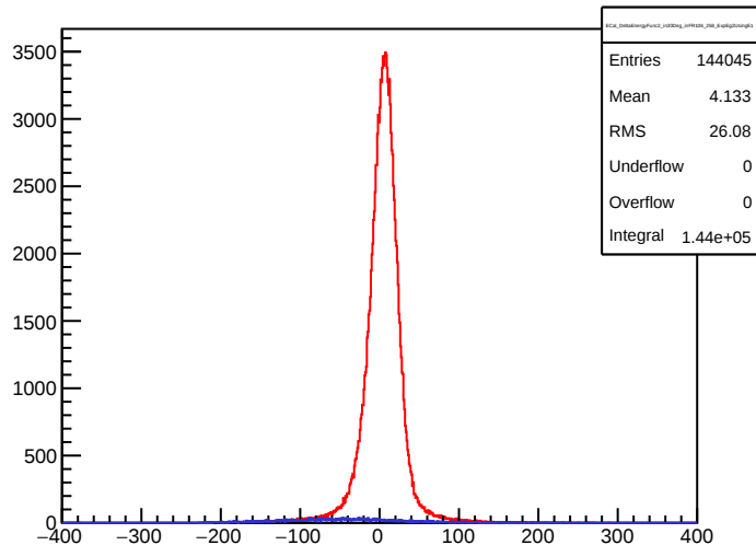
ECal_DeltaEnergyFunc2_in30Deg_inFR106_258_ExpEg2UsingE1
