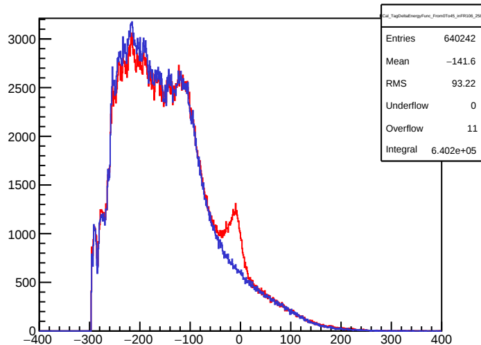
ECal_TagDeltaEnergyFunc_From0To45_inFR106_258
