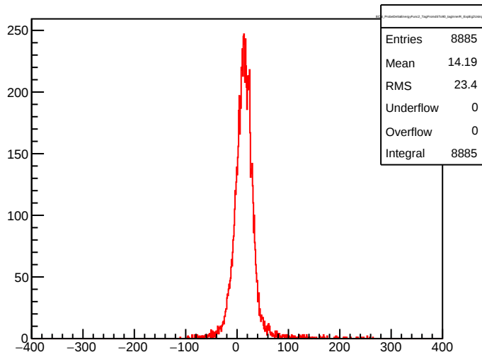
ECal_ProbeDeltaEnergyFunc2_TagFrom45To90_tagInnerR_ExpEg2UsingE1
