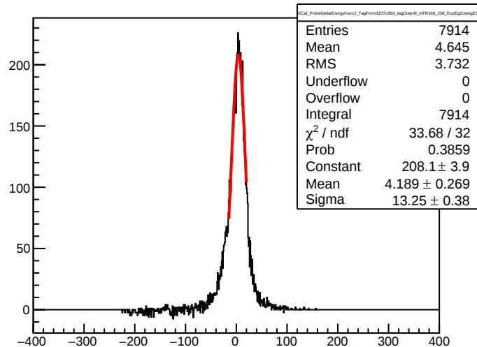
ECal_ProbeDeltaEnergyFunc2_TagFrom315To360_tagOuterR_inFR106_258_ExpEg2UsingE1
