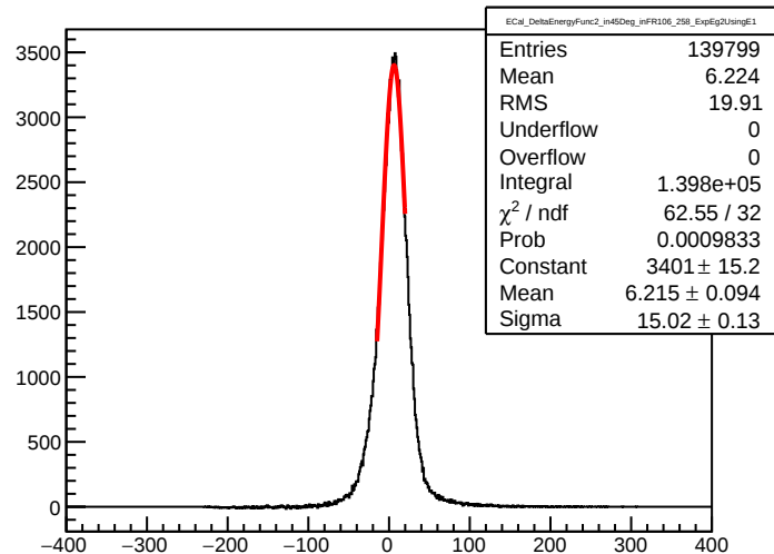
ECal_DeltaEnergyFunc2_in45Deg_inFR106_258_ExpEg2UsingE1
