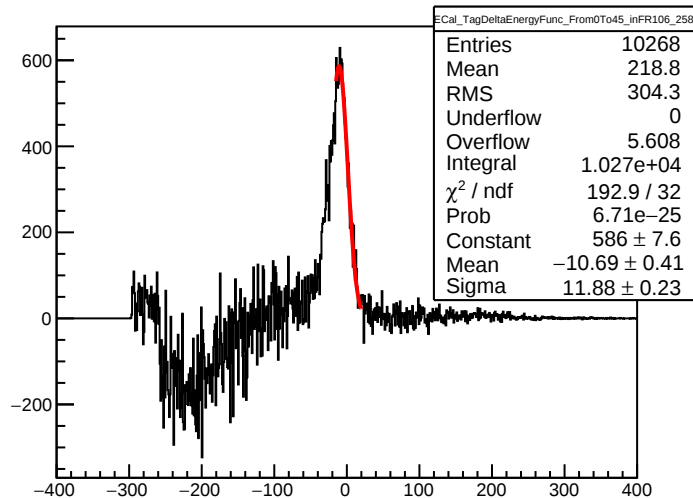
ECal_TagDeltaEnergyFunc_From0To45_inFR106_258
