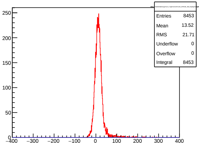
ECal_ProbeDeltaEnergyFunc2_TagFrom115To125_inFR106_258_ExpEg2UsingE1
