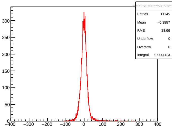
ECa1_ProbeDeltaEnergyFunc2_TagFrom225To270_tagInnnerR_ExpEg2UsingE1
