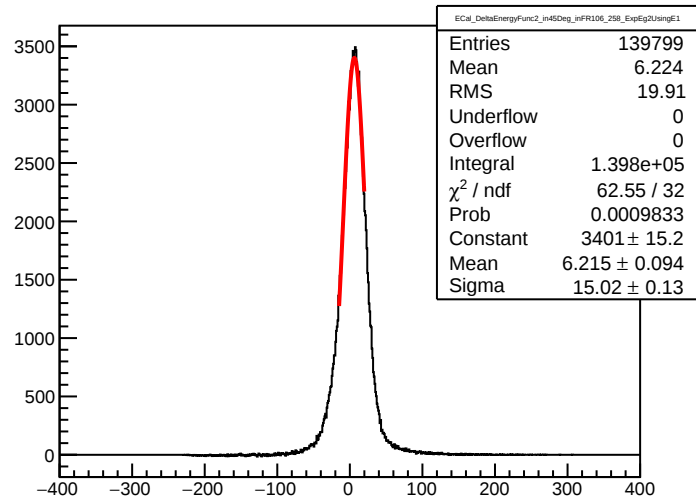
ECal_DeltaEnergyFunc2_in45Deg_inFR106_258_ExpEg2UsingE1
