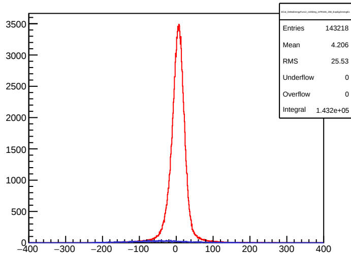
ECal_DeltaEnergyFunc2_in25Deg_inFR106_258_ExpEg2UsingE1
