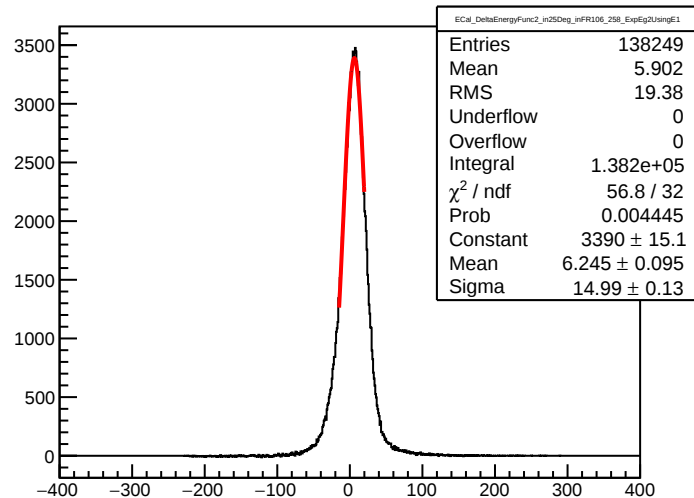
ECal_DeltaEnergyFunc2_in25Deg_inFR106_258_ExpEg2UsingE1
