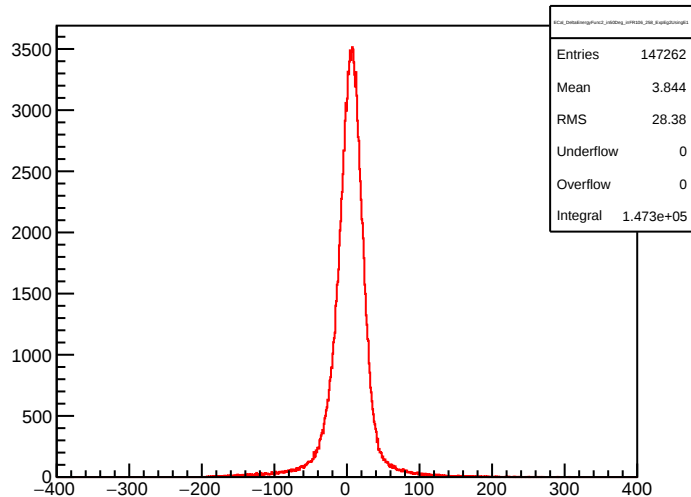
ECaI_DeltaEnergyFunc2_in50Deg_inFR106_258_ExpEg2UsingE1
