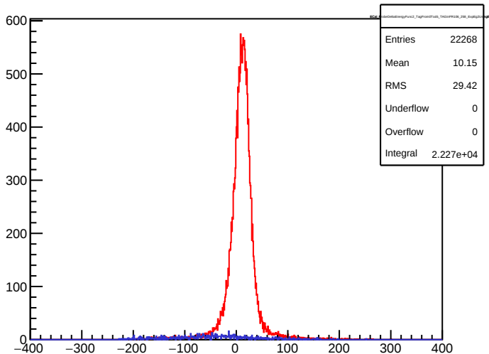
ECal_ProbeDeltaEnergyFunc2_TagFrom0To45_TAGinFR106_258_ExpEg2UsingE1
