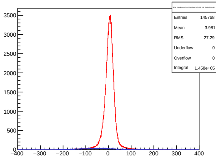
ECaL_DeltaEnergyFunc2_in40Deg_inFR106_258_ExpEg2UsingE1
