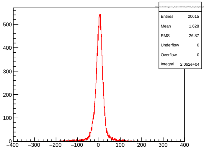
ECal_ProbeDeltaEnergyFunc2_TagFrom180To225_inFR106_258_ExpEg2UsingE1
