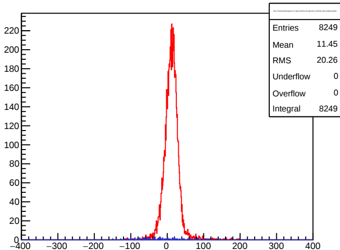
ECal_ProbeDeltaEnergyFunc2_TagFrom90To135_taginnerR_inFR106_258_ExpEg2UsingE1
