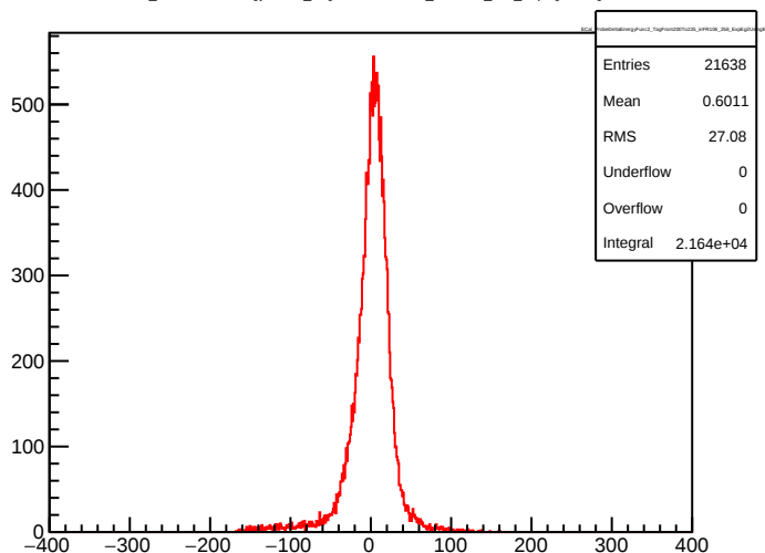
ECal_ProbeDeltaEnergyFunc2_TagFrom200To225_inFR106_258_ExpEg2UsingE1
