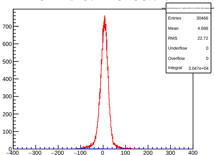
ECal_ProbeDeltaEnergyFunc2_TagFrom150To175_inFR106_258_ExpEg2UsingE1
