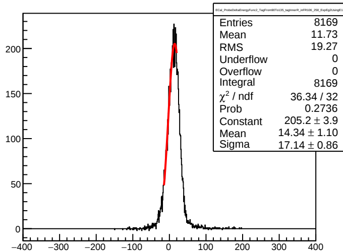
ECal_ProbeDeltaEnergyFunc2_TagFrom90To135_taginnerR_inFR106_258_ExpEg2UsingE1
