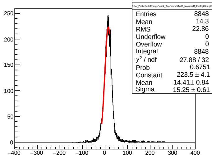
ECal_ProbeDeltaEnergyFunc2_TagFrom45To90_tagInnerR_ExpEg2UsingE1
