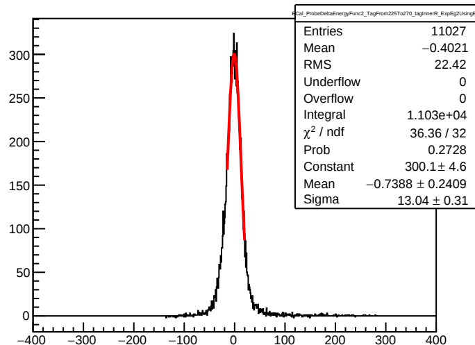
ECa1_ProbeDeltaEnergyFunc2_TagFrom225To270_tagInnnerR_ExpEg2UsingE1
