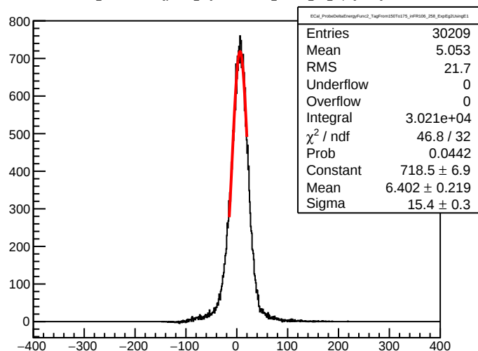
ECal_ProbeDeltaEnergyFunc2_TagFrom150To175_inFR106_258_ExpEg2UsingE1
