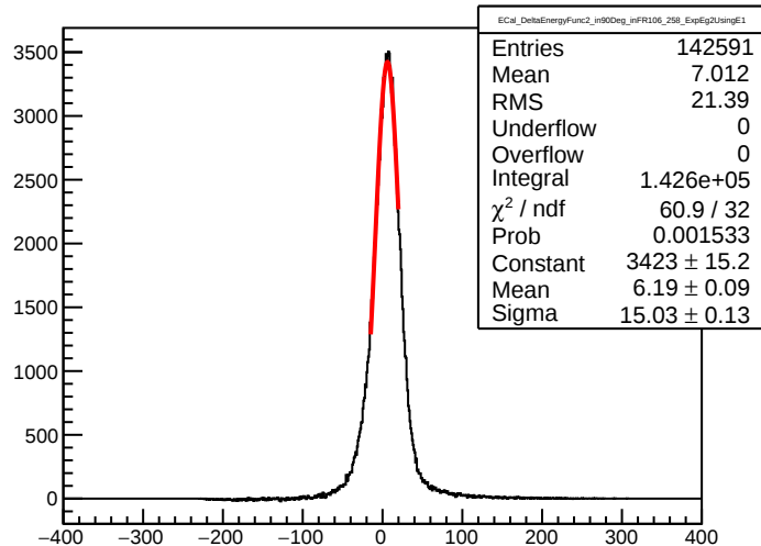
ECal_DeltaEnergyFunc2_in90Deg_inFR106_258_ExpEg2UsingE1
