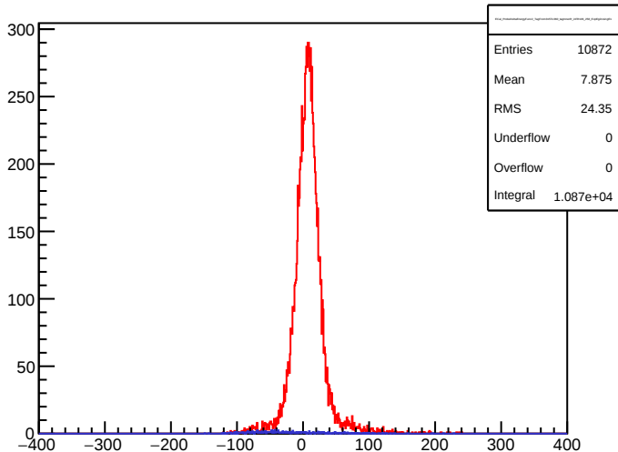
ECal_ProbeDeltaEnergyFunc2_TagFrom315To360_tagInnerR_inFR106_258_ExpEg2UsingE1
