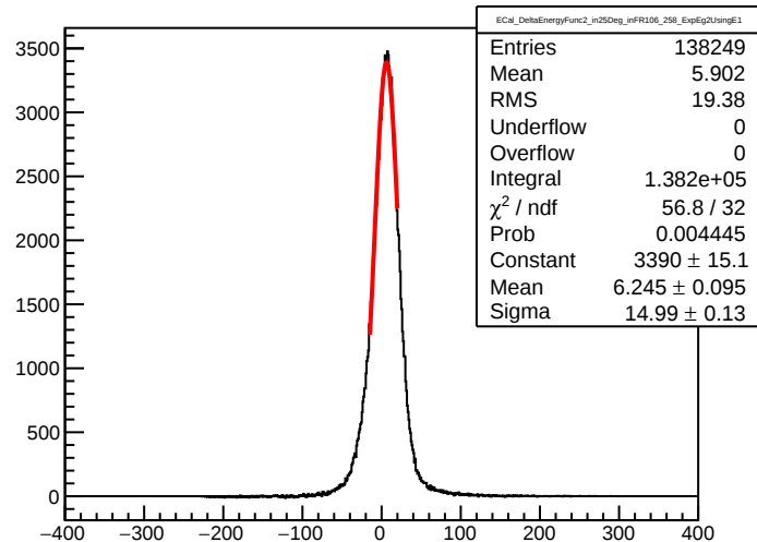
ECal_DeltaEnergyFunc2_in25Deg_inFR106_258_ExpEg2UsingE1
