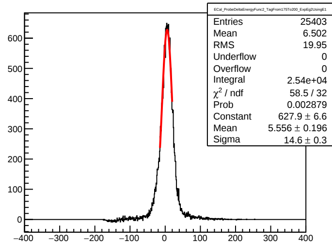
ECal_ProbeDeltaEnergyFunc2_TagFrom175To200_ExpEg2UsingE1
