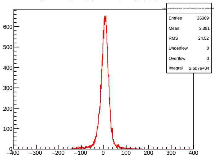
ECal_ProbeDeltaEnergyFunc2_TagFrom175To200_inFR106_258_ExpEg2UsingE1
