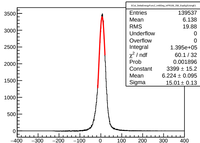
ECaL_DeltaEnergyFunc2_in40Deg_inFR106_258_ExpEg2UsingE1
