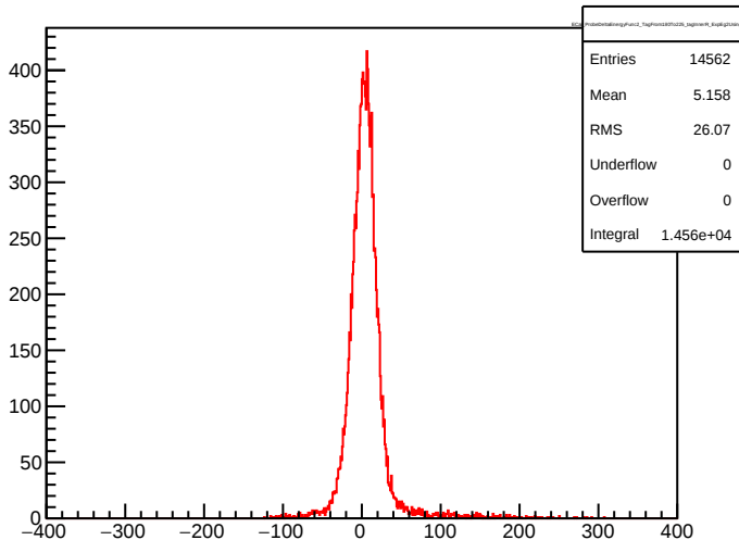
ECal_ProbeDeltaEnergyFunc2_TagFrom180To225_tagInnerR_ExpEg2UsingE1
