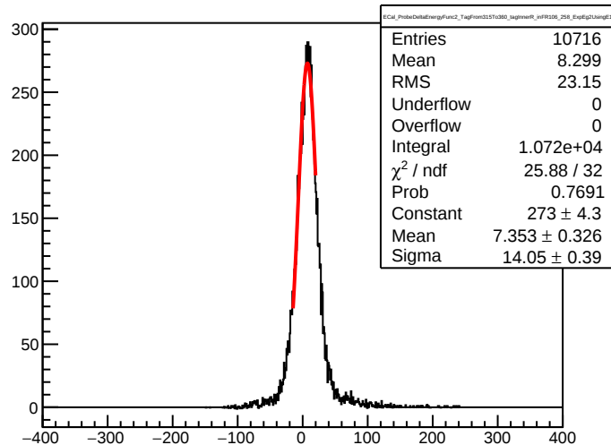
ECal_ProbeDeltaEnergyFunc2_TagFrom315To360_tagInnerR_inFR106_258_ExpEg2UsingE1
