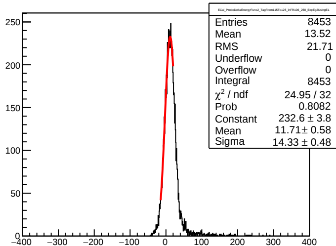
ECal_ProbeDeltaEnergyFunc2_TagFrom115To125_inFR106_258_ExpEg2UsingE1
