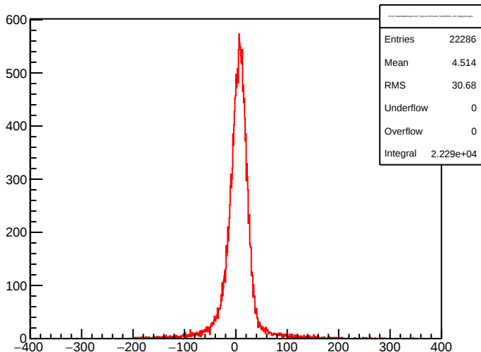
ECal_ProbeDeltaEnergyFunc2_TagFrom135To180_TAGinFR106_258_ExpEg2UsingE1
