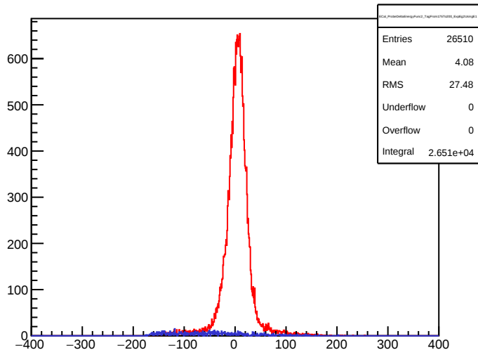
ECal_ProbeDeltaEnergyFunc2_TagFrom175To200_ExpEg2UsingE1
