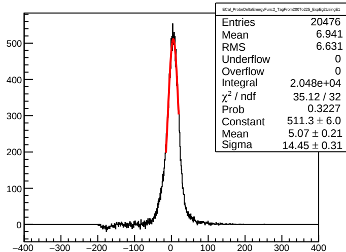
ECal_ProbeDeltaEnergyFunc2_TagFrom200To225_ExpEg2UsingE1
