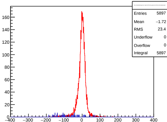
ECal_ProbeDeltaEnergyFunc2_TagFrom270To315_tagOuterR_inFR106_258_ExpEg2UsingE1
