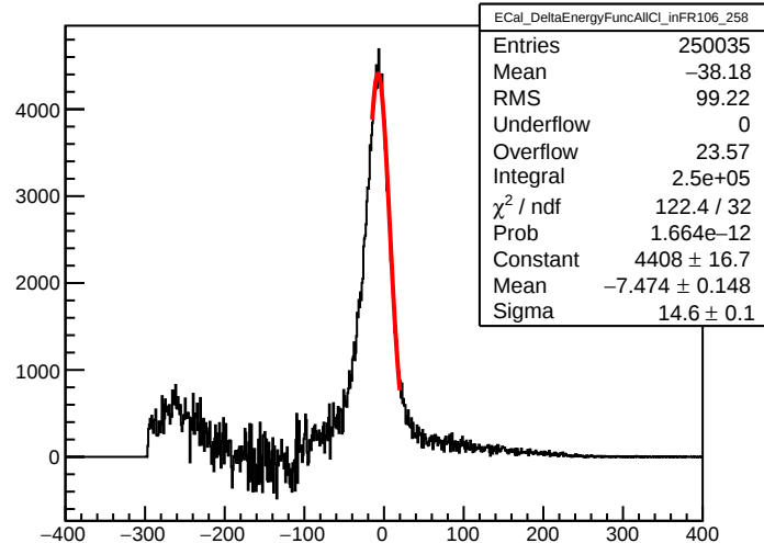
ECal_DeltaEnergyFuncAllCI_inFR106_258
