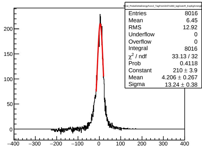
ECal_ProbeDeltaEnergyFunc2_TagFrom315To360_tagOuterR_ExpEg2UsingE1
