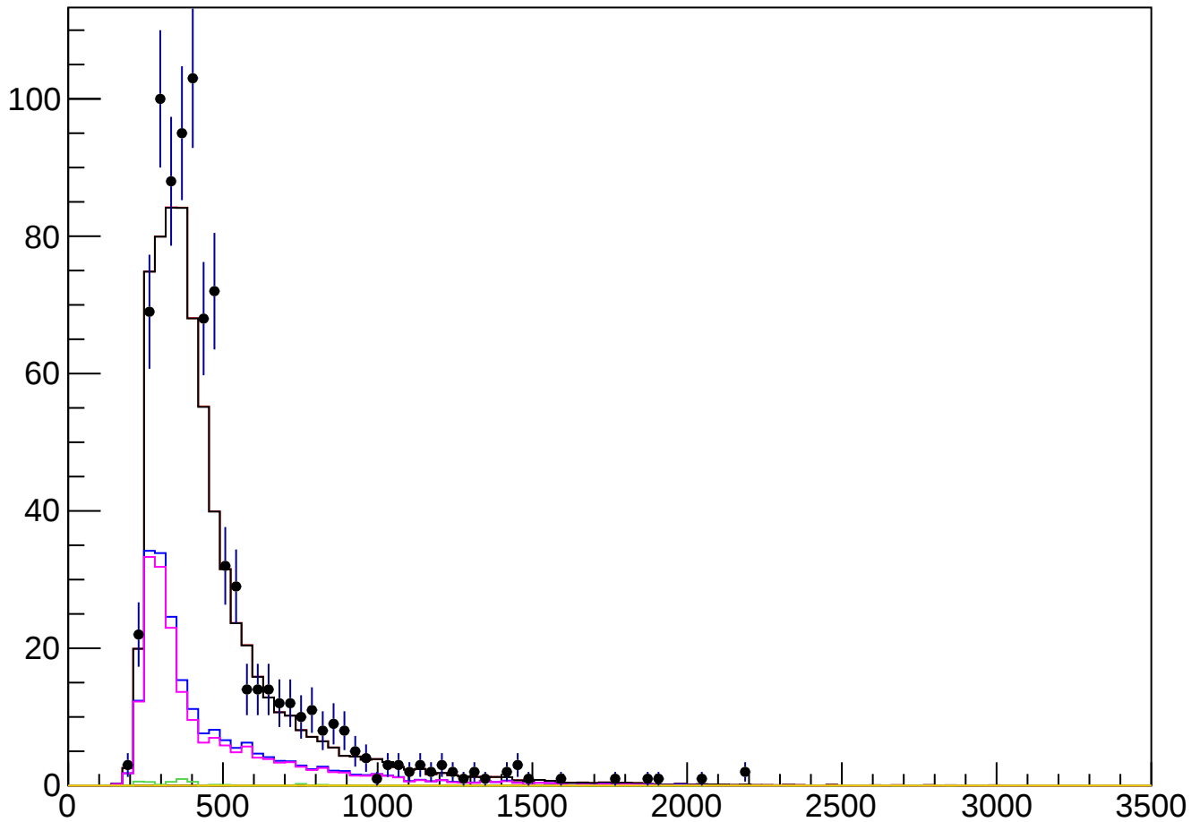
hSig_X_resolved_WZ_m
