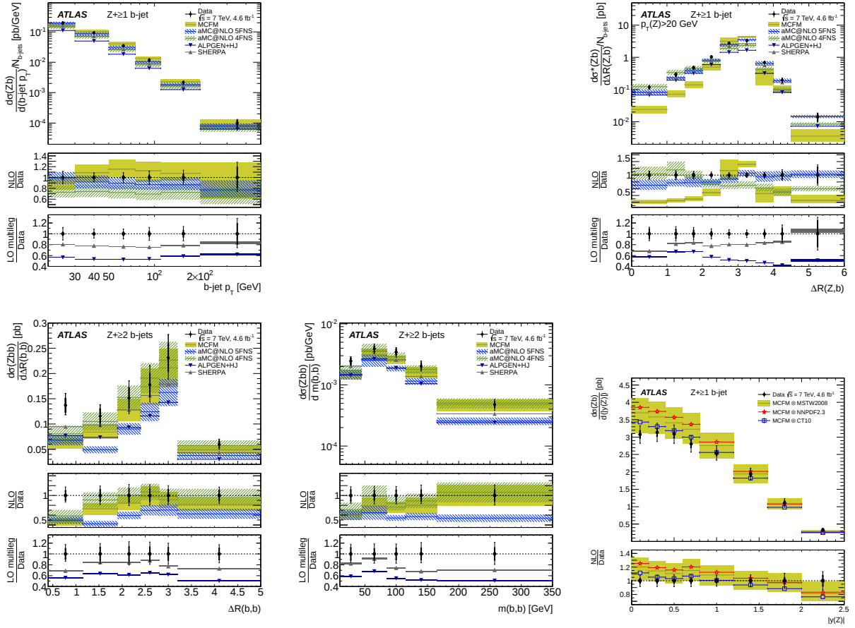
Figure 2. Differential cross sections for the Z+\geq 1b -jet (top); from left to right, the measured distributions of the following kinematic variables are shown: the b -jet transverse momentum, the absolute difference in rapidity and the distance \Delta R(Z, b - \text{jet}) = \sqrt{\Delta\phi^2 + \Delta y^2} between the Z boson the b -jet of highest p_T in the event. Differential cross sections for the Z+\geq 2b -jets (bottom, left and center) as a function of the separation between the two b -jets, \Delta R(b, b) , and of the invariant mass of the two b -jets. The bottom-right plot shows the rapidity distribution of the Z boson in the inclusive Z+\geq 1b -jet selection, superimposed with the predictions from MCFM interfaced to three different sets of NLO Parton Density Functions.
