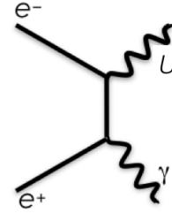
Figure 1. Feynman diagram for U boson (dark photon) production in annihilation of a positron with an electron of the target.
