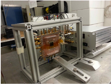
Figure 2. First full carbon PADME active target prototype realized in Lecce.
